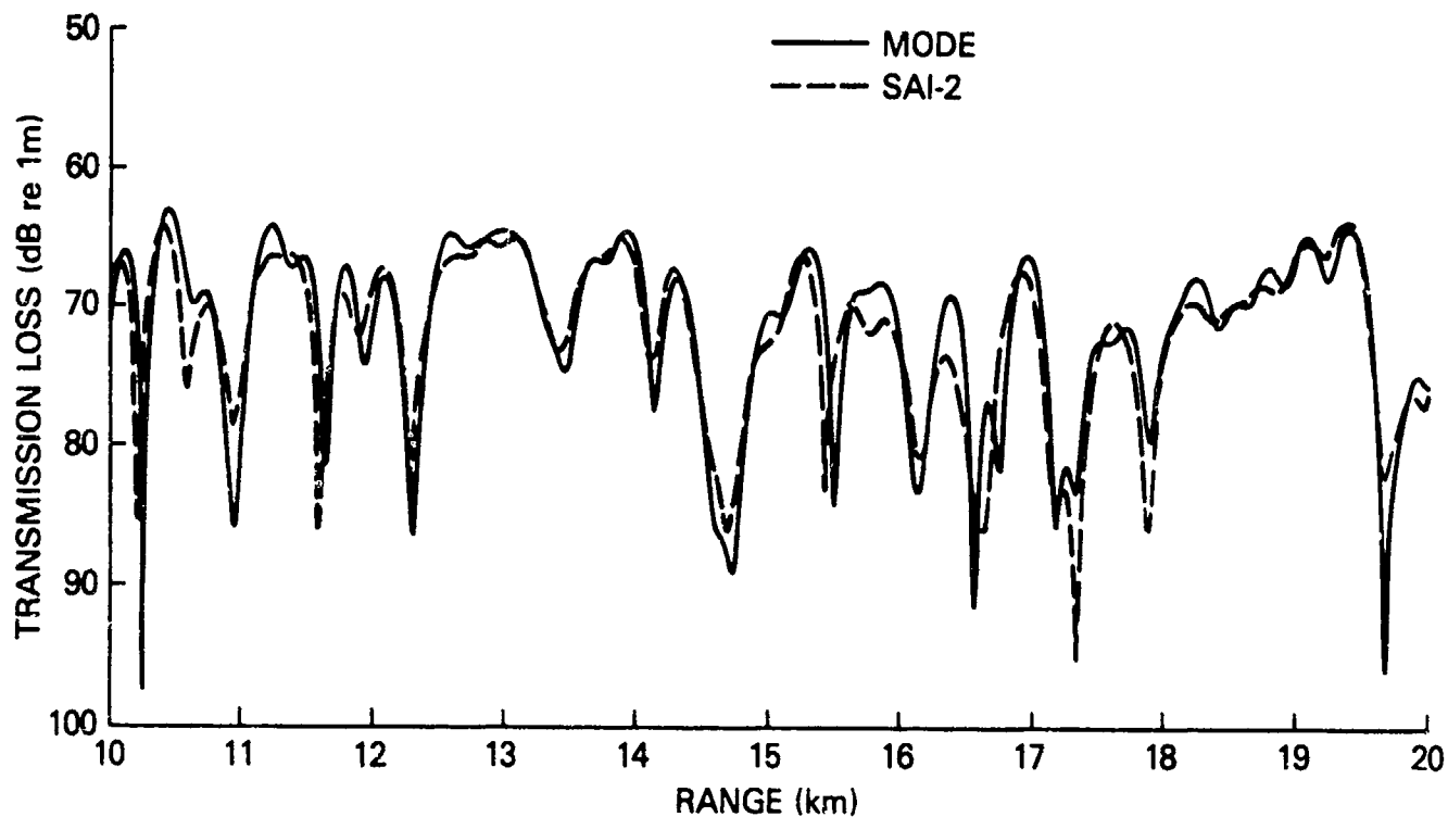
Figure 13. SAI-2 PE result compared with reference result (MODE) for Test Case 2C
