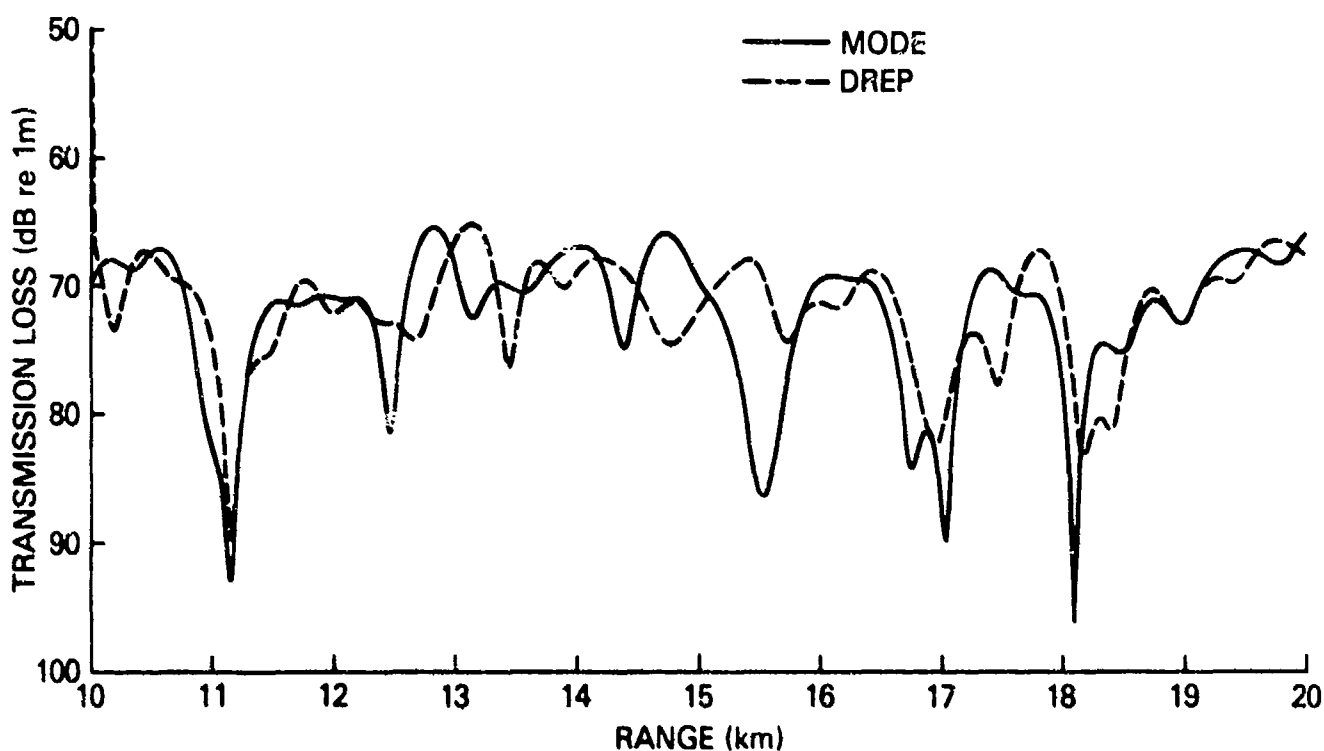
Figure 10. DREP PE result compared with reference result (MODE) for Test Case 2B
