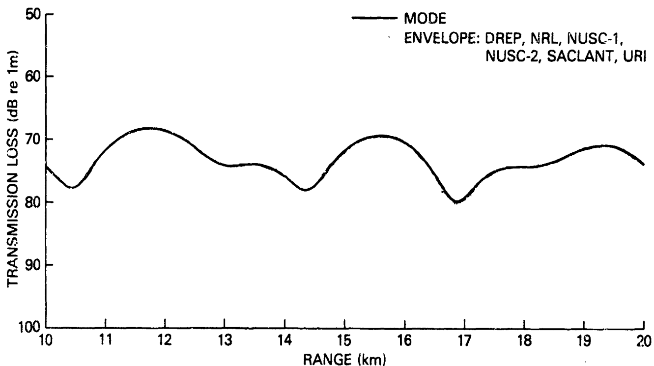
Figure 6. Envelope of various PE results compared with reference calculation (MODE) for Test Case 2A
