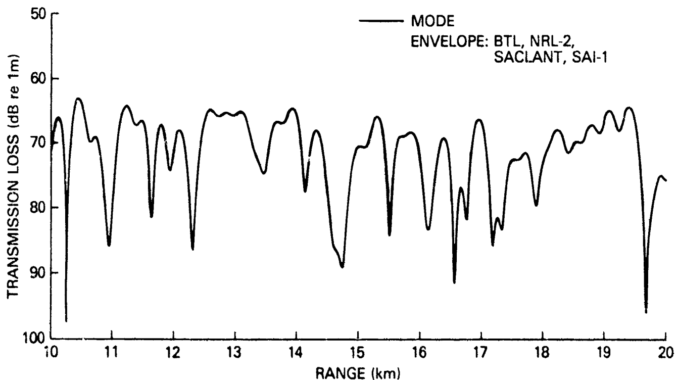
Figure 16. Envelope of results of PE programs that did use CMOD compared with reference result (MODE) for Test Case 2C
