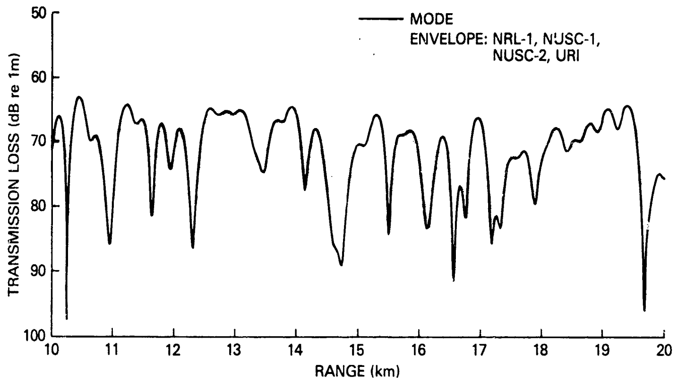
Figure 15. Envelope of results of PE programs that did not use CMOD compared with reference result (MODE) for Test Case 2C
