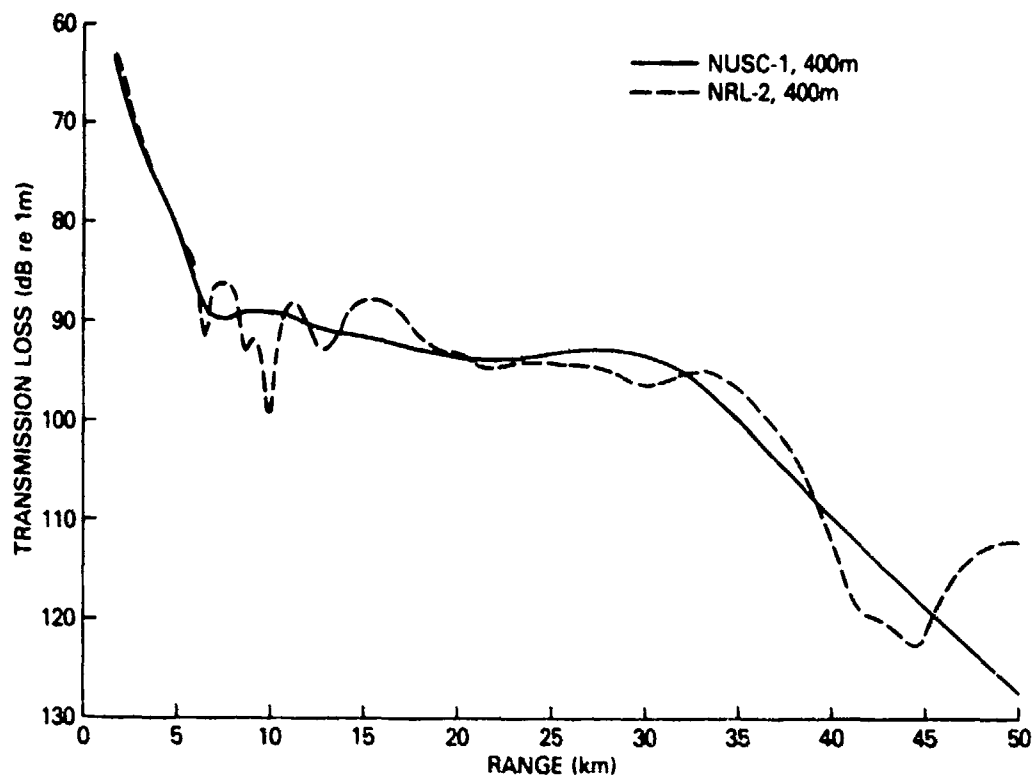
Figure 2. NRL-2 PE results for Test Case 1C compared with NUSC-1 PE
