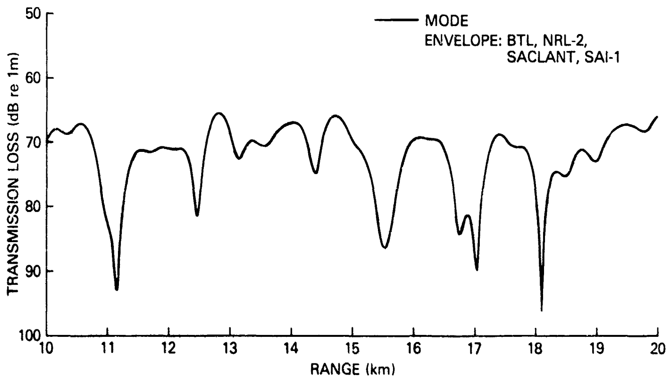
Figure 12. Envelope of results of PE programs that did use CMOD compared with reference result (MODE) for Test Case 2B
