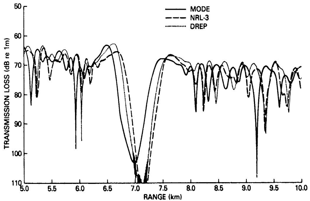
Figure 27. NRL-3 and DREP PE results compared with reference result (MODE) for Test Case 3B
