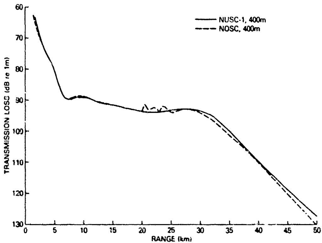
Figure 5. NOSC PE results for Test Case 1C compared with NUSC-1 PE
