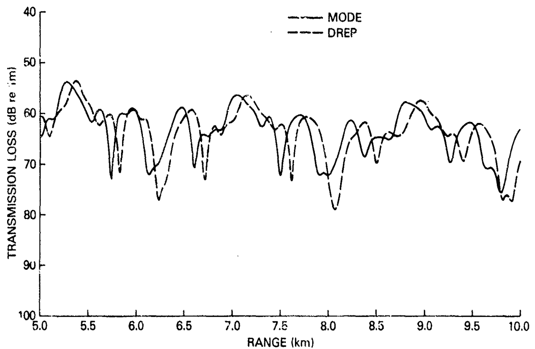
Figure 13. DREP PE result compared with reference result (MODE) for Test Case 3A
