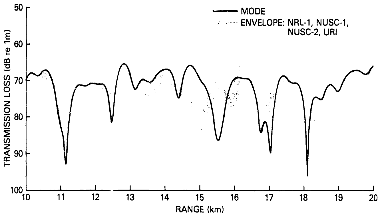
Figure 11. Envelope of results of PE programs that did not use CMOD compared with reference result (MODE) for Test Case 2B
