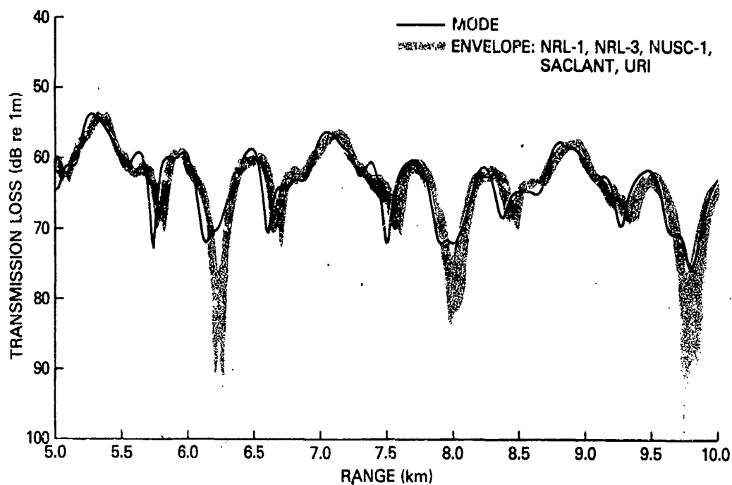
Figure 19. Envelope of the results of a group of PE programs compared with reference result (MODE) for Test Case 3A
