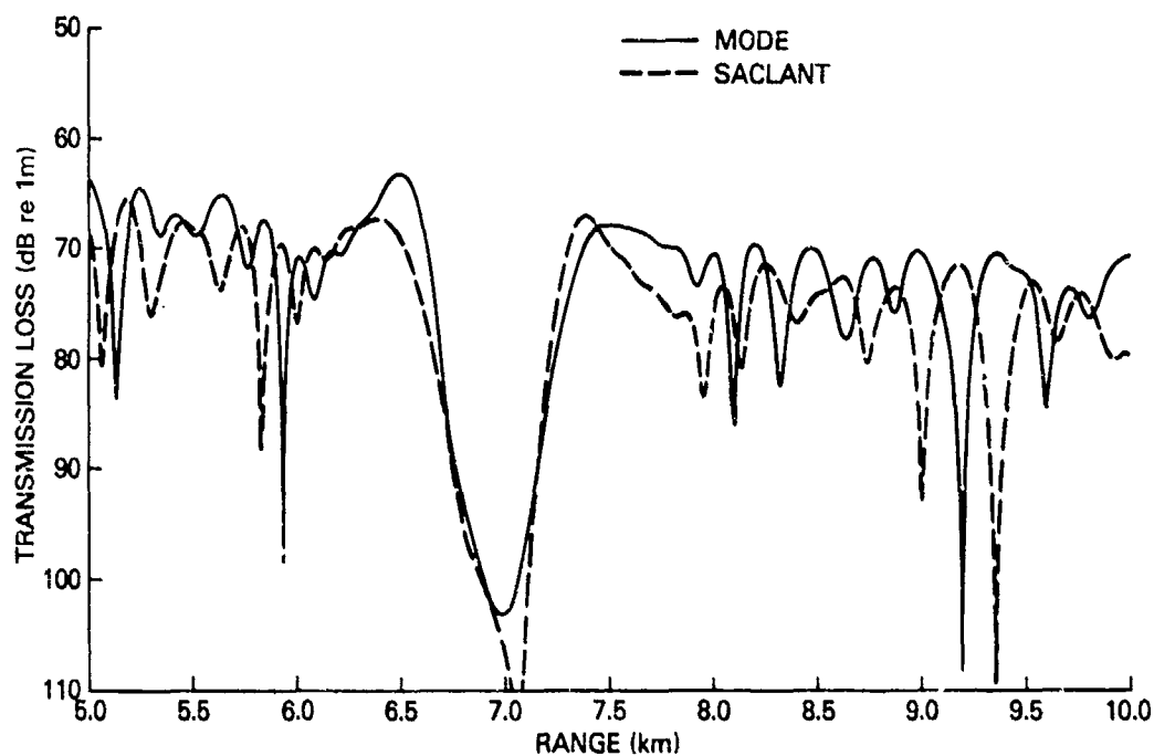
Figure 25. SACLANT PE result compared with reference result (MODE) for Test Case 3B
