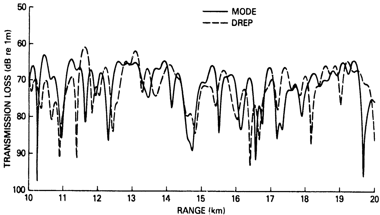
Figure 14. DREP PE result compared with reference result (MODE) for Test Case 2C
