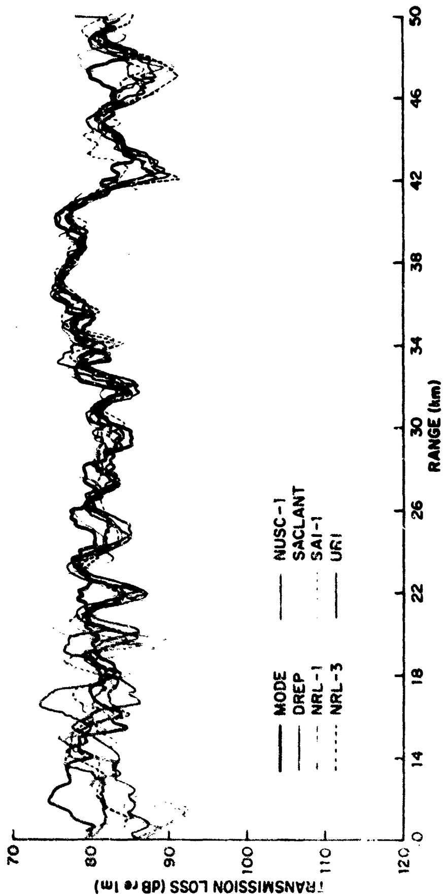
Figure 29. PE program results (1 km intensity average) compared with reference result (MODE) for basin of Test Case 4A
