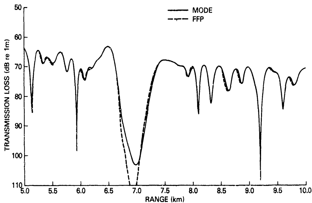
Figure 22. Comparison of MODE (SNAP) and FFP results for Test Case 3B
