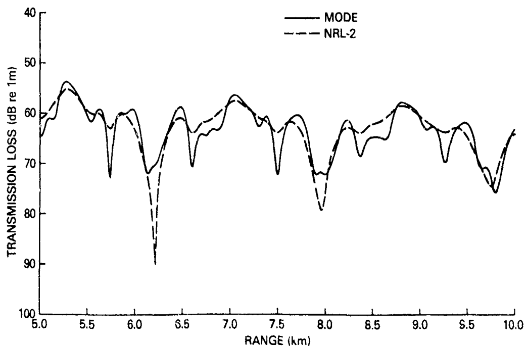
Figure 20. NRL-2 PE result compared with reference result (MODE) for Test Case 3A
