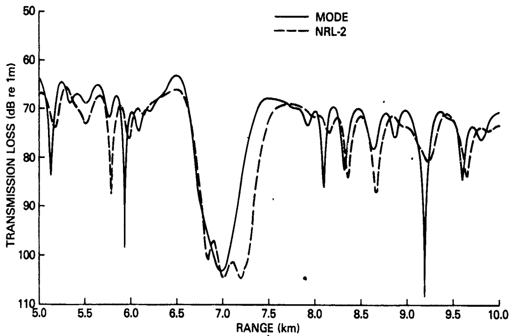
Figure 26. NRL-2 PE result compared with reference result (MODE) for Test Case 3B
