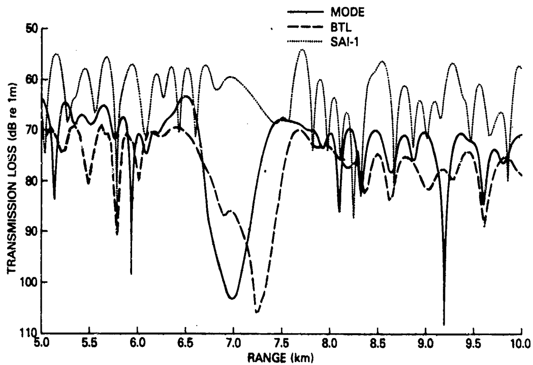
Figure 28. BTL and SAI-1 PE results compared with reference result (MODE) for Test Case 3B
