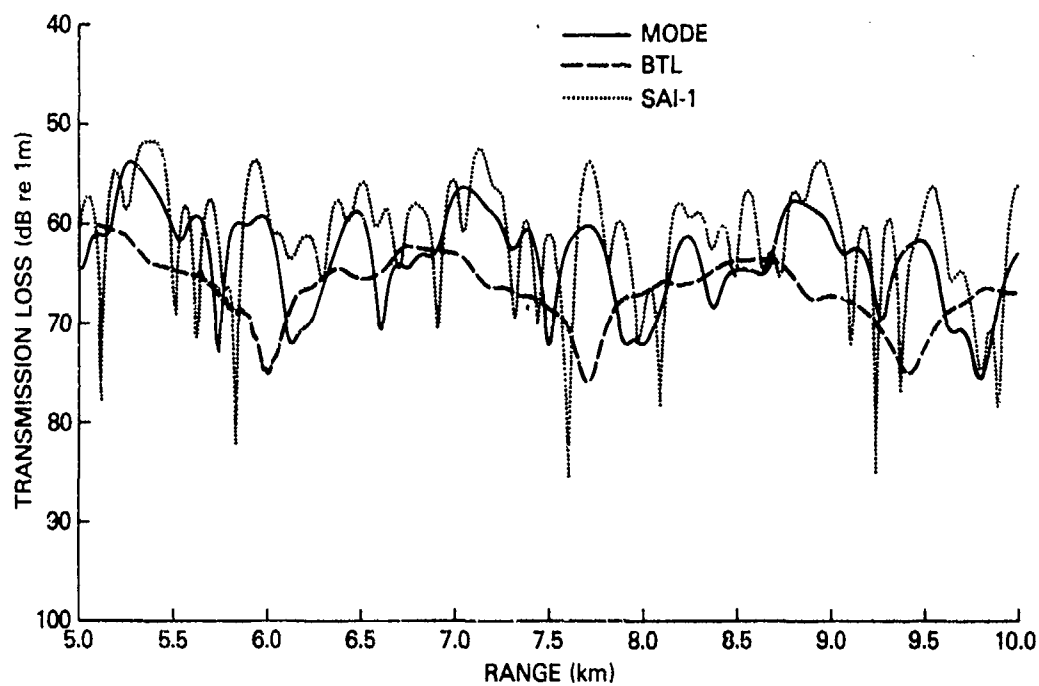
Figure 21. BTL and SAI-1 PE results compared with reference result (MODE) for Test Case 3A
