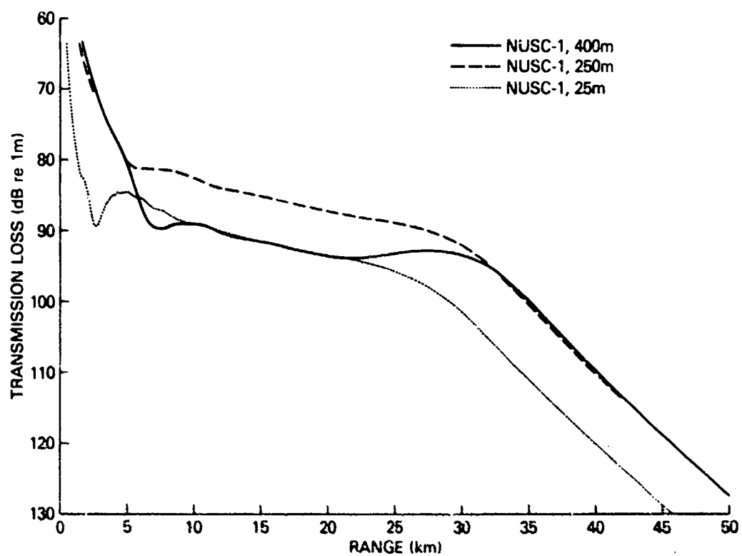
Figure 1. NUSC-1 PE results for Test Case 1
