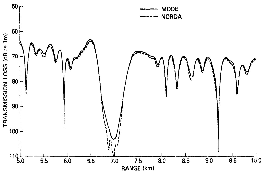
Figure 23. NORDA PE result compared with reference result (MODE) for Test Case 3B
