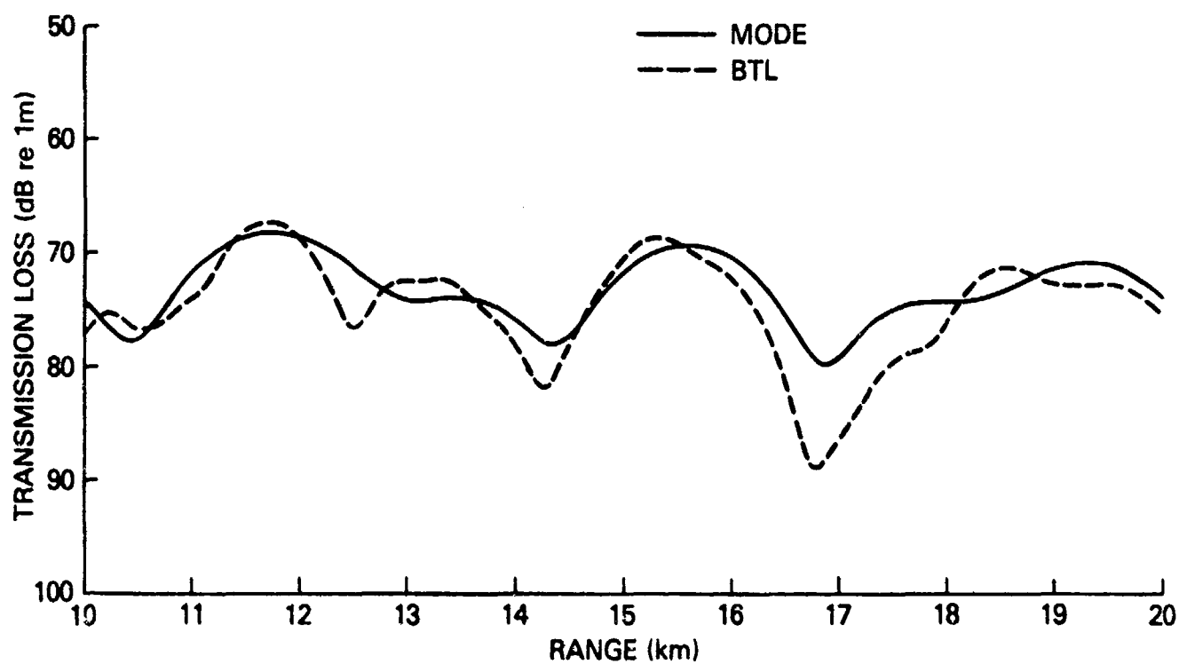
Figure 8. BTL PE result compared with reference result (MODE) for Test Case 2A
