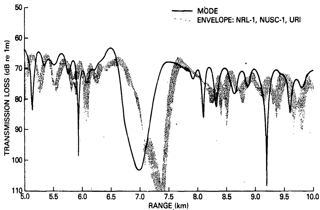
Figure 24. Envelope of NRL-1, NUSC-1, and URI PE results compared with reference result (MODE) for Test Case 3B
