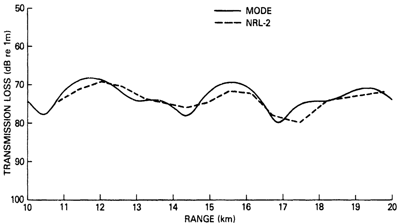
Figure 7. NRL-2 PE result compared with reference result (MODE) for Test Case 2A
