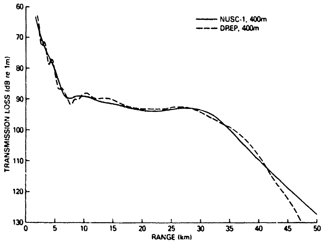
Figure 3. DREP PE result for Test Case 1C compared with NUSC-1 PE
