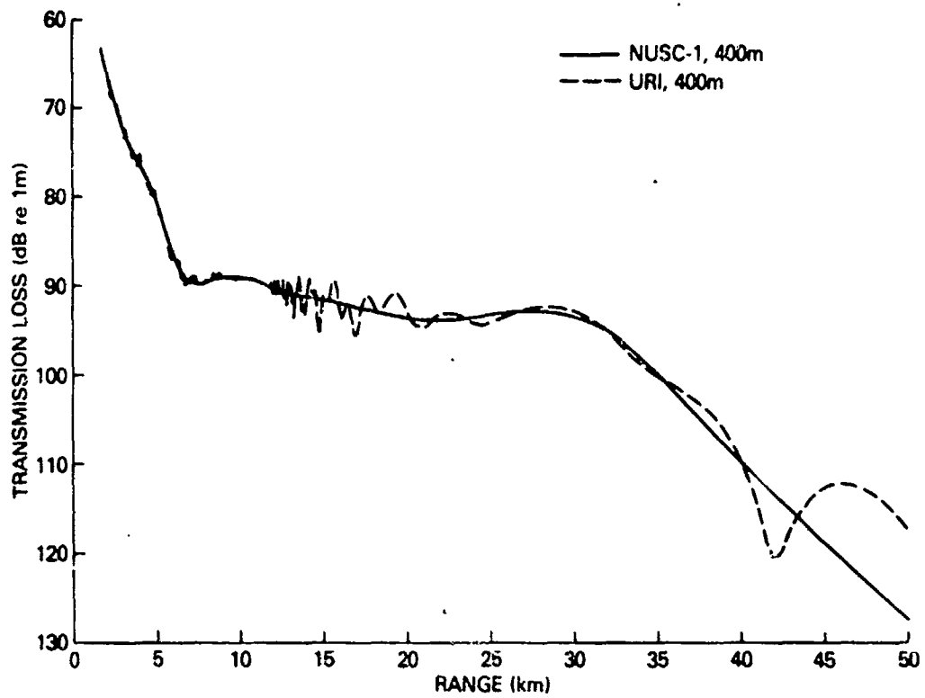
Figure 4. URI PE results for Test Case 1C compared with NUSC-1 PE
