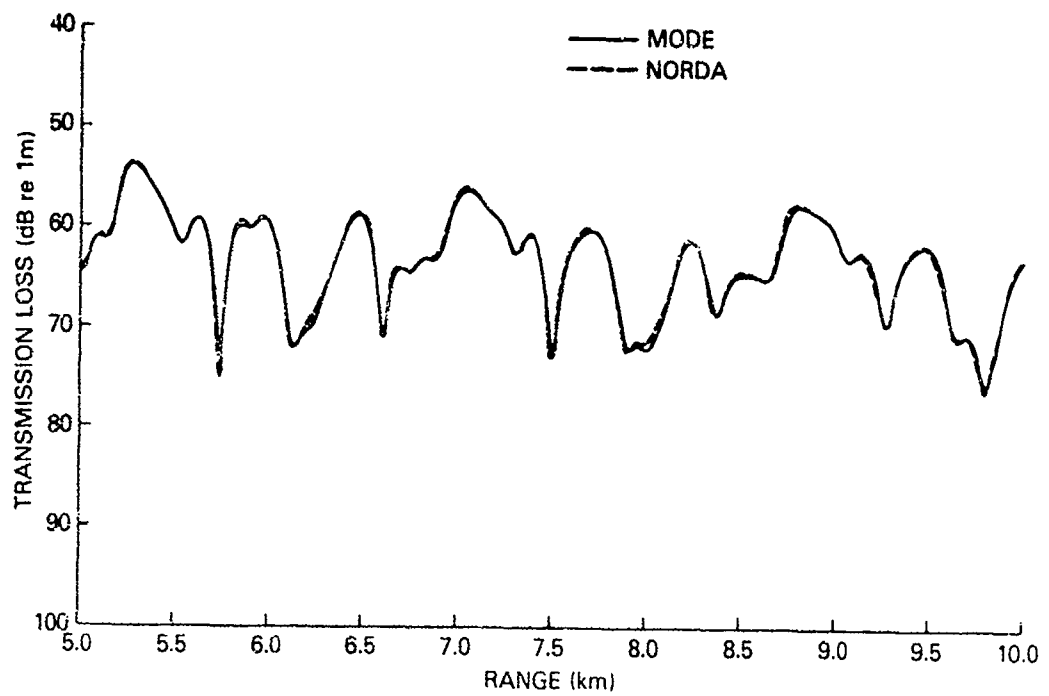
Figure 17. NORDA PE result compared with reference result (MODE) for Test Case 3A
