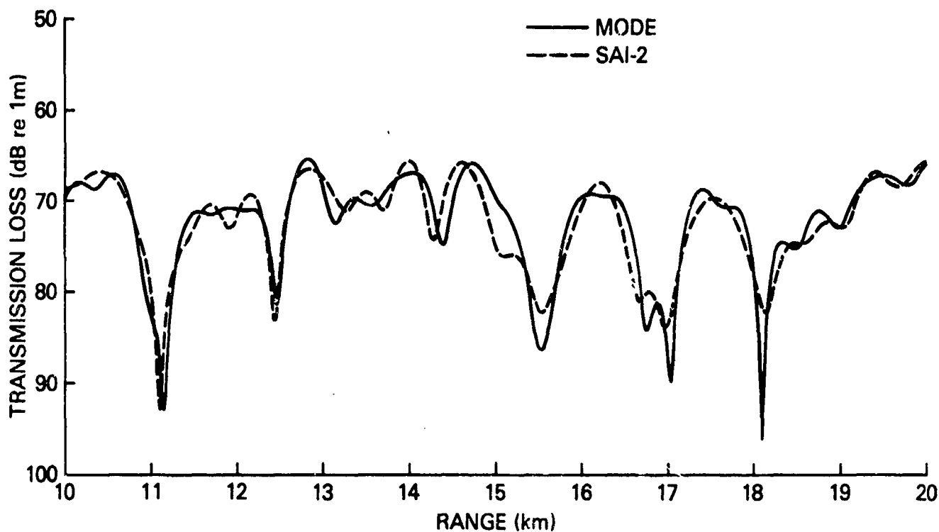
Figure 9. SAI-2 PE result compared with reference result (MODE) for Test Case 2B
