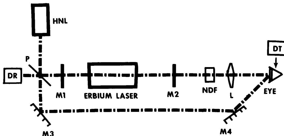
Figure 1. Erbium laser exposure system with emission wavelength of 1.732 \mu\text{m} . DR - Reference detector, DT - Target detector, HNL - Helium neon alignment laser, NDF - Neutral density filter holder, M1 to M4 - mirrors, P - pellicle, L - lens.
