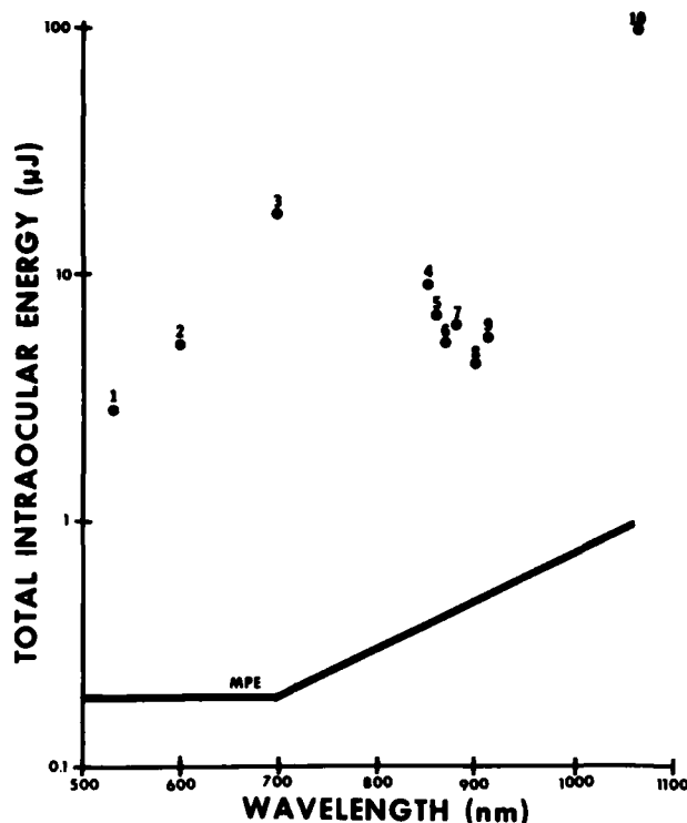
Figure 9. Wavelength dependence of the MPE and the ED 50 for retinal damage in the rhesus monkey.
