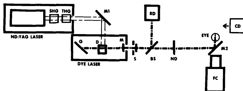
Figure 3. Exposure configuration.
