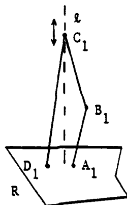
Figure 2.3.3 Keeping links nearly "vertical". (The slot along l and the two link connection between A_1 and D_1 are not shown.)
