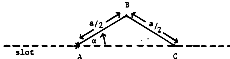
Figure 2.4.1 Representing z by angle \alpha
