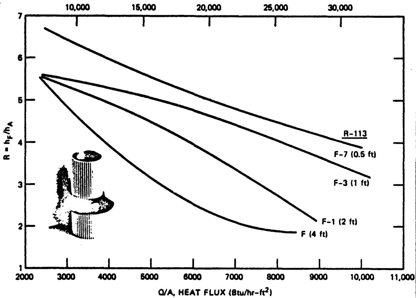
Figure 19. Enhancement ratio for a vertical fluted tube, and the effects of drain-off skirts [from Ref. 82].
