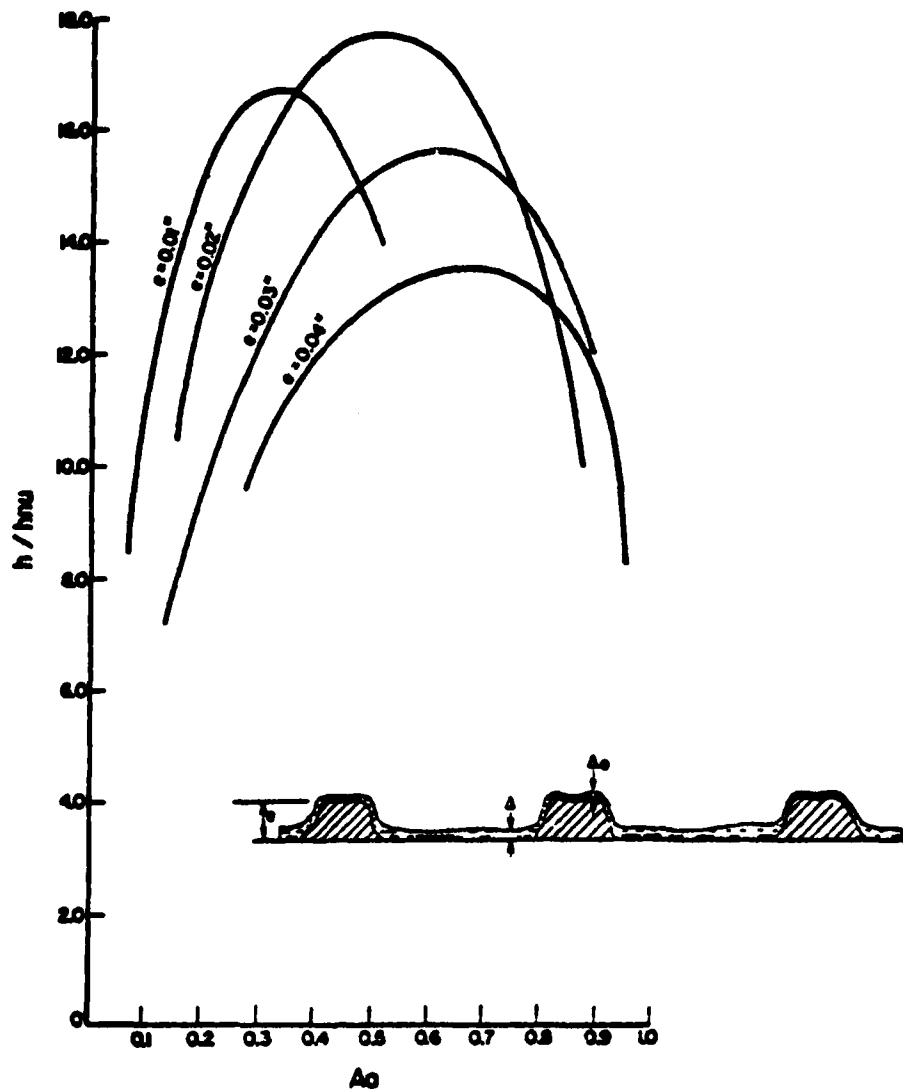
Figure 20. The influence of randomly distributed metal particles on film condensation on a vertical tube [from Ref.85 ].
