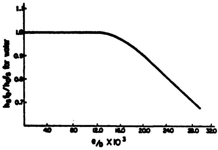
Figure 1. Performance characteristics of three-dimensional roughness [from Ref. 9]
