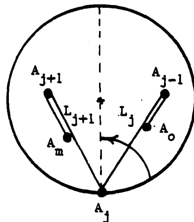
Configuration 2: L_{j+1} lies off the diagonal
