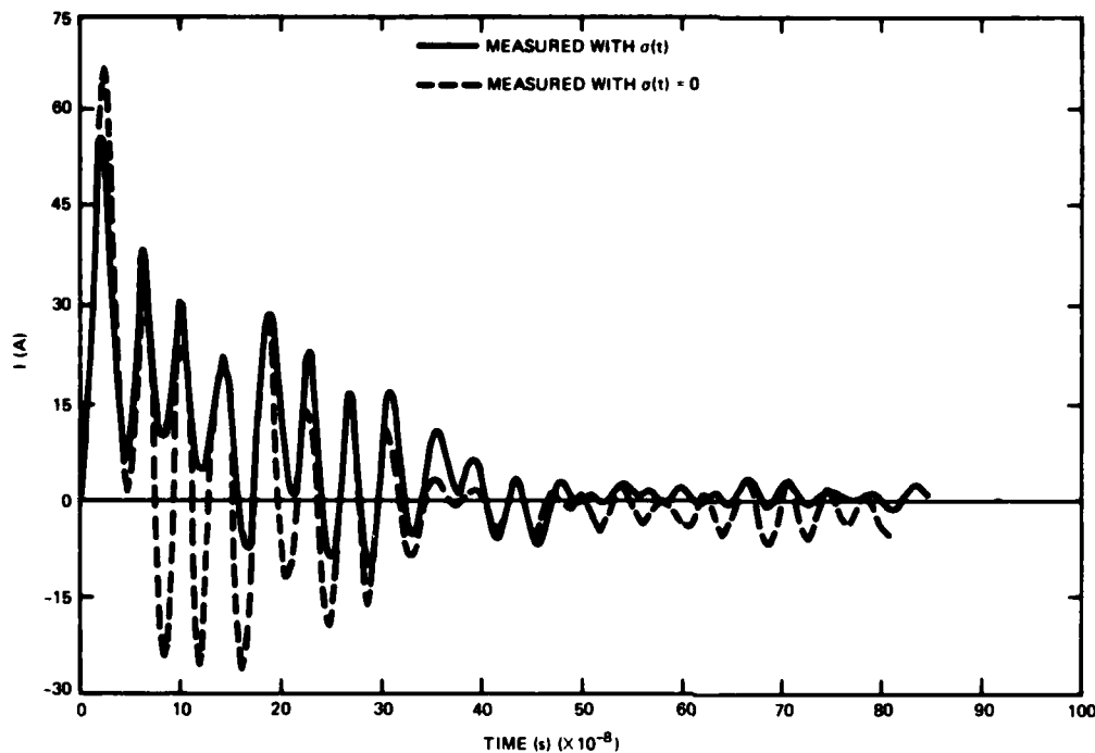
Figure 24. Comparison of measured short-circuit current monopole antenna response (2.42 m) with and without ambient time-varying ionized air conductivity (time in s \times 10^{-8} ).
