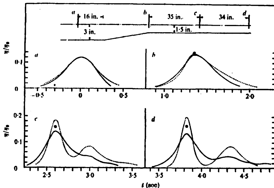
Figure 83. Comparisons of Boussinesq theory and experiments for wave shoaling (after Madsen and Mei, 1969). 49
