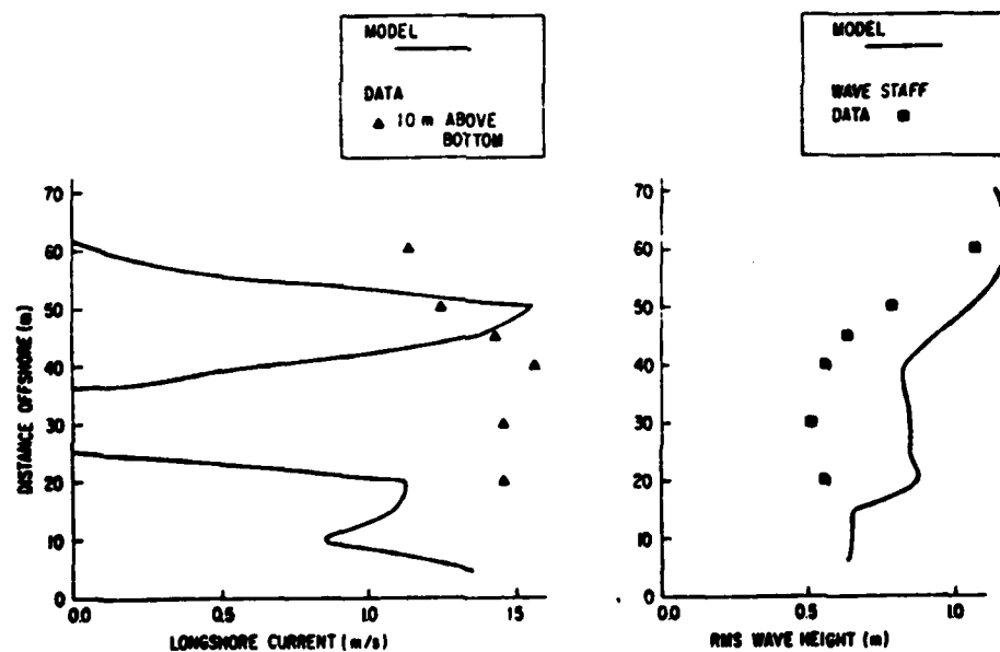
(d) Sharply peaked model current profiles (a) result from underestimation of wave height decay (b) across the surf zone.
