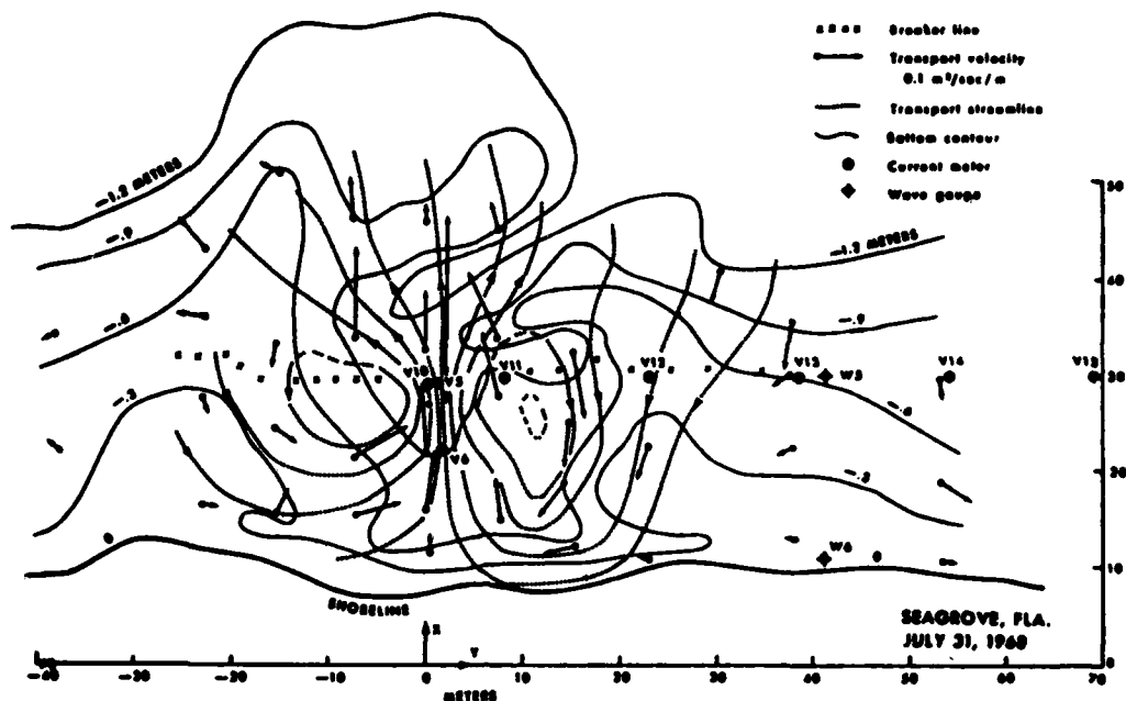
Distribution of transport velocities and streamlines in the circulation cell. Streamline separation is 0.4 \text{ m}^2/\text{sec} , H_0 = 0.395 \text{ meter} , T_0 = 5.0 \text{ sec} , and \alpha_0 = 0 .
