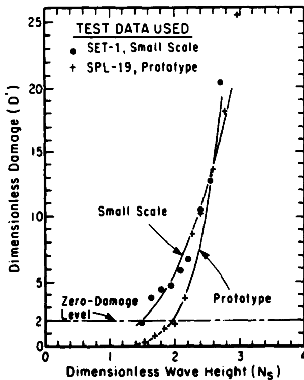
Figure 5. Typical small-scale and prototype damage trends for d/gT^2 = 0.0144 .
