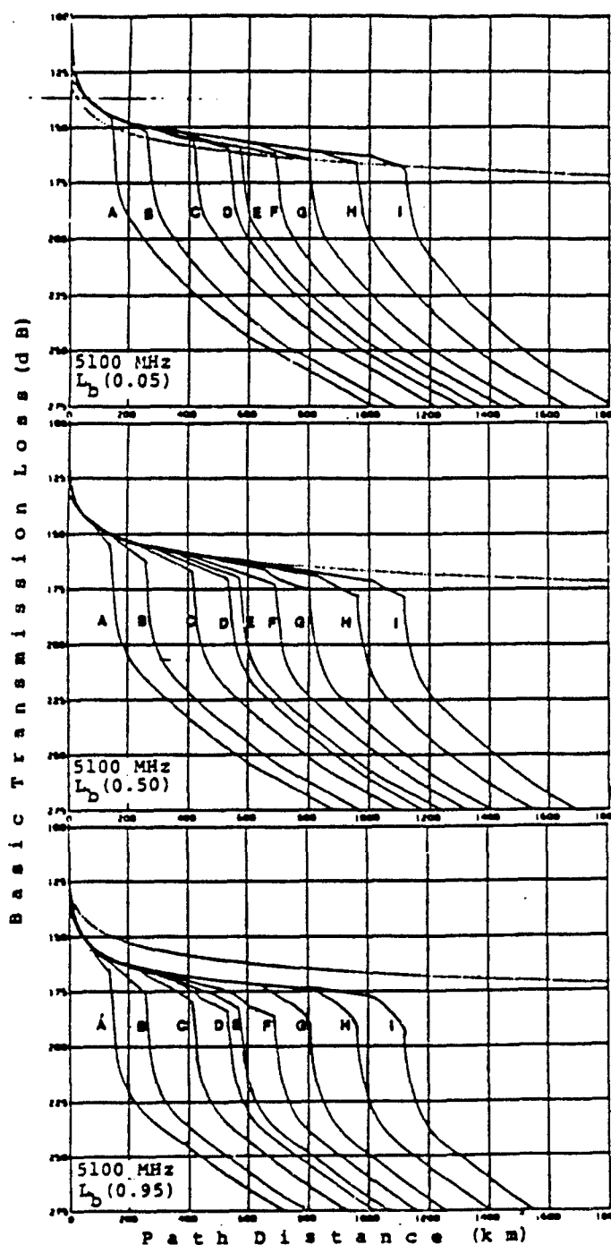
Figure 8-4. Basic transmission loss, 5100 MHz.
