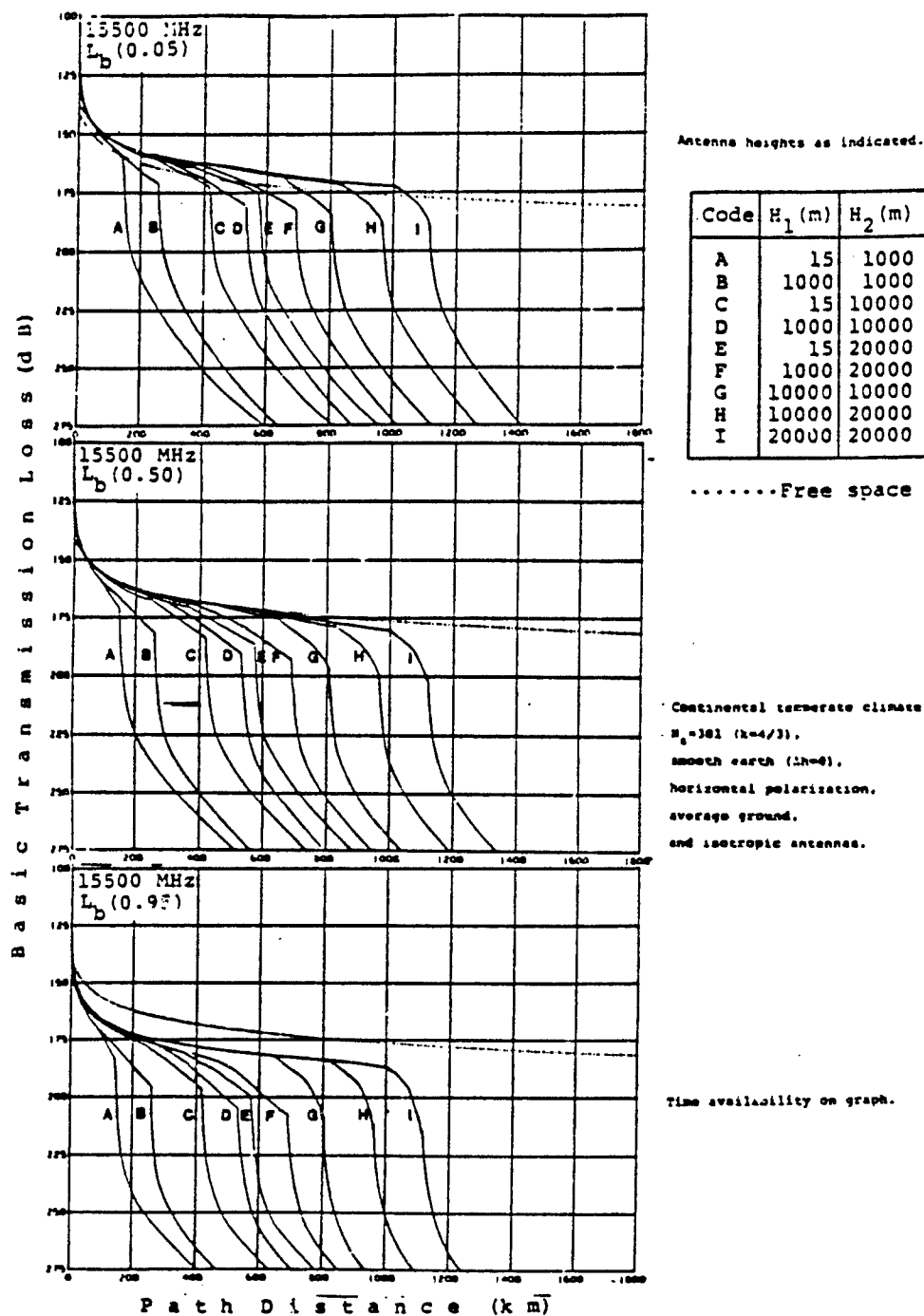
Figure 8-6. Basic transmission loss, 15,500 MHz.
