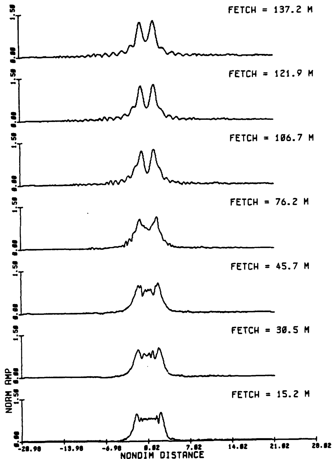
Fig. 3.26b Amplitude modulations from the inviscid NLS solution, at times corresponding to the fetches in (a), for the evolution of a group of 25 waves, initial steepness ak = .07 (Exp 77).
