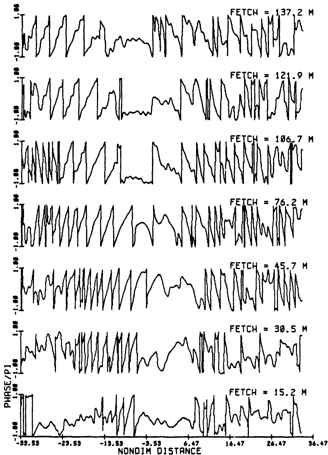
Fig. 3.47a Phase modulations from observations, principal value and normalized by \pi , for successive fetches for the evolution of a group of 15 waves, initial steepness ak = .16 (Exp 22).
