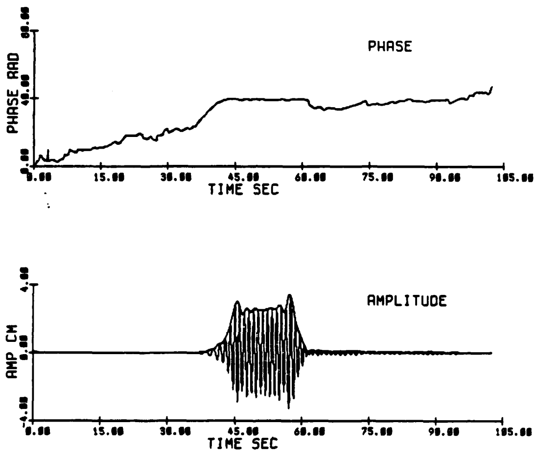
Fig 3.30 Initial condition at 6.1 m (E87) ak = .10, N = 15
