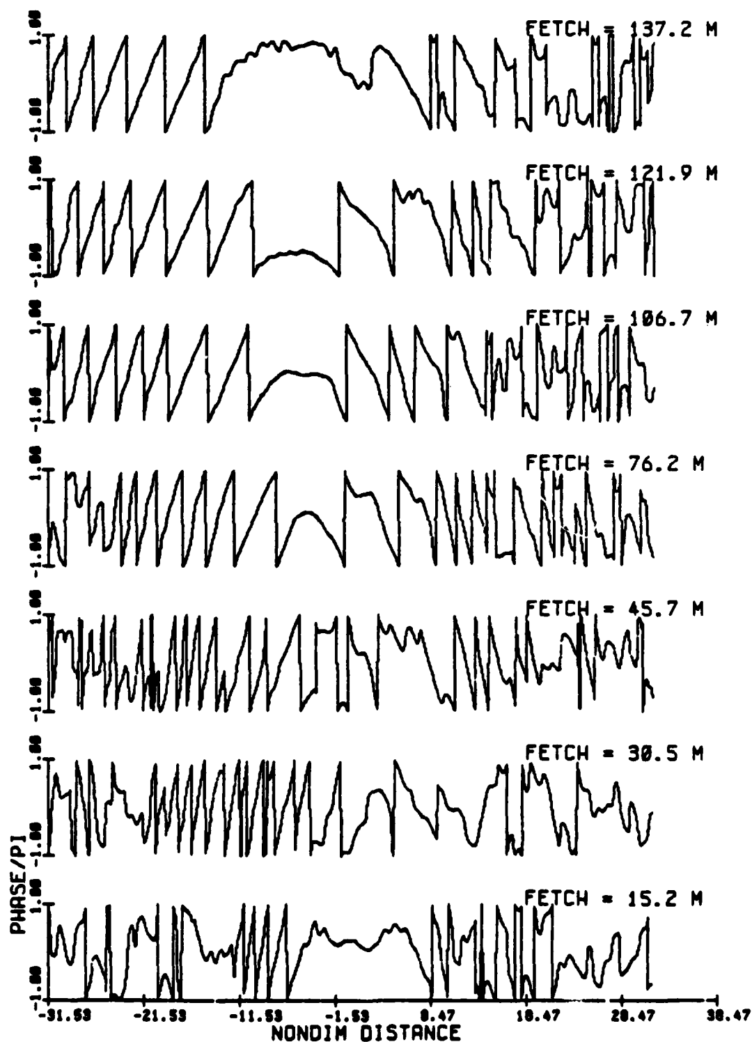
Fig. 3.42a Phase modulations from observations, principal value and normalized by \pi , for successive fetches for the evolution of a group of 15 waves, initial steepness ak = .15 (Exp 62).
