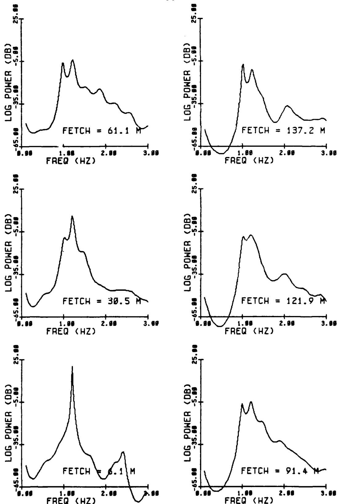
Fig. 2.18 Same as previous (2.17) except data is unfiltered and spectrum is done on larger interval (.1,3.0)hz. Notice the first harmonic peak (6.1 m), the loss in resolution of sidebands (30.5 m) and the removal of spurious peaks at the bandedges of the filter.
