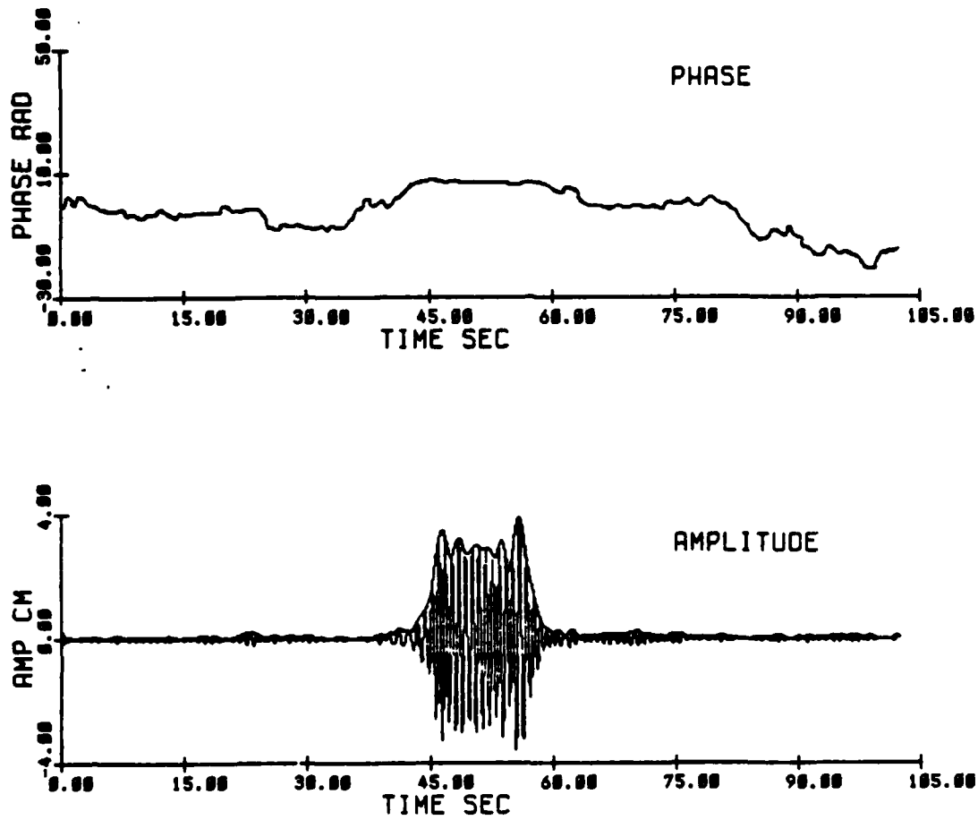
Fig 3.45 Initial condition at 6.1 m (E22) ak = .16, N = 15
