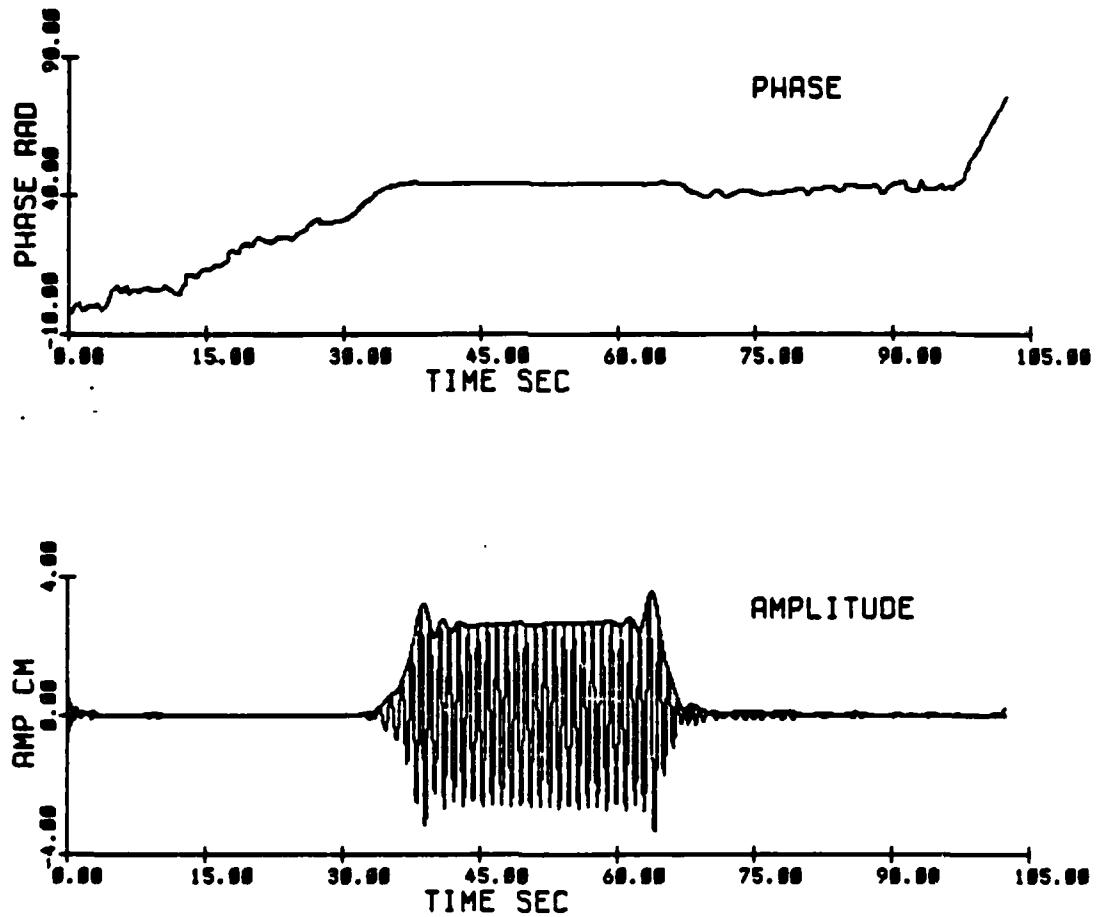
Fig 3.35 Initial condition at 6.1 m (E88) ak = .10, N = 25
