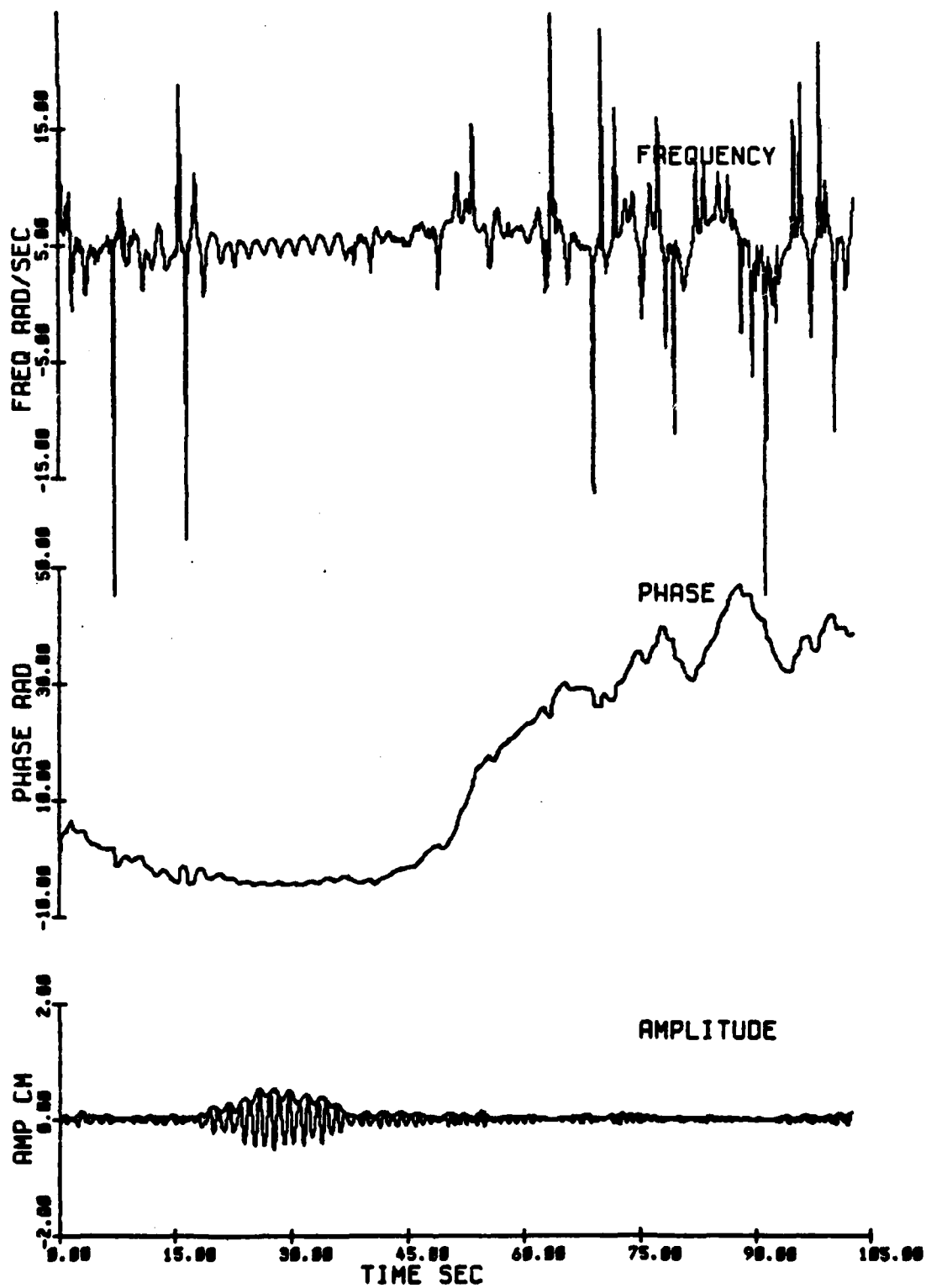
Fig. 2.28 Amplitude, phase and frequency modulations at 106.7 m for a group of 10 waves of initial steepness ak = .03 (Exp 78).
