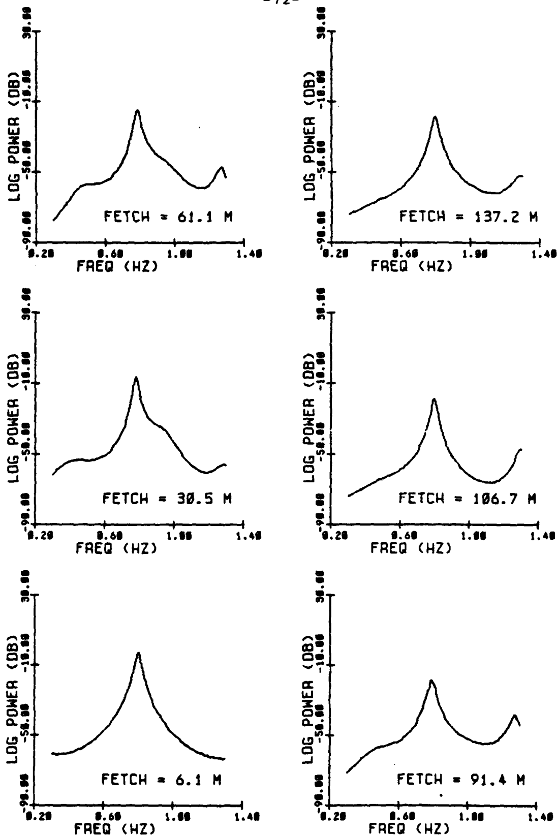
Fig. 2.12 Maximum entropy (MEM) spectral evolution with fetch for a group of 10 waves of steepness ak = .03 (Exp 78). Fetches as indicated. Group was bandpassed on the interval [.3, 1.3] Hz centered on the initial carrier frequency 0.80 Hz. Filter rolloff occurs at the bandedges.
