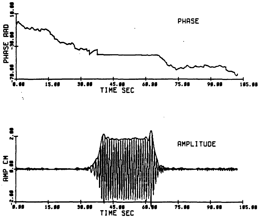
Fig 3.25 Initial condition at 6.1 m (E77) ak = .07, N = 25
