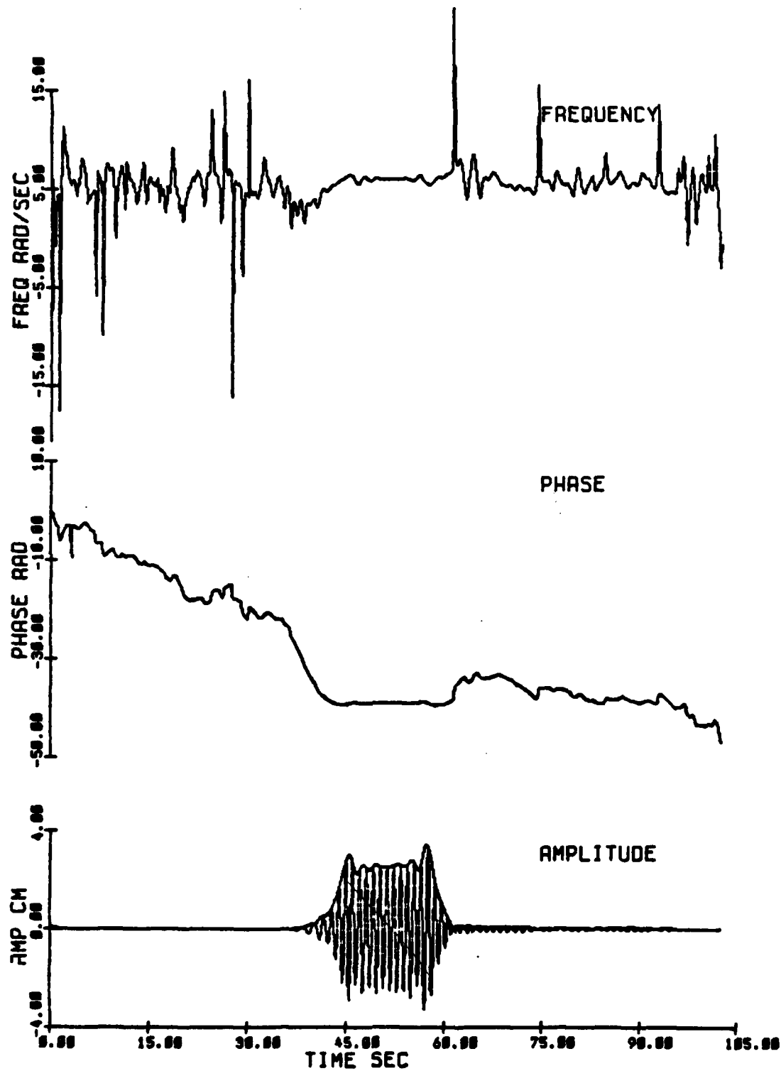
Fig. 2.30 Amplitude, phase and frequency modulations at 6.1 m for a group of 15 waves of initial steepness ak = .10 (Exp 97).
