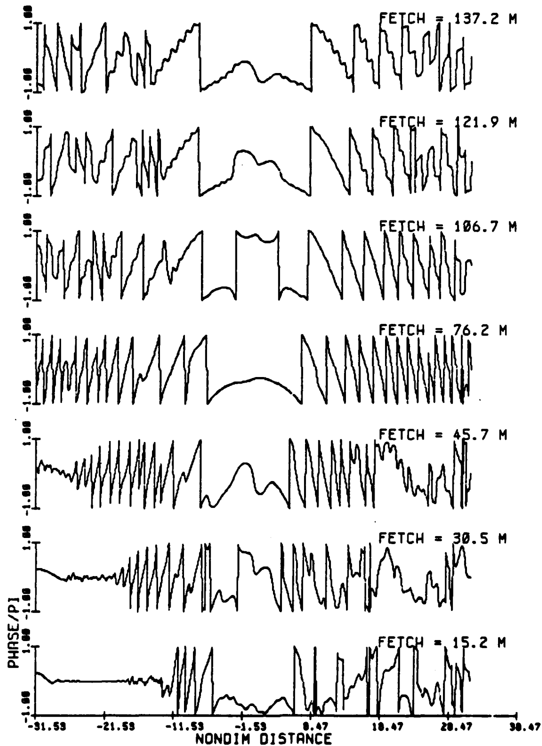
Fig. 3.42b Phase modulations from the inviscid NLS solution, at times corresponding to the fetches in (a), for the evolution of a group of 15 waves, initial steepness sk = .15 (Exp 62).
