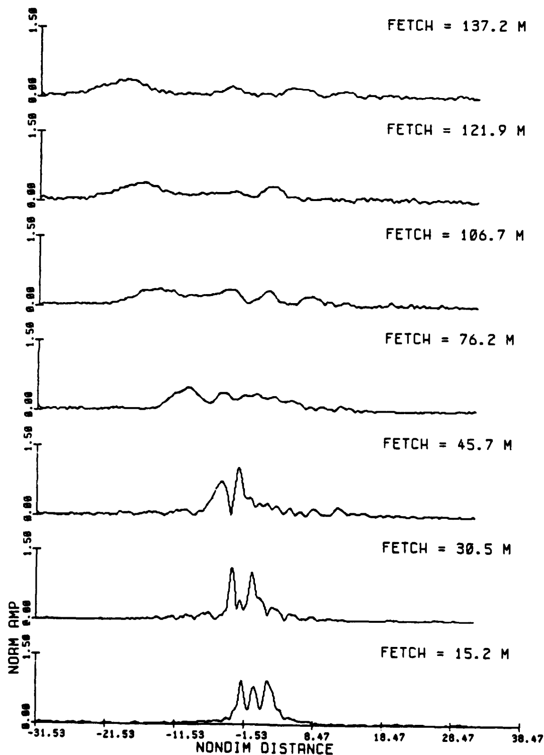
Fig. 3.41a Amplitude modulations from observations, nondimensionalized at each fetch by the initial condition scaling, for the evolution of a group of 15 waves, initial steepness ak = .15 (Exp 62).
