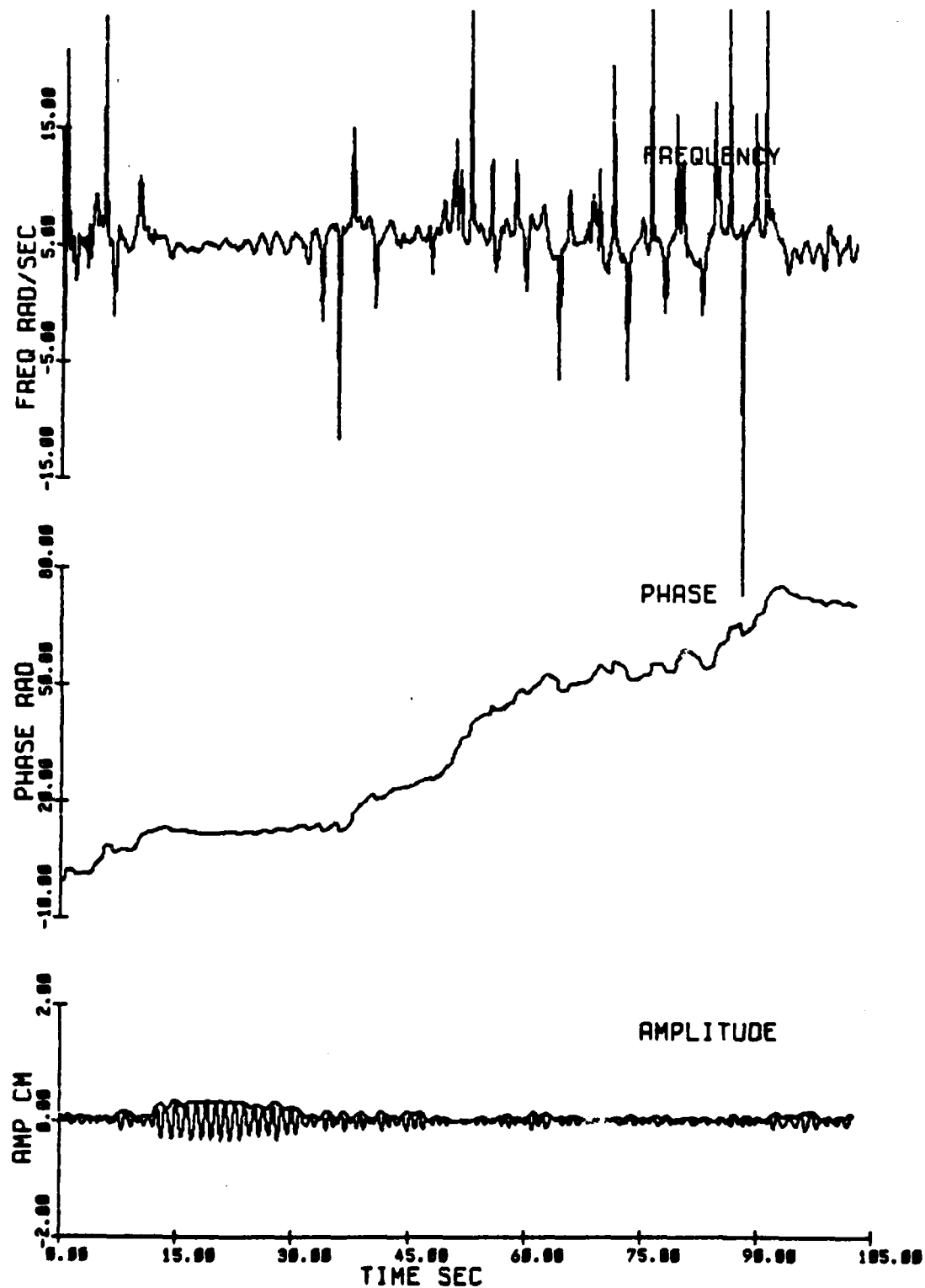
Fig. 2.29 Amplitude, phase and frequency modulations at 137.2 m for a group of 10 waves of initial steepness ak = .03 (Exp 7B).
