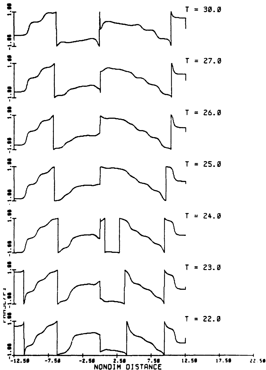
Fig. 3.16d Further evolution of the principal value of the wave modulation, normalized by p_1 , at 7 successive time steps, corresponding to the amplitude modulation of Fig. 3.16b
