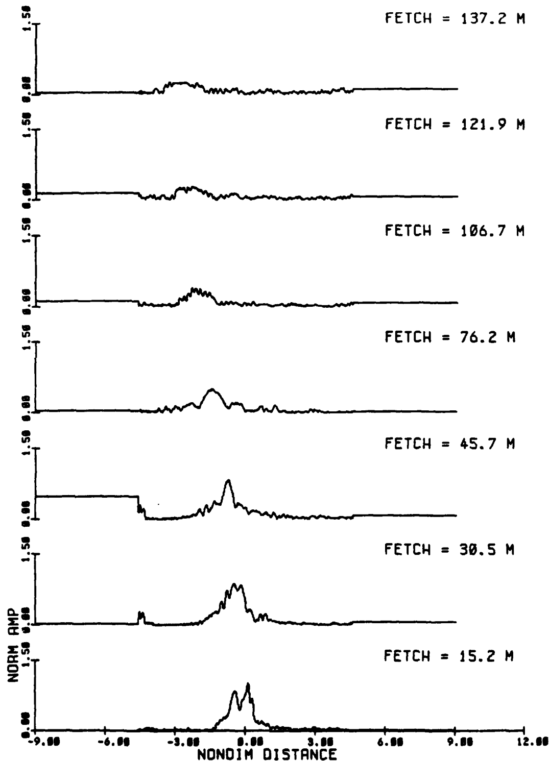
Fig. 3.21a Amplitude modulations from observations, nondimensionalized at each fetch by the initial condition scaling, for the evolution of a group of 10 waves, initial steepness ak = .03 (Exp 78).
