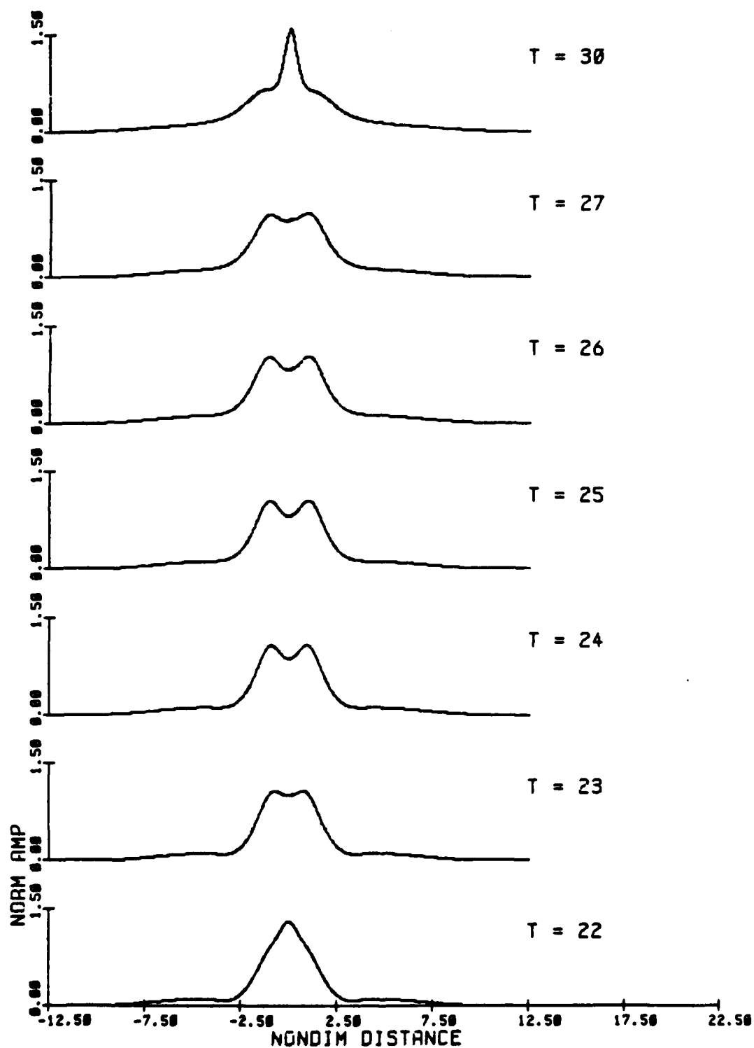
Fig. 3.13c Further evolution of the magnitude of the complex envelope plotted at 7 successive time steps (time increases upwards) for the 5/2-soliton initial condition.
