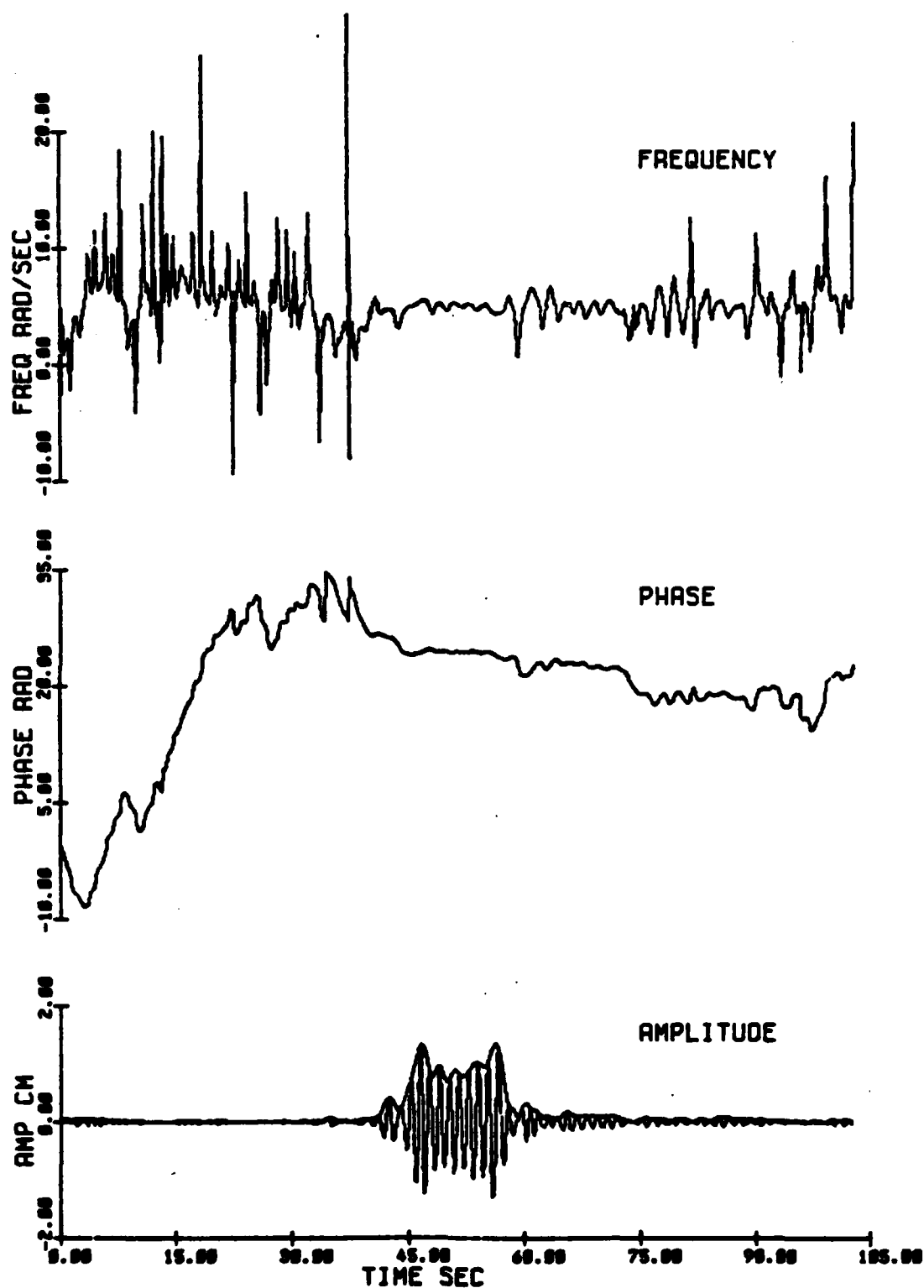
Fig. 2.24 Amplitude, phase and frequency modulations at 6.1 m for a group of 10 waves of initial steepness ak = .03 (Exp 78).
