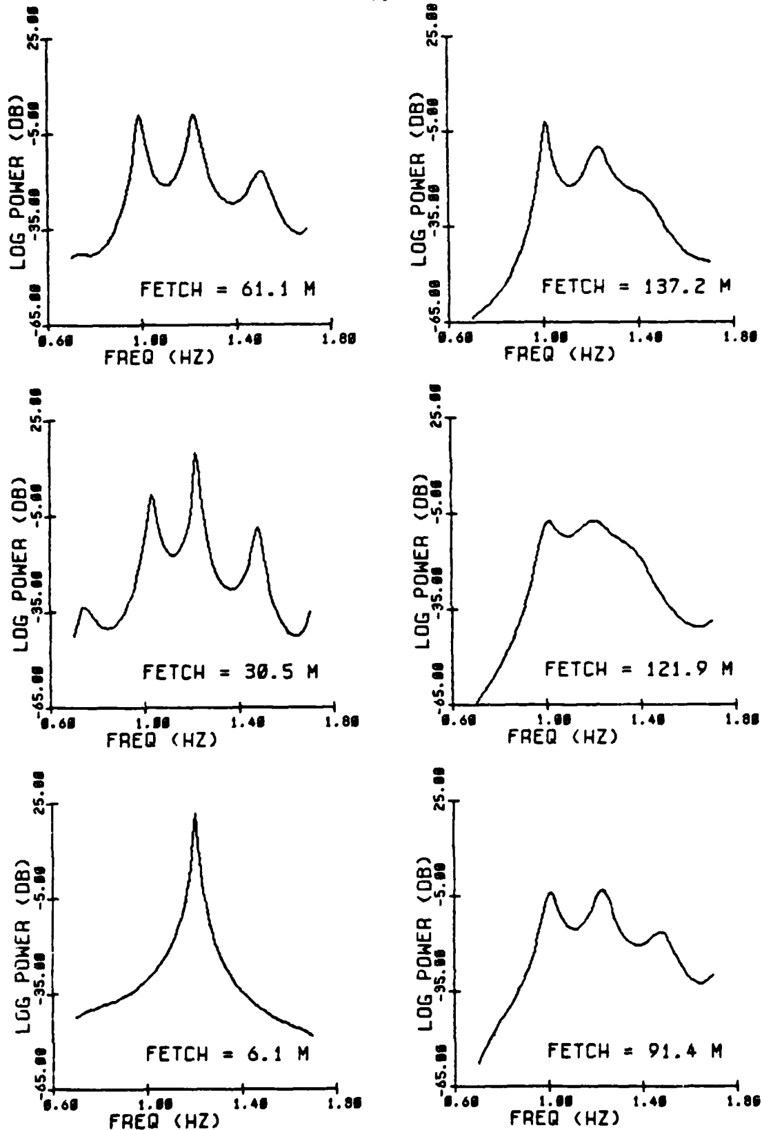
Fig. 2.17 Maximum entropy (MEM) spectral evolution with fetch for a group of 25 waves of steepness ak = .16 (Exp 23). Fetches as indicated. Group was bandpassed on the interval [0.7, 1.7] Hz centered on the initial carrier frequency 1.20 Hz. Filter rolloff occurs at the bandedges.
