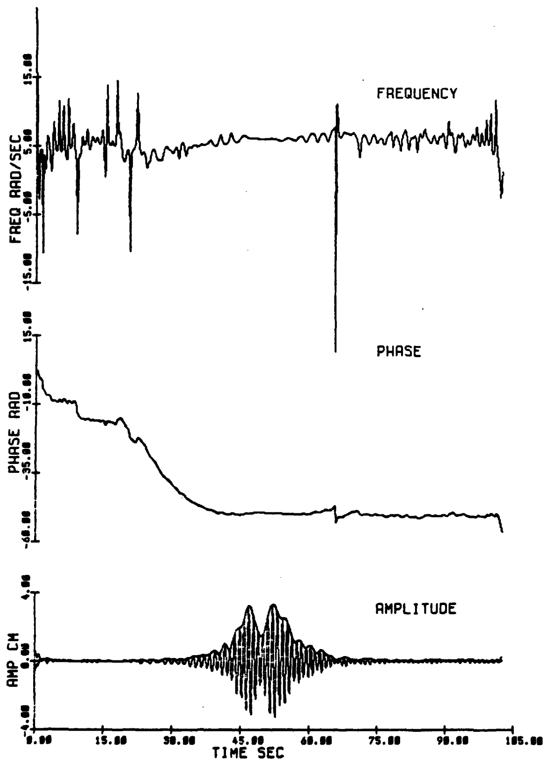
Fig. 2.31 Amplitude, phase and frequency modulations at 30.5 m for a group of 15 waves of initial steepness ak = .10 (Exp 87).
