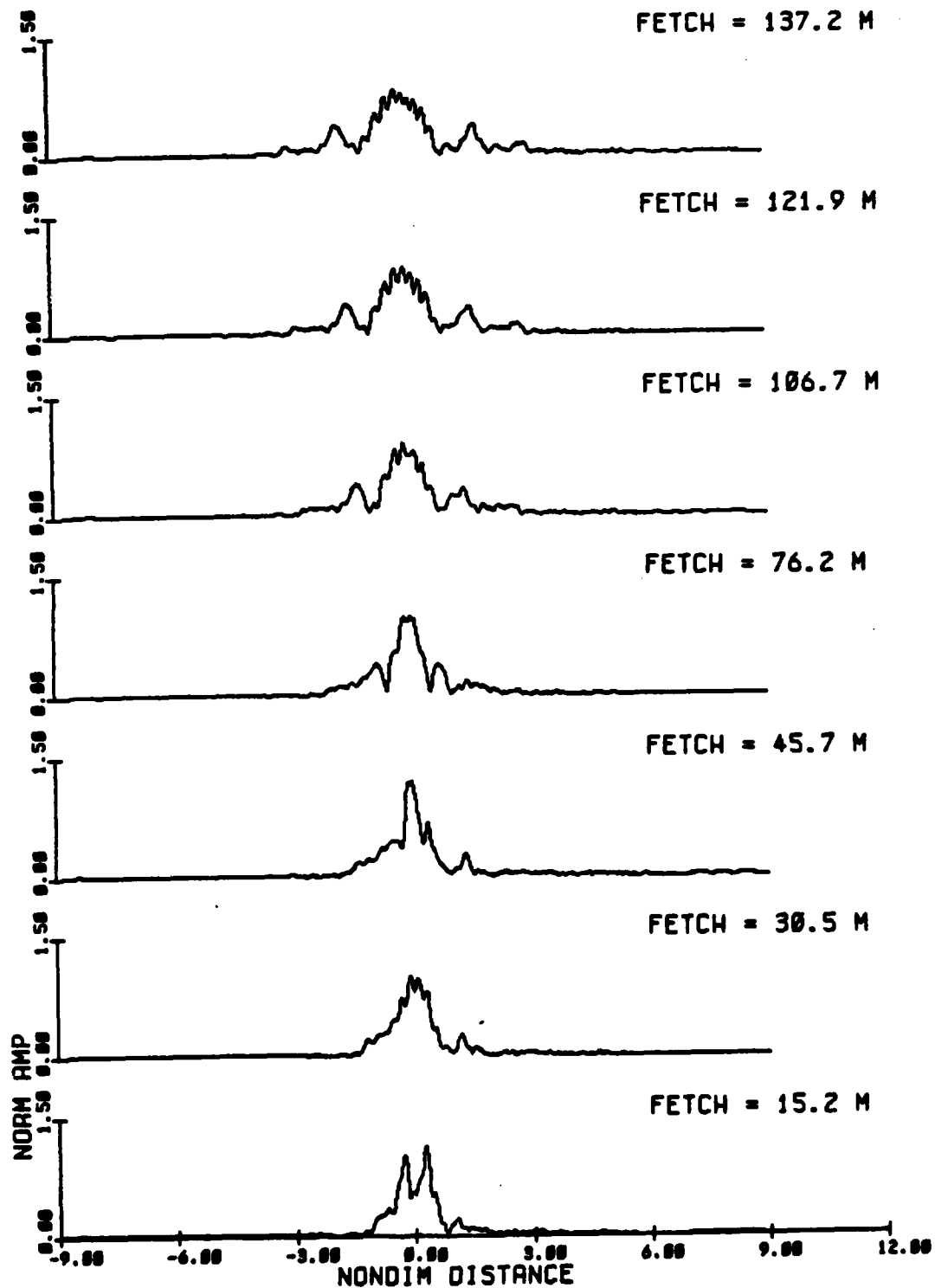
Fig. 3.21b Amplitude modulations from the inviscid NLS solution, at times corresponding to the fetches in (a), for the evolution of a group of 10 waves, initial steepness ak = .03 (Exp 78).
