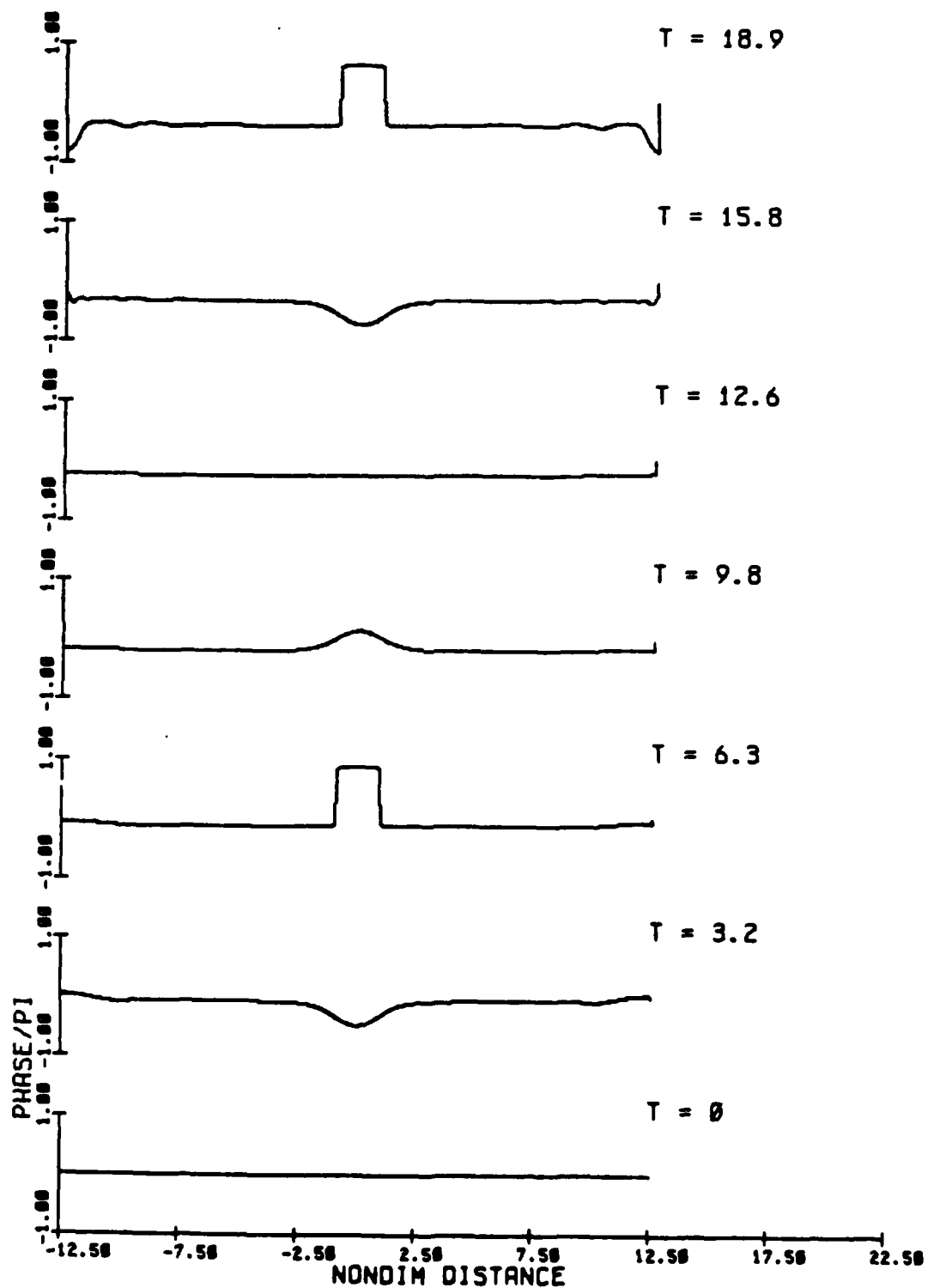
Fig. 3.8b Evolution of the principal value of the phase modulation, normalized by \pi , at 7 successive time steps corresponding to the amplitude modulation of fig. 3.8a.
