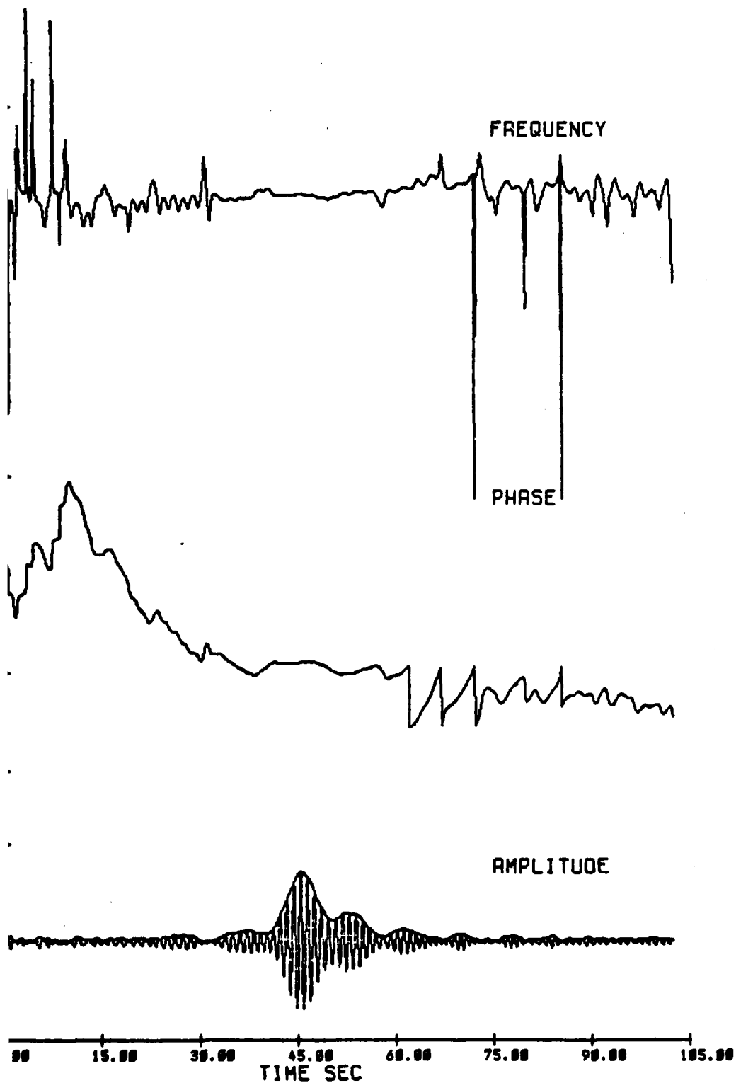
2.33 Amplitude, phase and frequency modulations at 91.4 m a group of 15 waves of initial steepness ak = .10 (Exp
