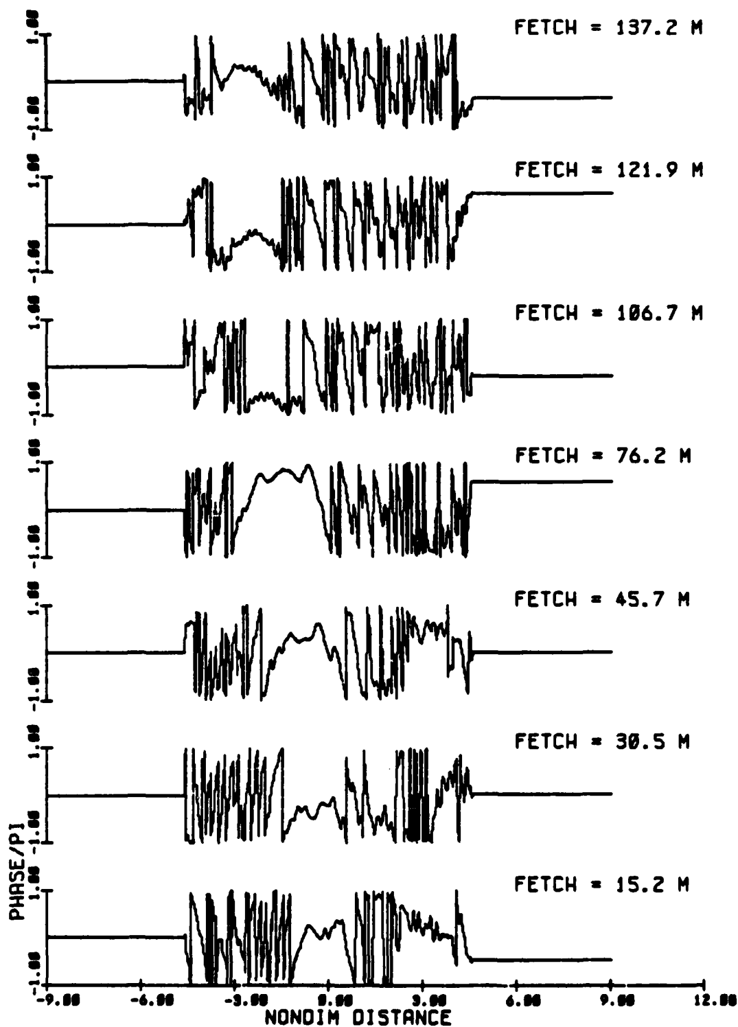
Fig. 3.22a Phase modulations from observations, principal value and normalized by \pi , for successive fetches for the evolution of a group of 10 waves, initial steepness ak = .03 (Exp 78).
