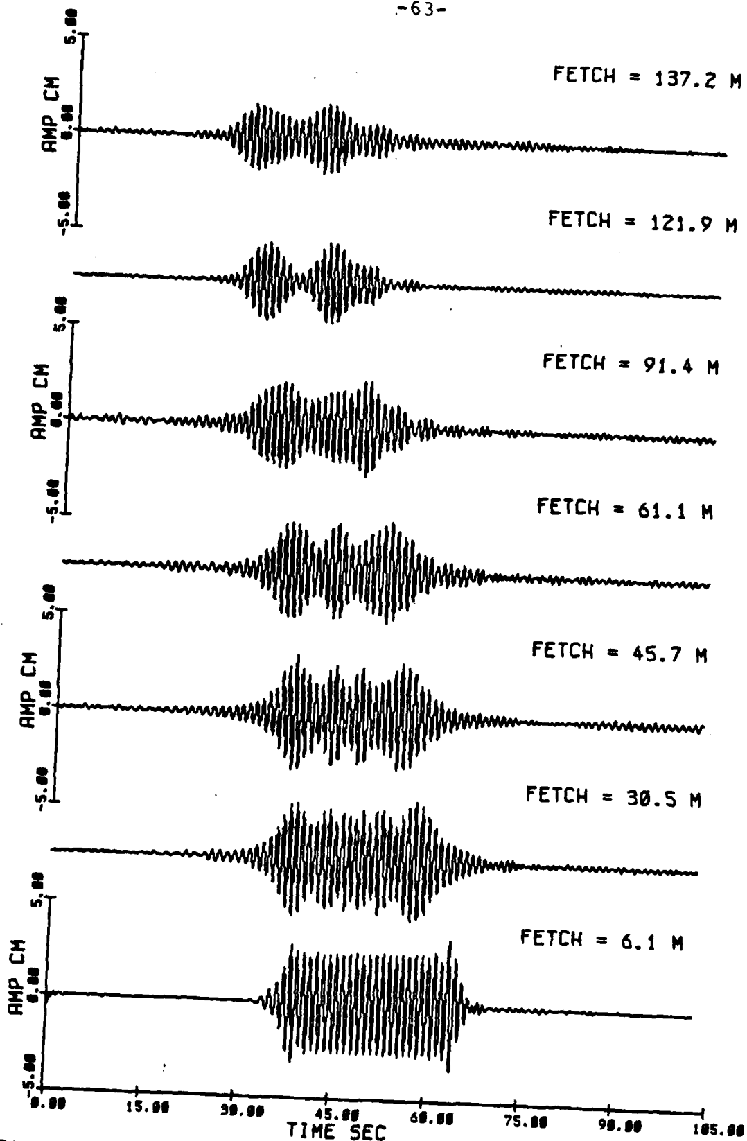
Fig. 2.7 Wave group development with fetch for a group of 25 waves of initial steepness ak = .10 (Exp 88).
