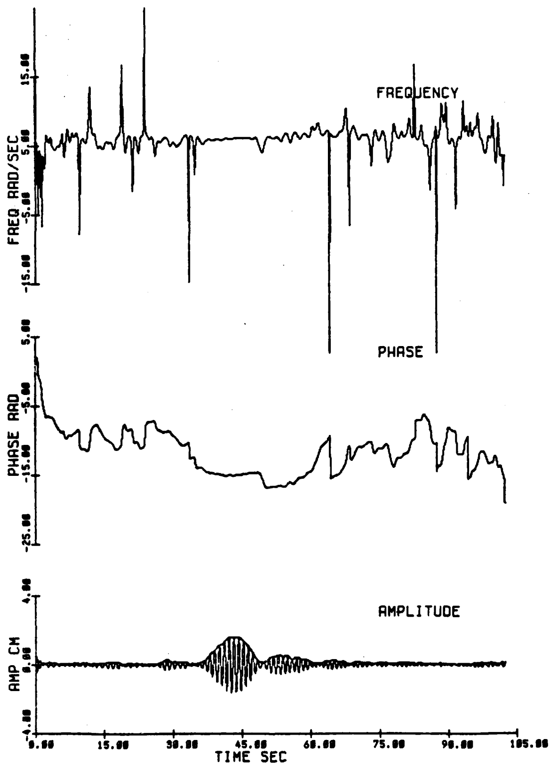
Fig. 2.35 Amplitude, phase and frequency modulations at 137.2 m for a group of 15 waves of initial steepness ak = .10 (Exp 87).
