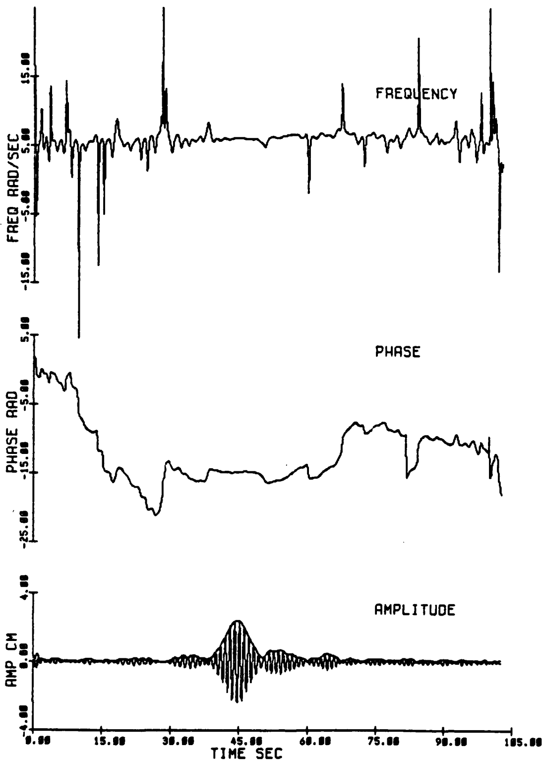
Fig. 2.34 Amplitude, phase and frequency modulations at 106.7 m for a group of 15 waves of initial steepness ak = .10 (Exp 87).
