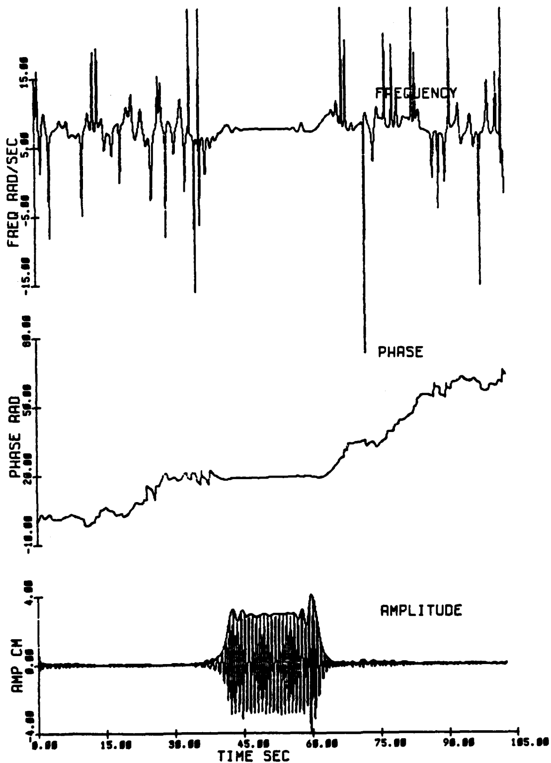
Fig. 2.36 Amplitude, phase and frequency modulations at 6.1 m for a group of 25 waves of initial steepness ak = .16 (Exp 23).
