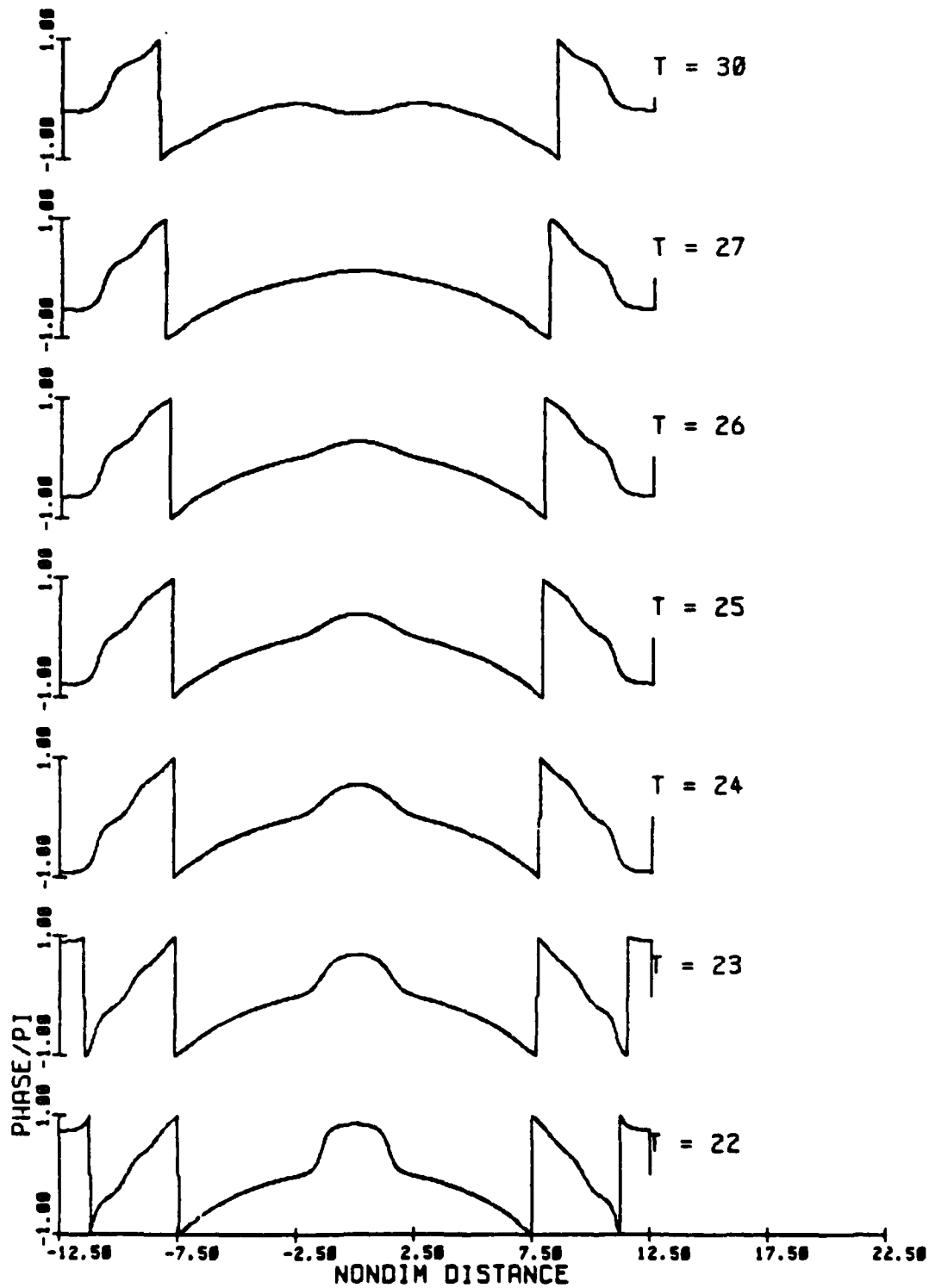
Fig. 3.11d Further evolution of the principal value of the phase modulation, normalized by \pi , at 7 successive time steps corresponding to the amplitude modulation of fig. 3.11c.
