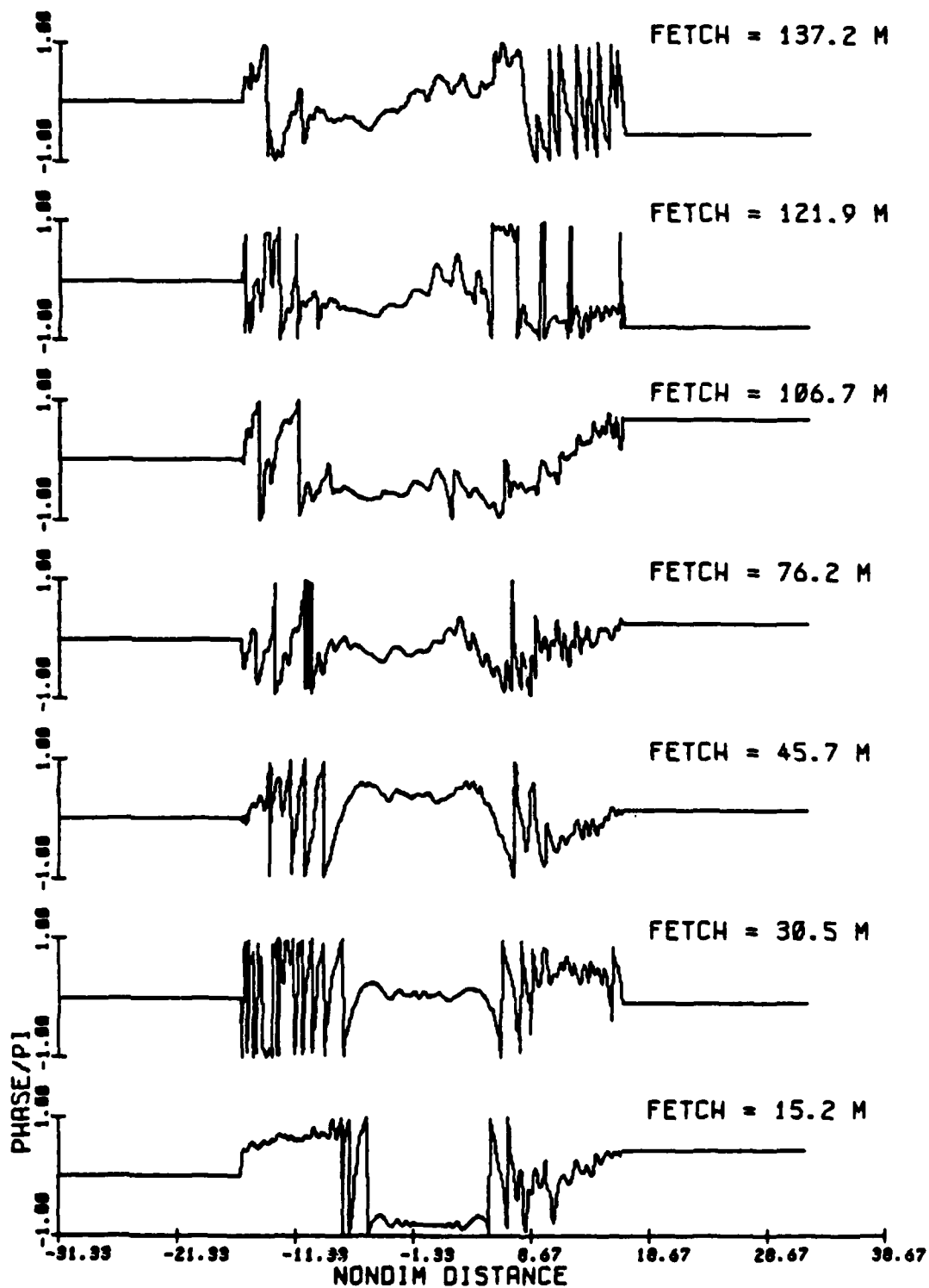
Fig. 3.37a Phase modulations from observations, principal value and normalized by \pi , for successive fetches for the evolution of a group of 25 waves, initial steepness ak = .10 (Exp 88).
