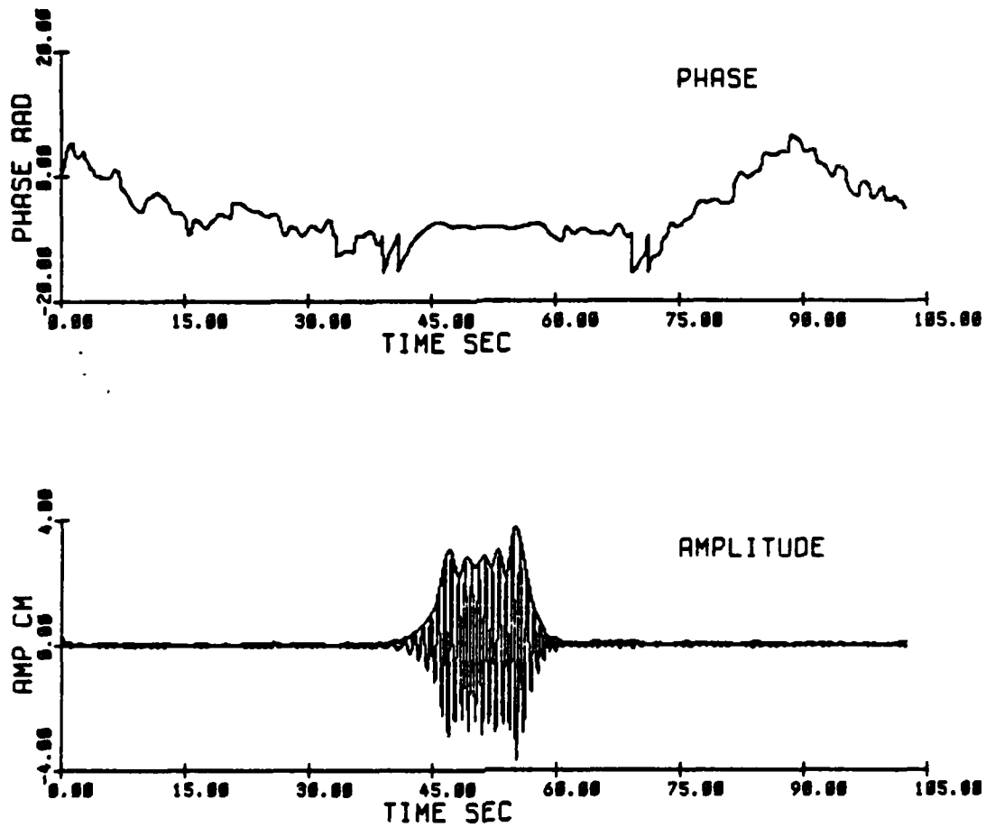
Fig 3.40 Initial condition at 6.1 m (E62) ok = .15, N = 15
