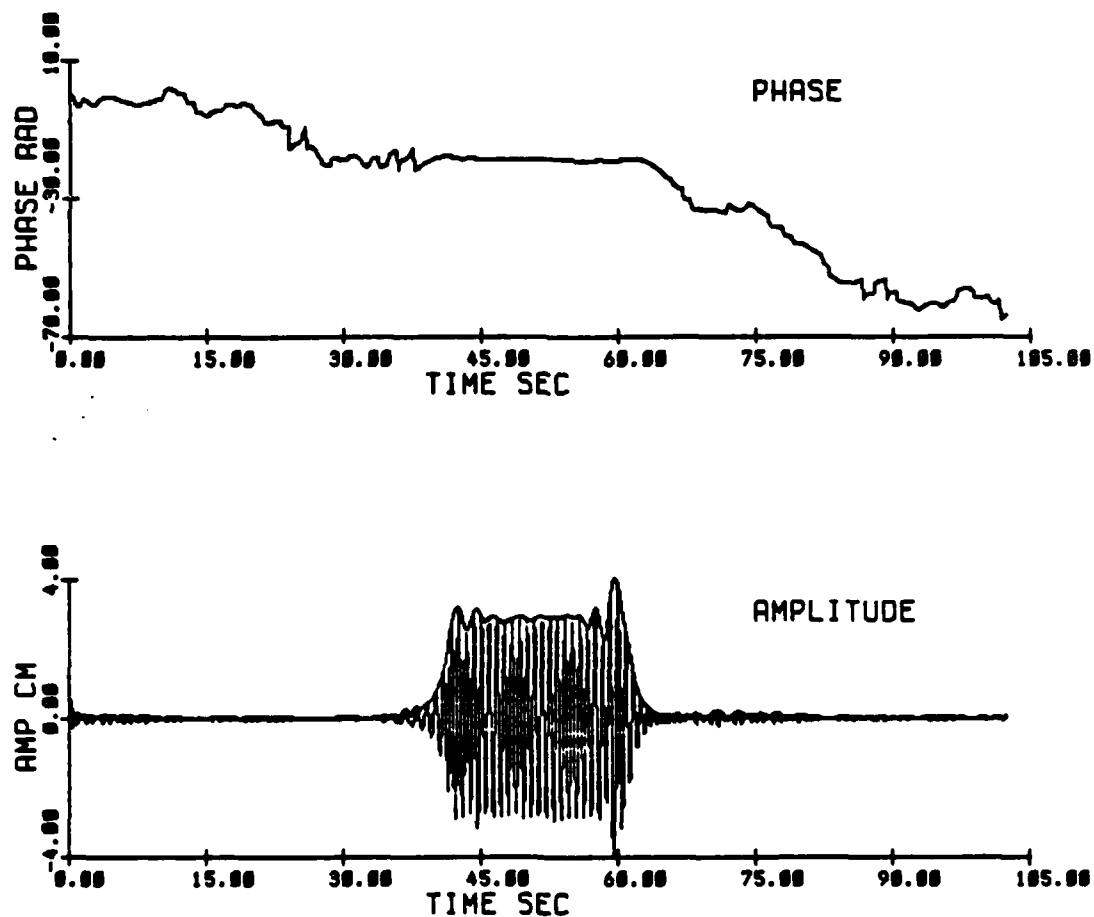
Fig 3.50 Initial condition at 6.1 m (E23) ak = .16, N = 25
