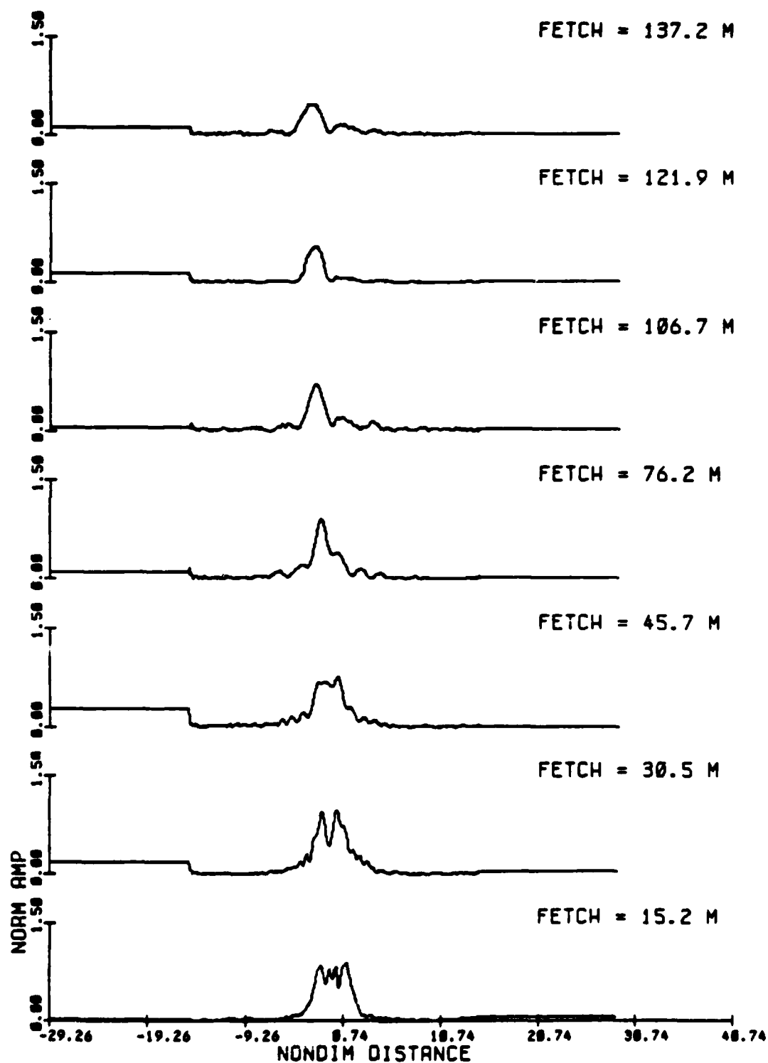
Fig. 3.31a Amplitude modulations from observations, nondimensionalized at each fetch by the initial condition scaling, for the evolution of a group of 15 waves, initial steepness ak = .10 (Exp 87).
