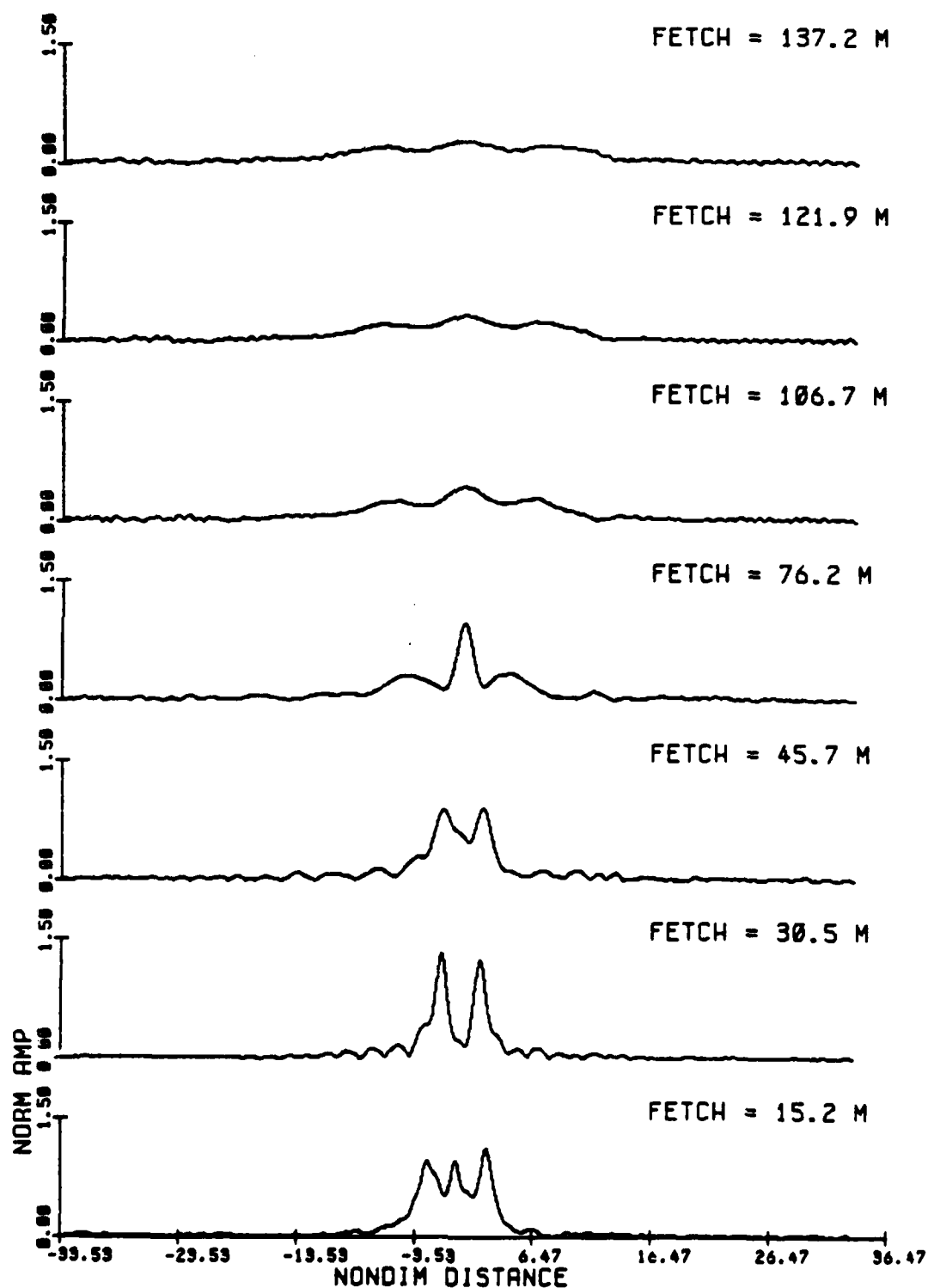
Fig. 3.46c-Amplitude modulations from the viscous NLS solution, at times corresponding to the fetches in (a), for the evolution of a group of 15 waves, initial steepness ak = .16 (Exp 22).
