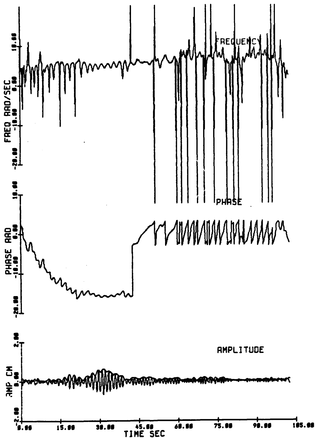
Fig. 2.27 Amplitude, phase and frequency modulations at 91.4 m for a group of 10 waves of initial steepness ak = .03 (Exp 78).
