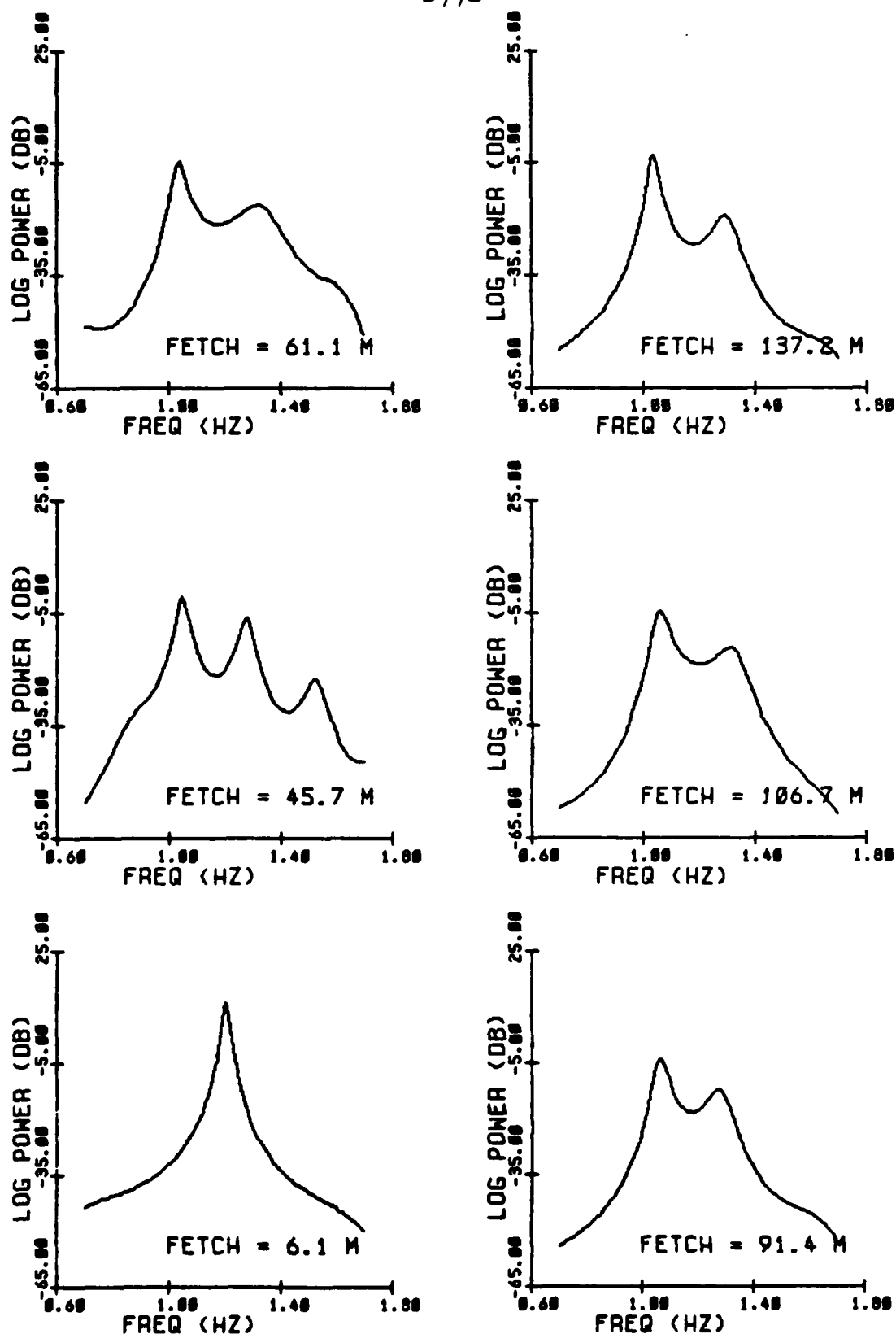
Fig. 2.16 Maximum entropy (MEM) spectral evolution with fetch for a group of 15 waves of steepness ak = .15 (Exp 62). Fetches as indicated. Group was bandpassed on the interval [0.7, 1.7] Hz centered on the initial carrier frequency 1.20 Hz. Filter rolloff occurs at the bandedges.
