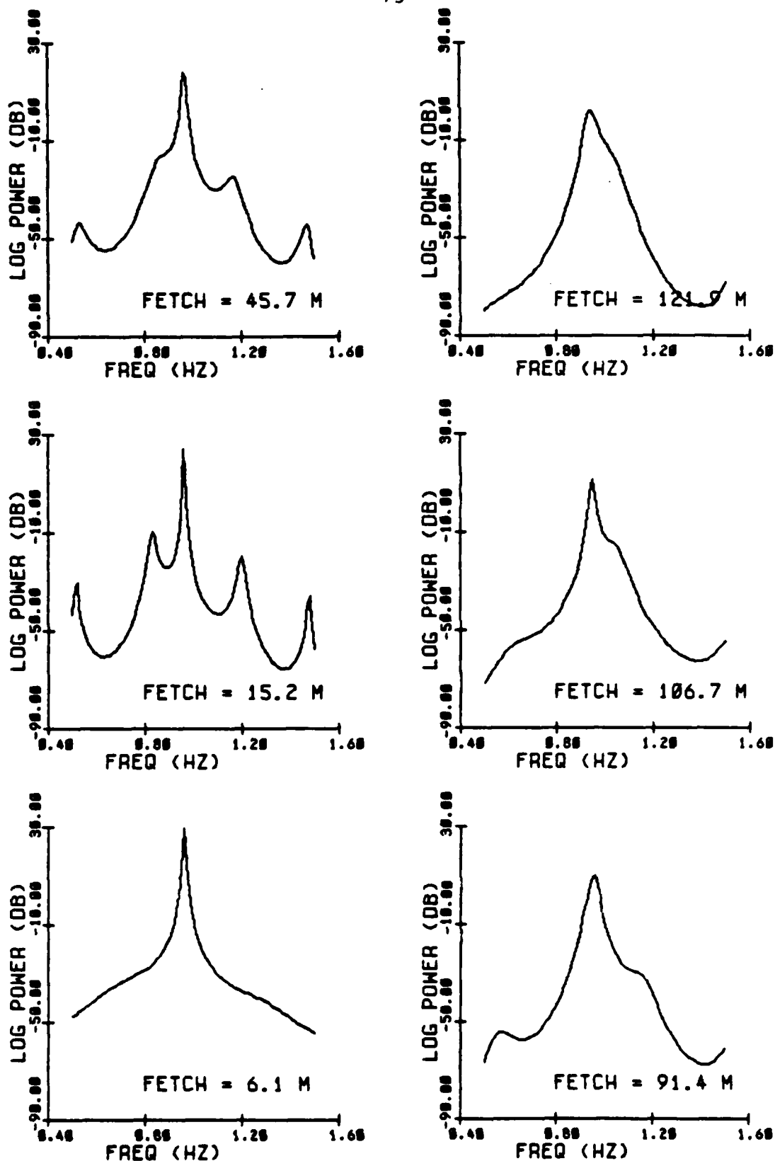
Fig. 2.14 Maximum entropy (MEM) spectral evolution with fetch for a group of 25 waves of steepness ak = .10 (Exp 88). Fetches as indicated. Group was bandpassed on the interval [.5, 1.5] Hz centered on the initial carrier frequency 0.96 Hz. Filter rolloff occurs at the bandedges.
