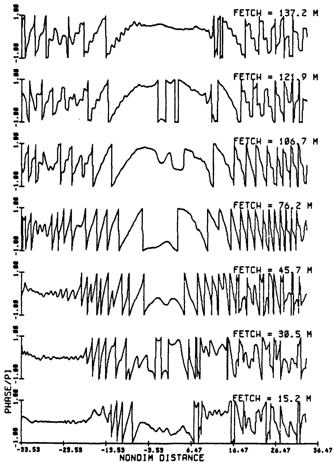
Fig. 3.47b Phase modulations from the inviscid NLS solution, at times corresponding to the fetches in (a), for the evolution of a group of 15 waves, initial steepness ak = .16 (Exp 22).
