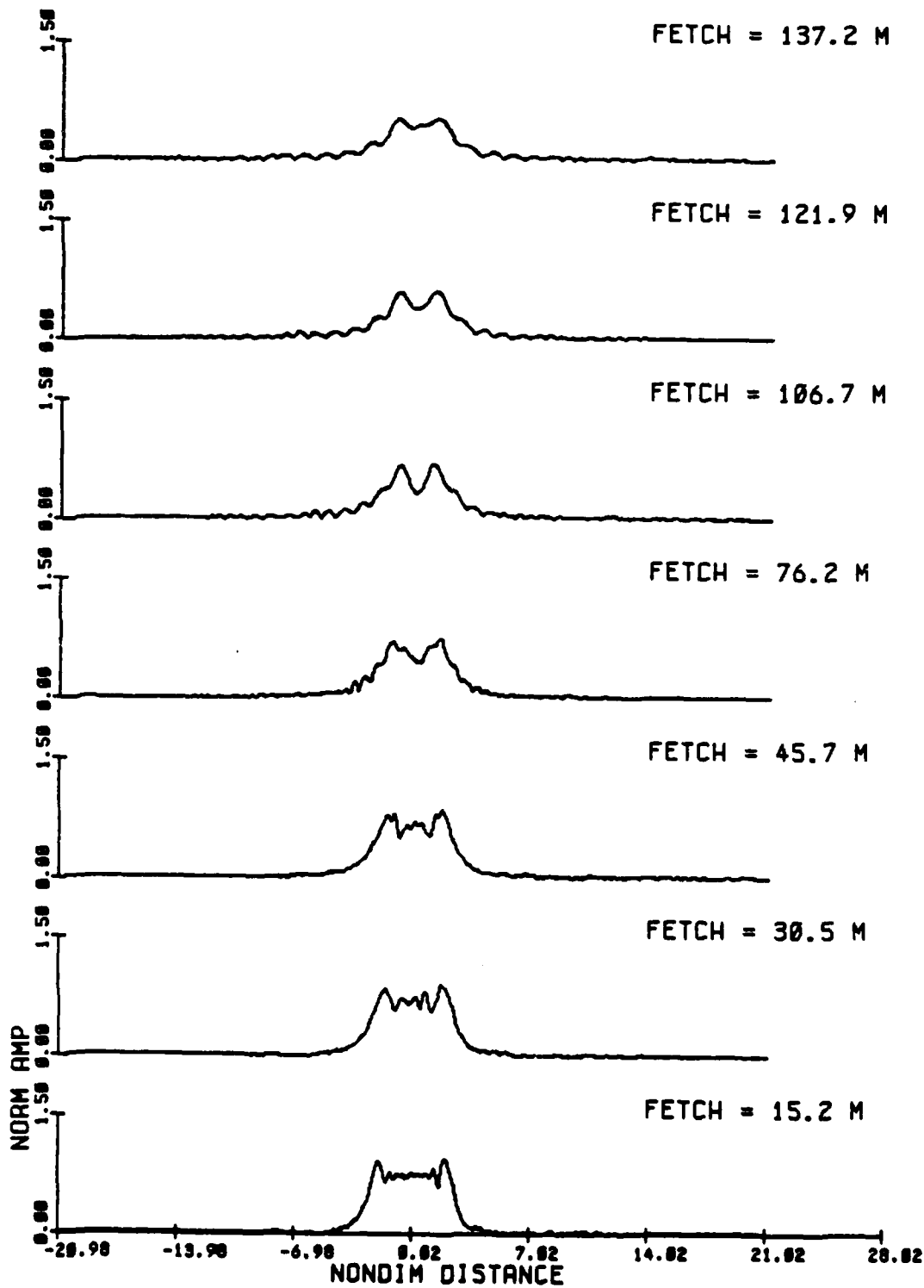
Fig. 3.26c Amplitude modulations from the viscous NLS solution, at times corresponding to the fetches in (a), for the evolution of a group of 25 waves, initial steepness ak = .07 (Exp 77).
