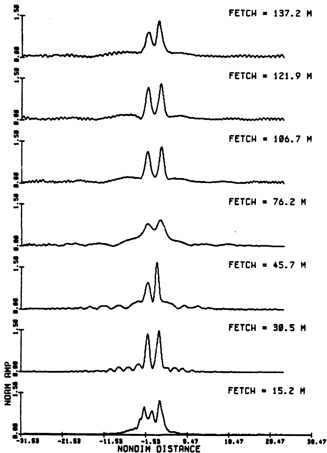
Fig. 3.41b Amplitude modulations from the inviscid NLS solution, at times corresponding to the fetches in (a), for the evolution of a group of 15 waves, initial steepness ak = .15 (Exp 62).
