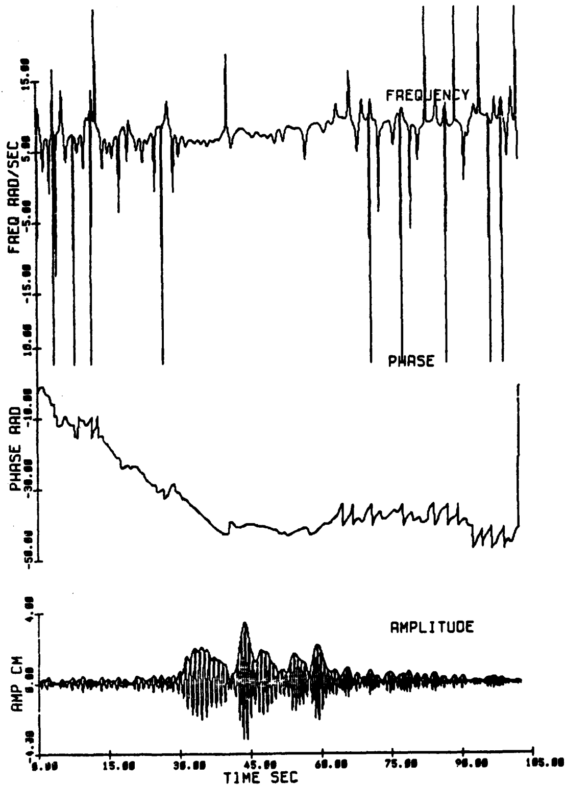
Fig. 2.39 Amplitude, phase and frequency modulations at 91.4 m for a group of 25 waves of initial steepness ak = .16 (Exp 23).
