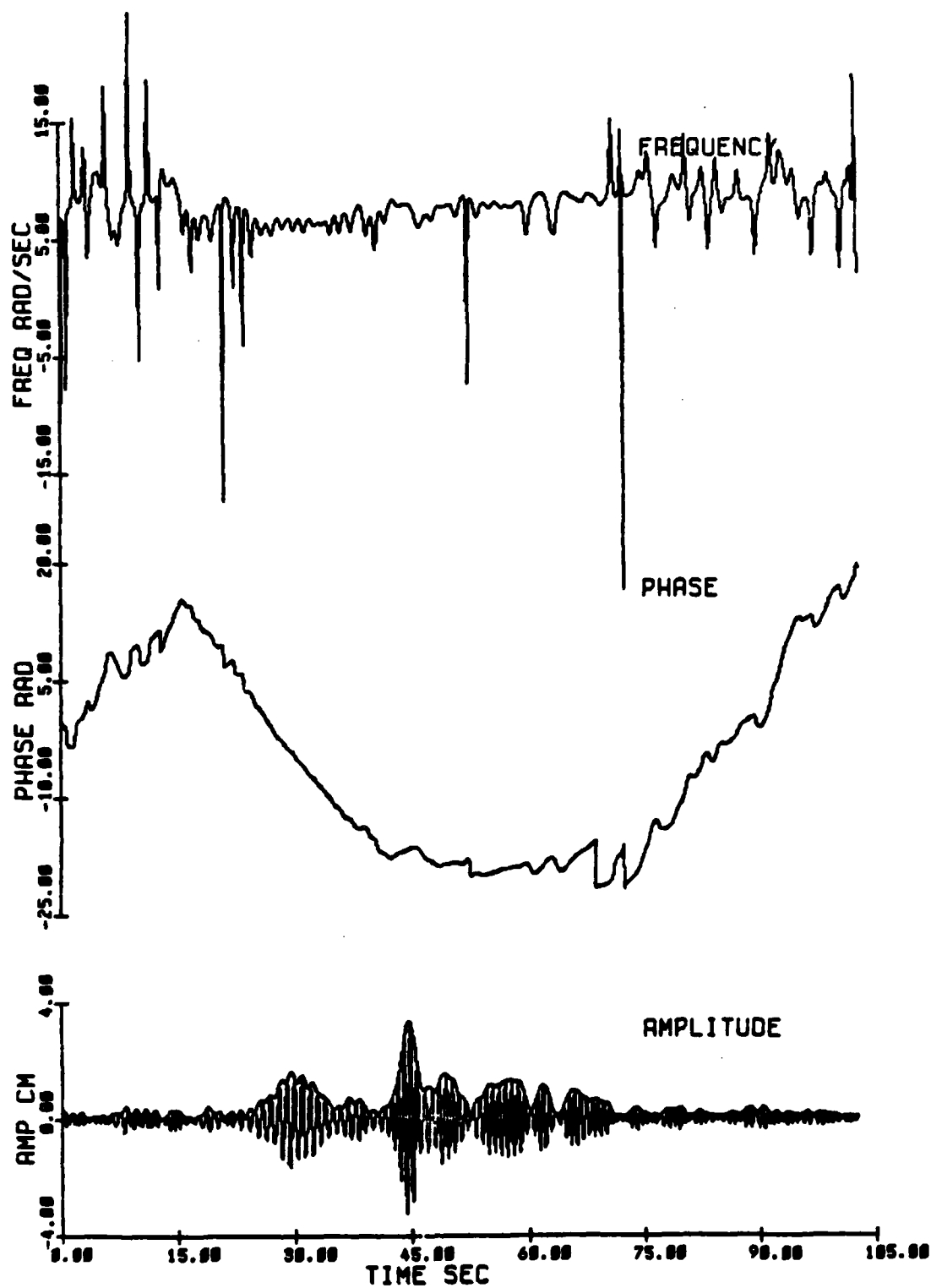
Fig. 2.40 Amplitude, phase and frequency modulations at 106.7 m for a group of 25 waves of initial steepness ak = .16 (Exp 23).
