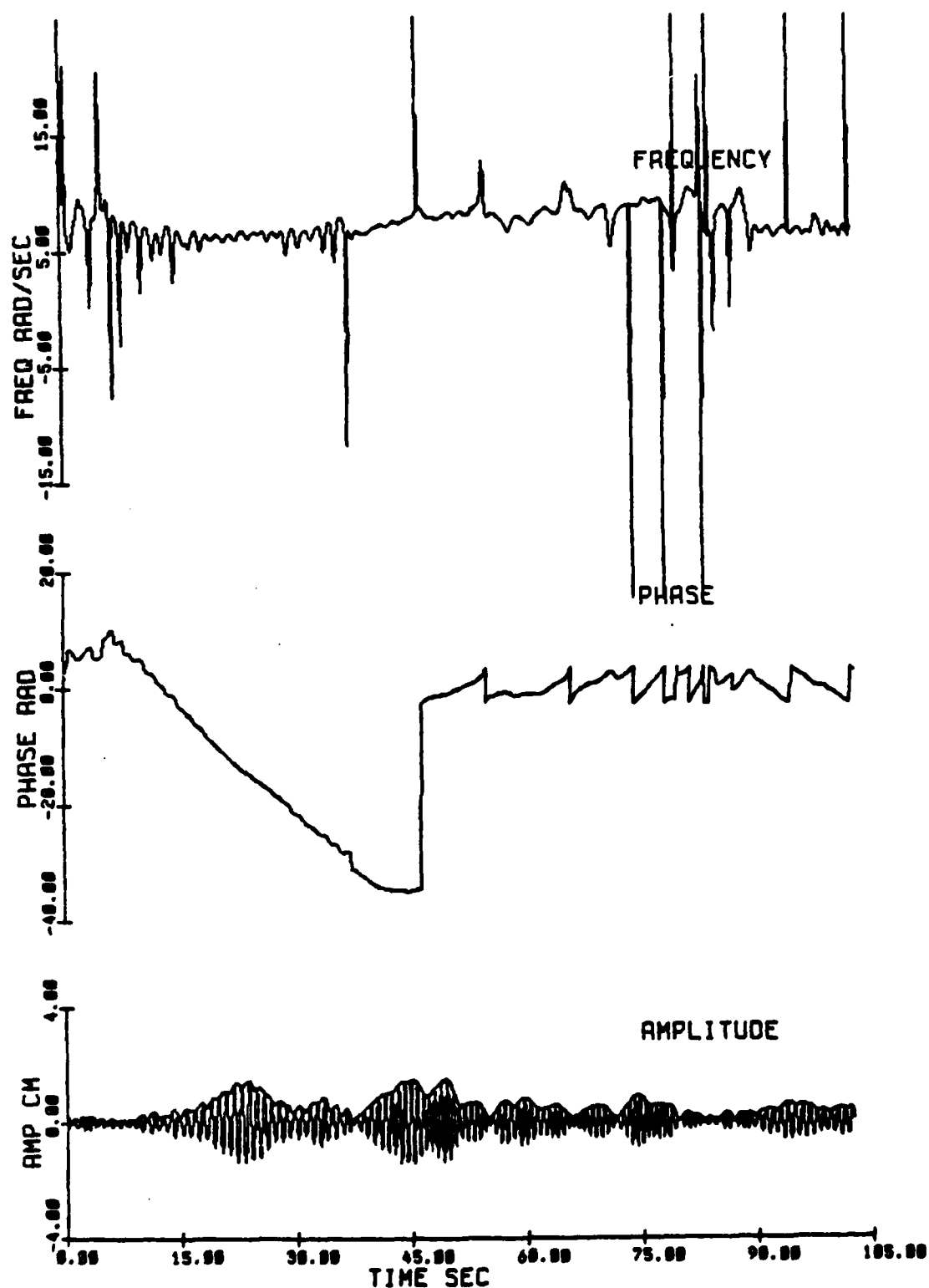
Fig. 2.41 Amplitude, phase and frequency modulations at 137.2 m for a group of 25 waves of initial steepness ak = .16 (Exp 23).
