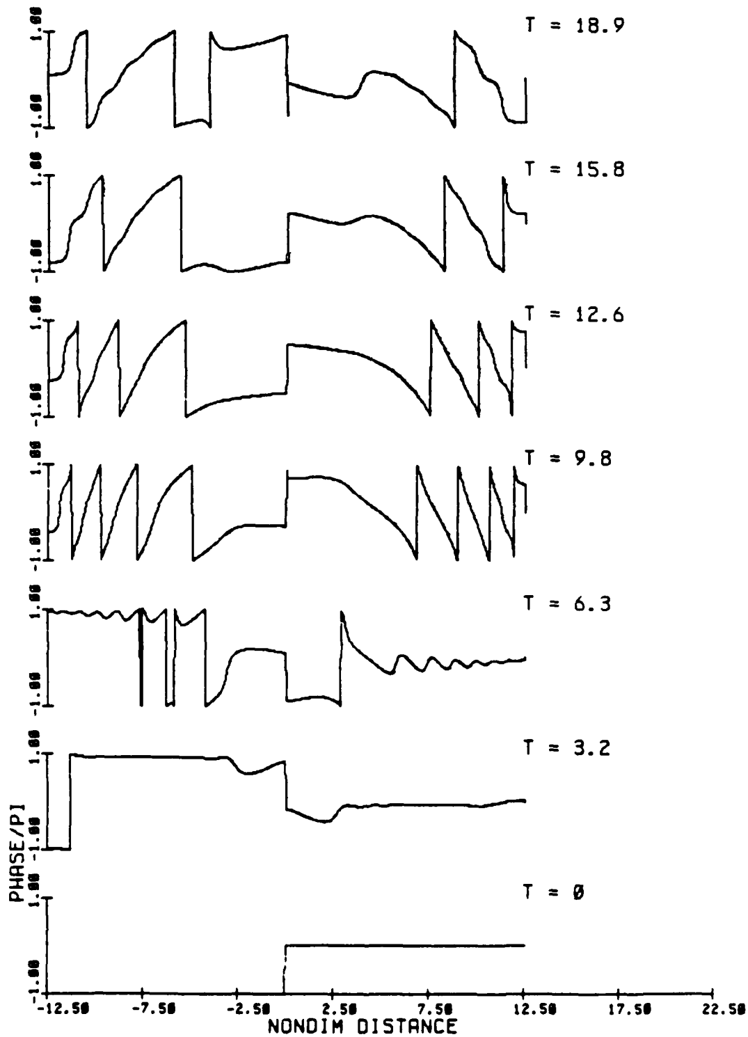
Fig. 3.16c Evolution of the principal value of the phase modulation, normalized by \pi , at 7 successive time steps corresponding to the amplitude modulation of fig. 3.16a.
