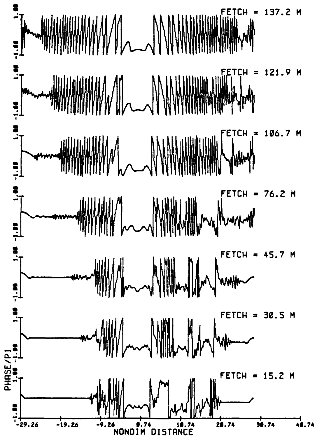
Fig. 3.32c Phase modulations from the viscous NLS solution, at times corresponding to the fetches in (a), for the evolution of a group of 15 waves, initial steepness ak = .10 (Exp 87).
