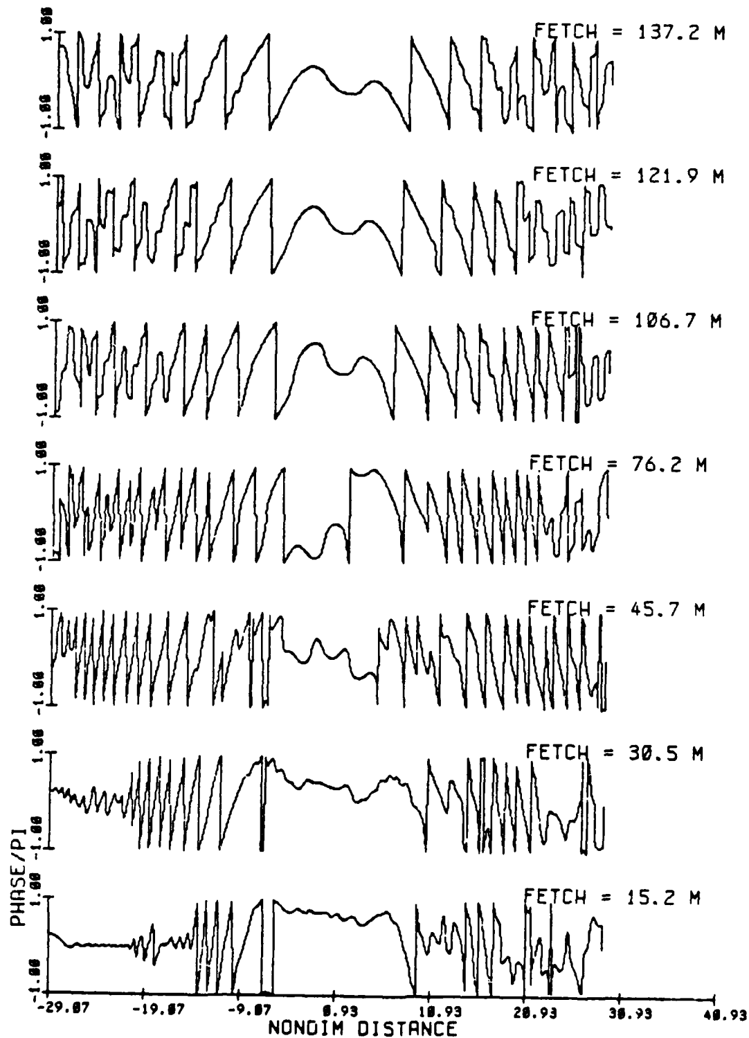
Fig. 3.52c Phase modulations from the viscous NLS solution, at times corresponding to the fetches in (a), for the evolution of a group of 25 waves, initial steepness ak = .16 (Exp 23).
