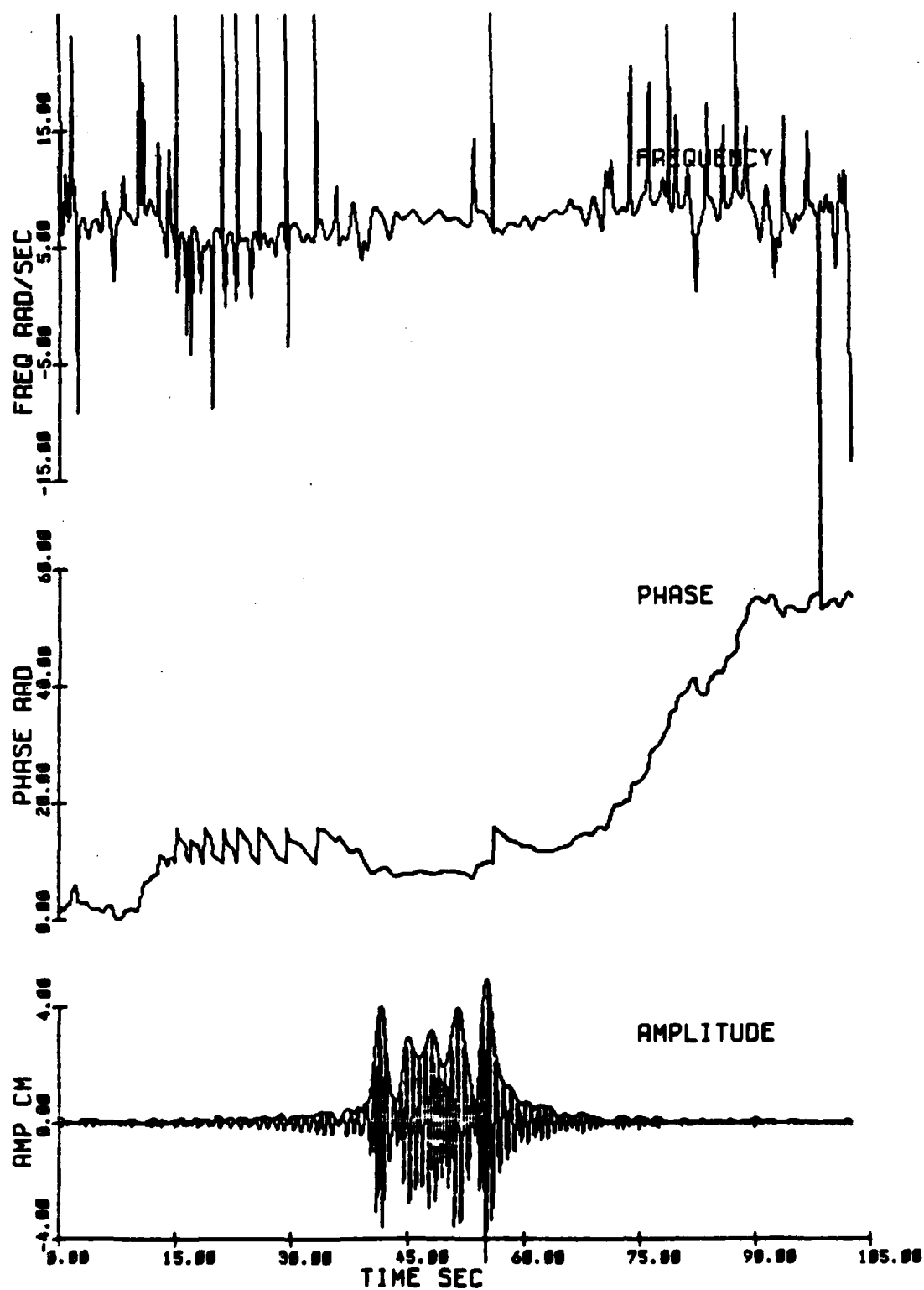
Fig. 2.37 Amplitude, phase and frequency modulations at 30.5 m for a group of 25 waves of initial steepness ak = .16 (Exp 23).
