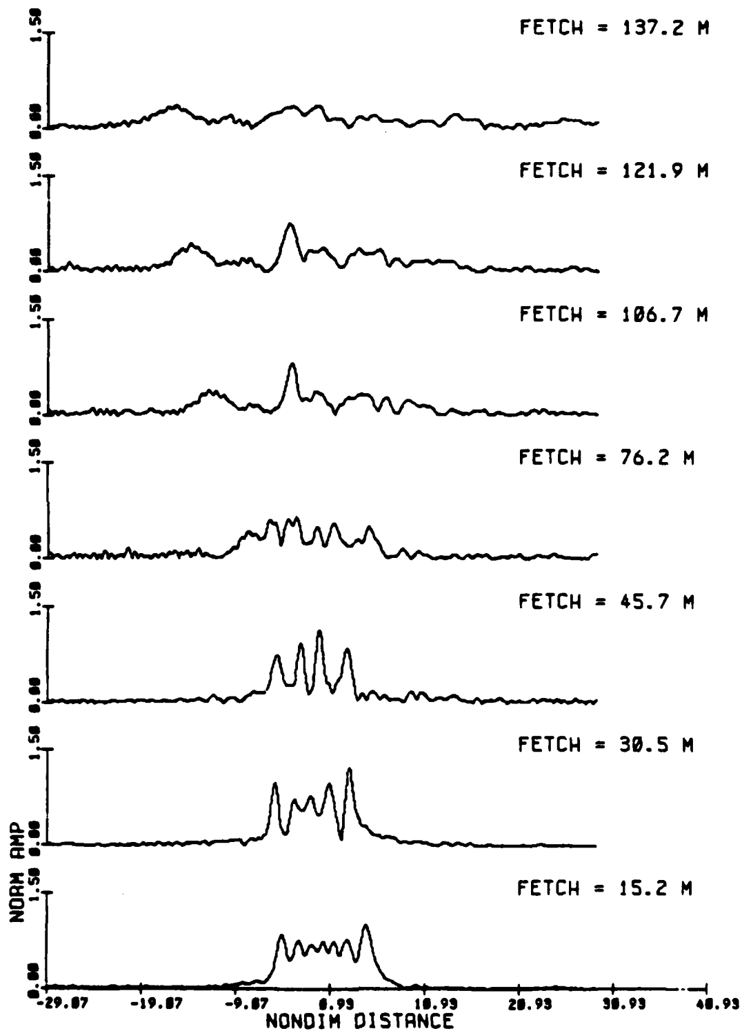
Fig. 3.51a Amplitude modulations from observations, nondimensionalized at each fetch by the initial condition scaling, for the evolution of a group of 25 waves, initial steepness ak = .16 (Exp 23).
