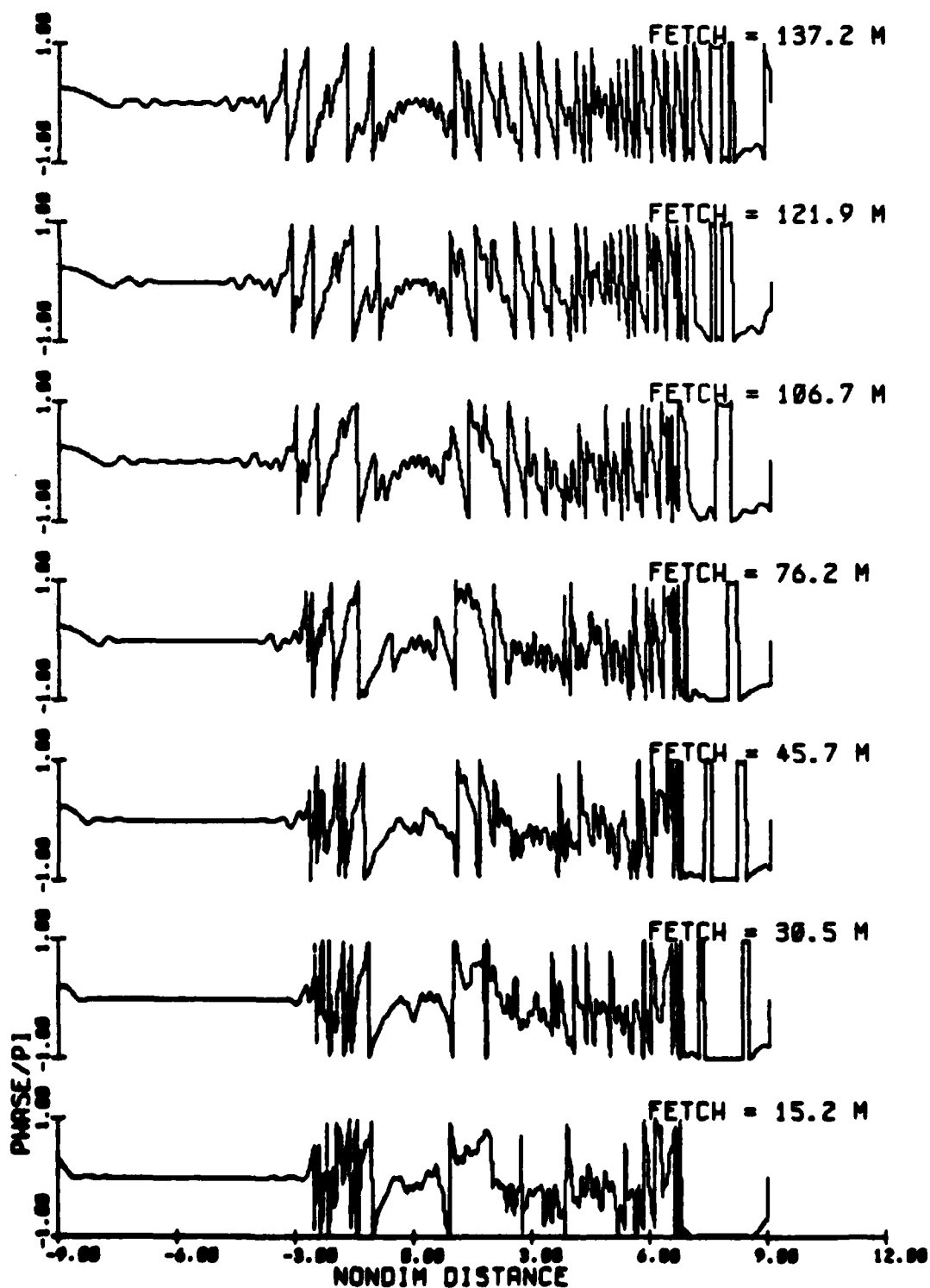
Fig. 3.22c Phase modulations from the viscous NLS solution, at times corresponding to the fetches in (a), for the evolution of a group of 10 waves, initial steepness ak = .03 (Exp 78).
