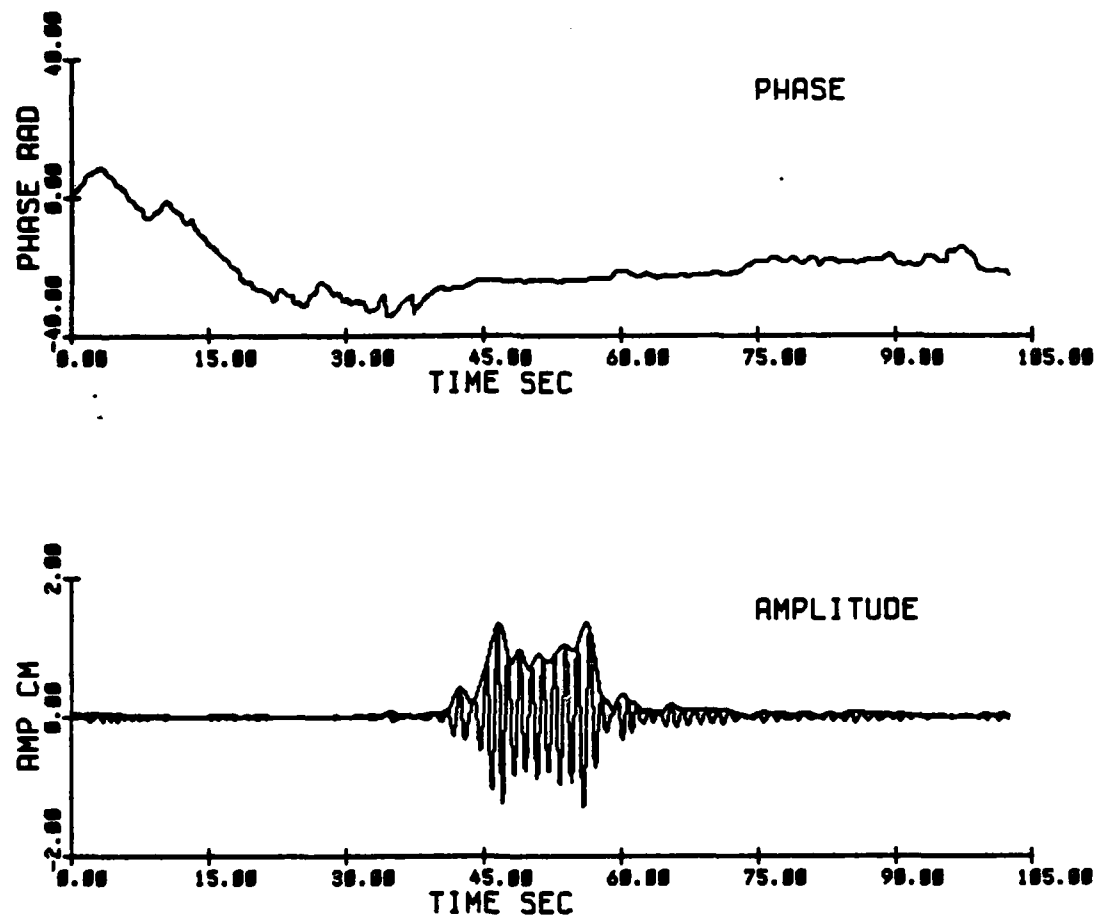
Fig 3.20 Initial condition at 6.1 m (E78) ak = .03, N = 10
