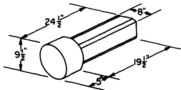
Figure 5.—Typical specimen.
