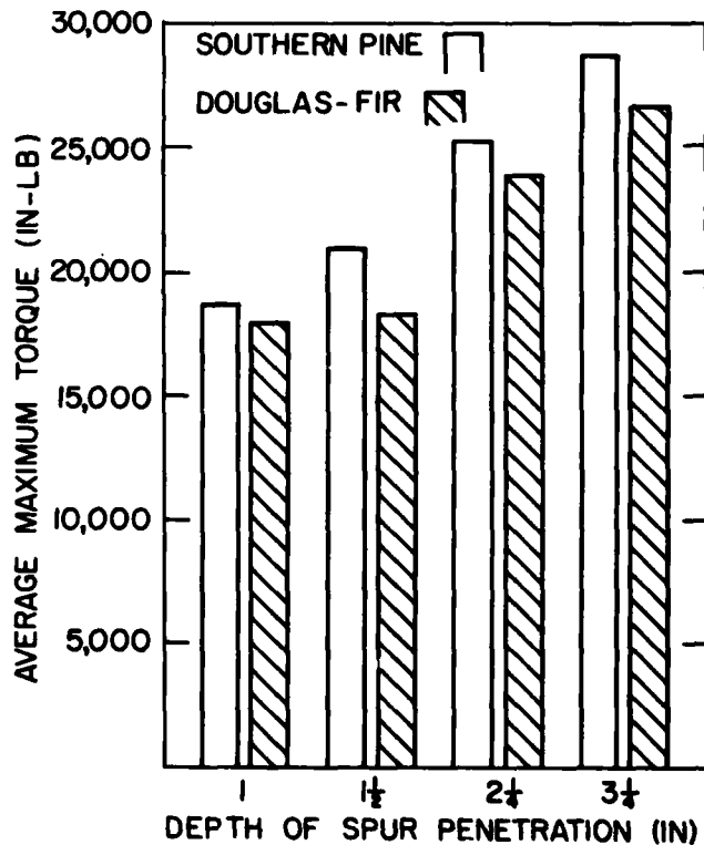
Figure 15.—Average maximum torque developed in southern pine and Douglas-fir at four spur penetration depths. Fifteen samples were taken, five at each of three temperatures: 60° F, 120° F, 150° F. (M 149 934)
