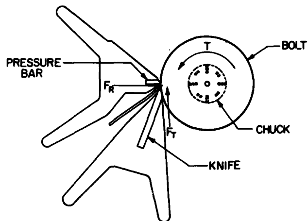
Figure 1.—Cross section of a veneer lathe showing resultant cutting forces and torque.
