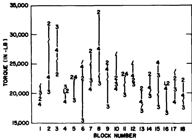
Figure 11.—Torque developed with each chuck on each block (Douglas-fir).
