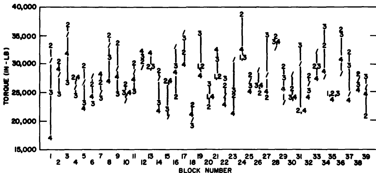
Figure 9.—Torque developed by each chuck on each block (southern pine).
