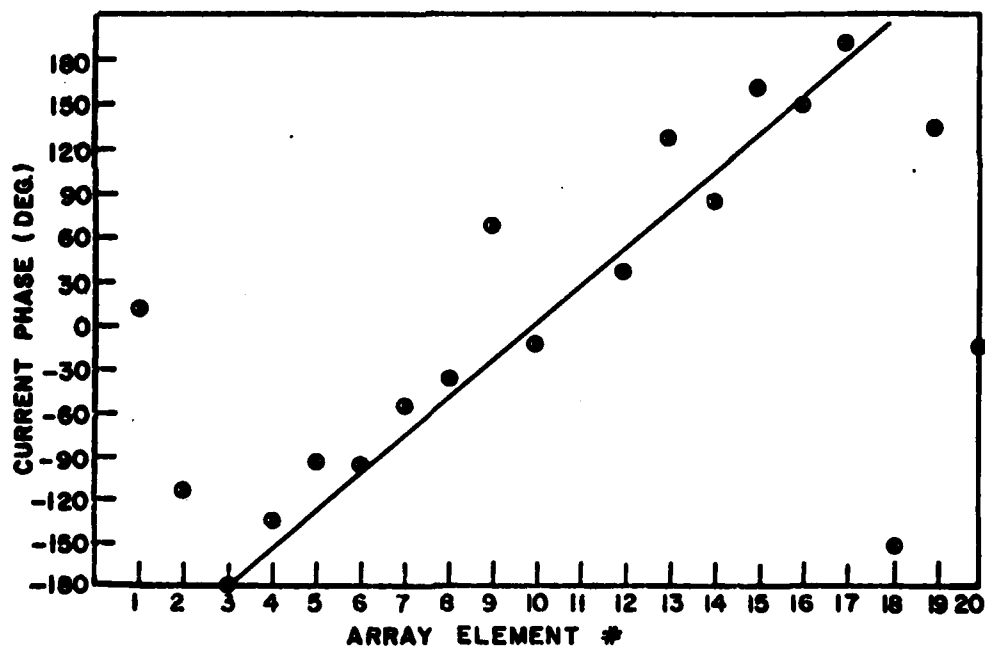
Figure 61: Constrained array current plots ( y=15.8 cm, |I_c|=1.6 \times 10^{-3} )
