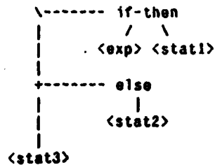
Figure 6-3: Before restructuring.
