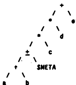
Figure 4-26: After macrotwiddleright .
