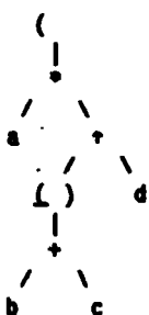
Figure 4-31: After matchparens.
