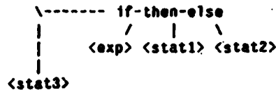
Figure 6-4: After restructuring.
