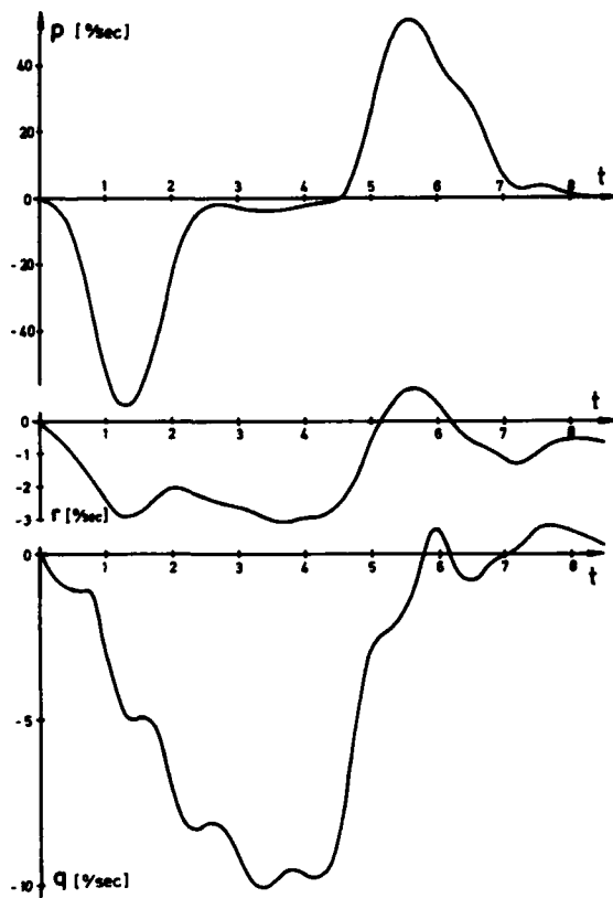
FIG. 10 INPUT ANGULAR RATES MEASURED AND SMOOTHED
