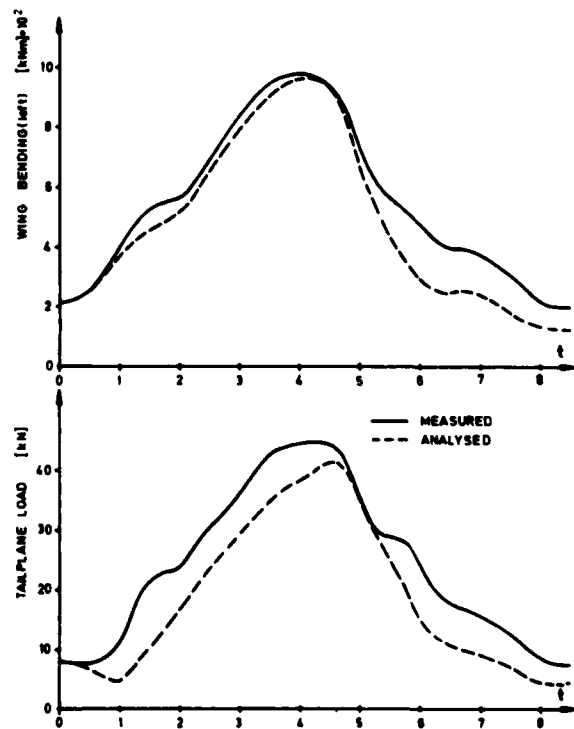
FIG. 13 LOADS ON WING AND TAILPLANE
