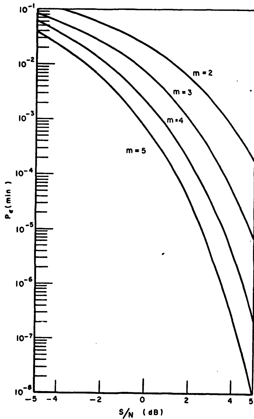
Fig. 4-19-- P_e(\min) vs. (S/N) given h_w/h_n = 1 .
