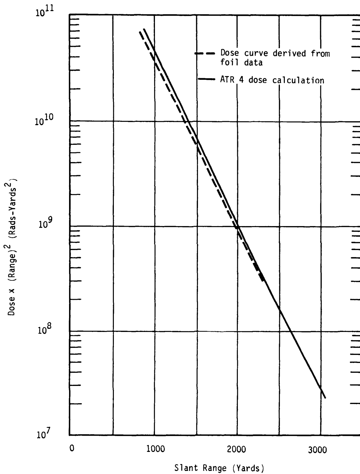
Figure 3-3. Shot Hood Neutron Dose.
