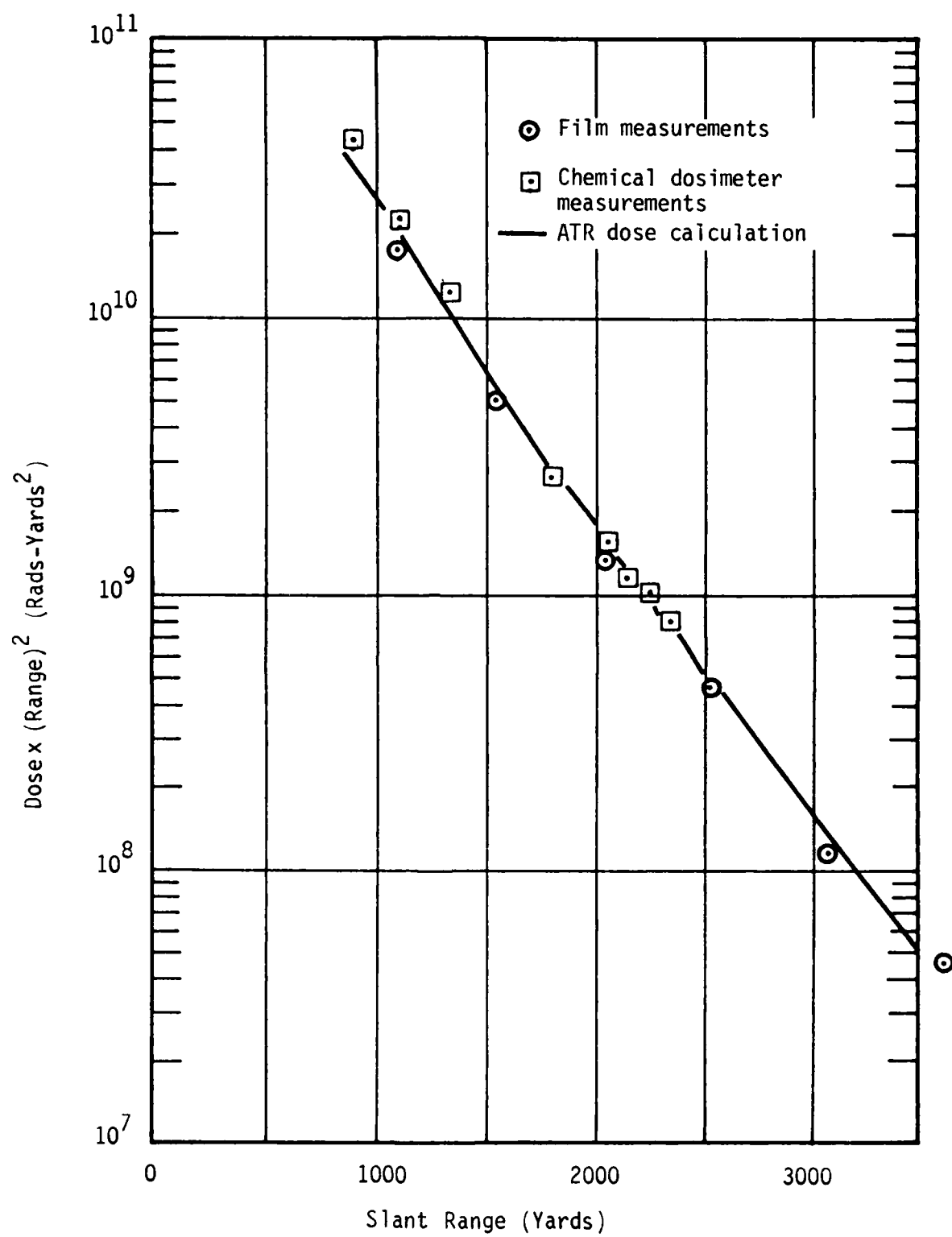
Figure 3-4. Shot Hood Gamma Dose.
