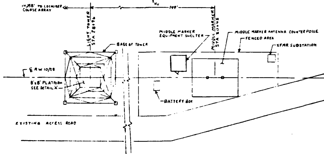
R/W 10 MIDDLE MARKER PLOT PLAN SITE B
