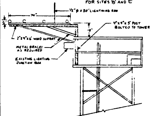
DETAIL B PROFILE VIEW OF ANTENNA INSTALLATION ON ALS TOWER TYPICAL SITES B AND C
