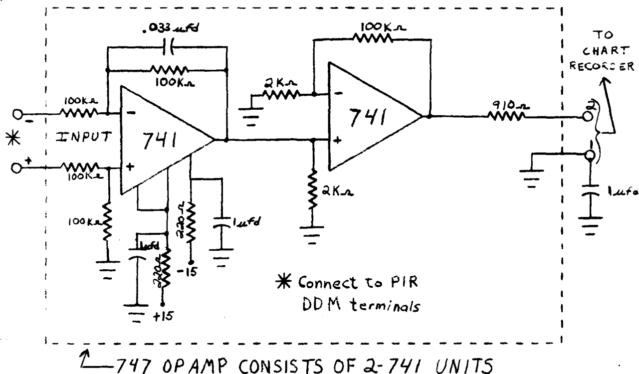
Figure 4-1. PIR Buffer Amplifier Schematic
