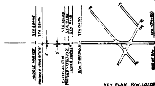
KEY PLAN R/W 10/20
