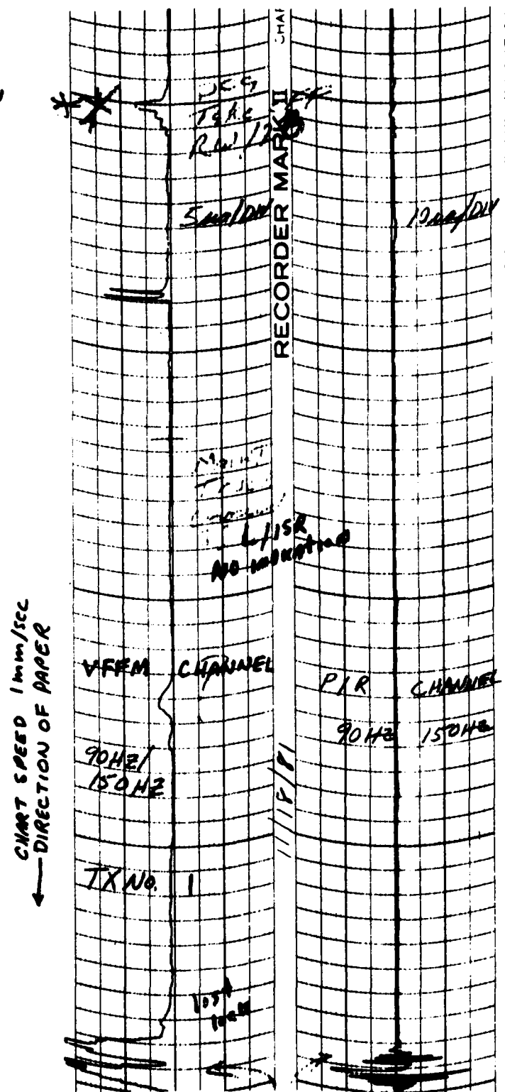
Figure 5-10. BWI R/W 15R Monitored Localizer Data. Aircraft Takeoff on Intersecting Runway.
