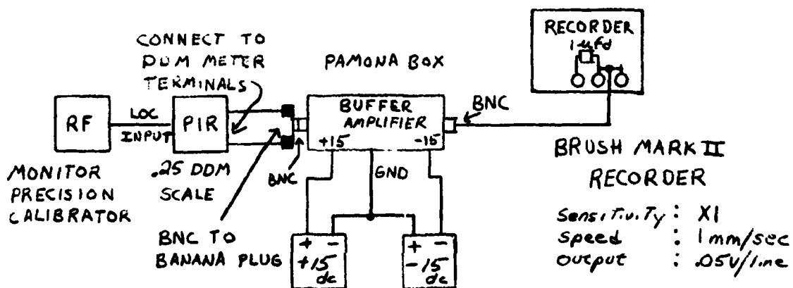
Figure 4-2. Test Setup for PIR Chart Recorder Connection
