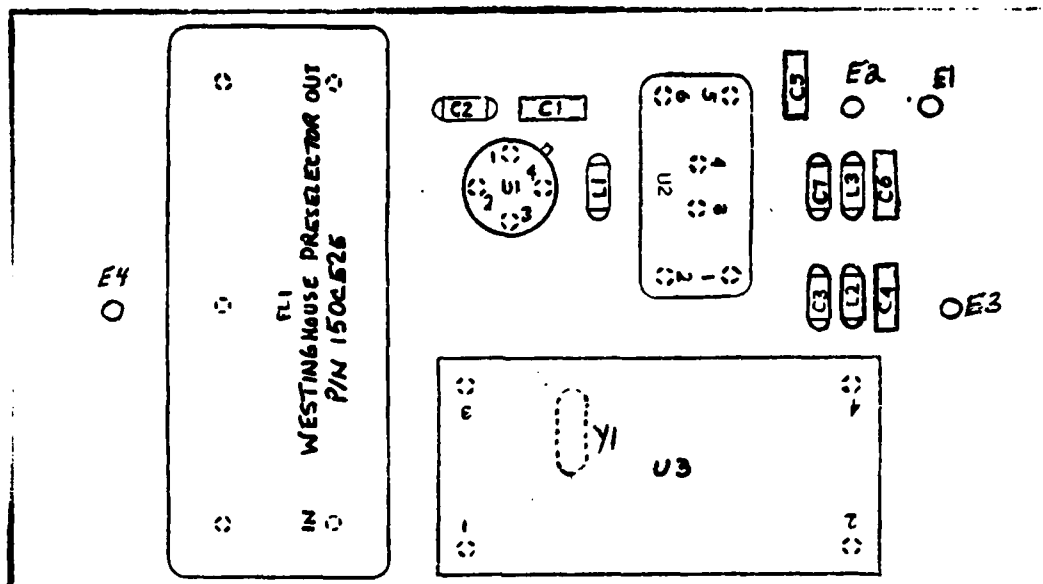
A2 RF AMP/LO COMPONENT LAYOUT
