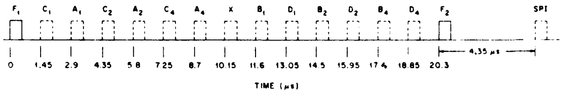
Fig. 2-2. ATCRBS Reply
