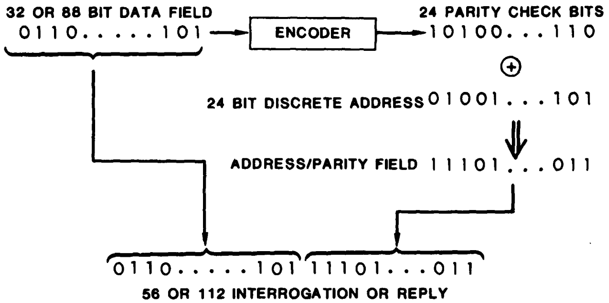
Fig. 2-7. Address/Parity Field Generation.
