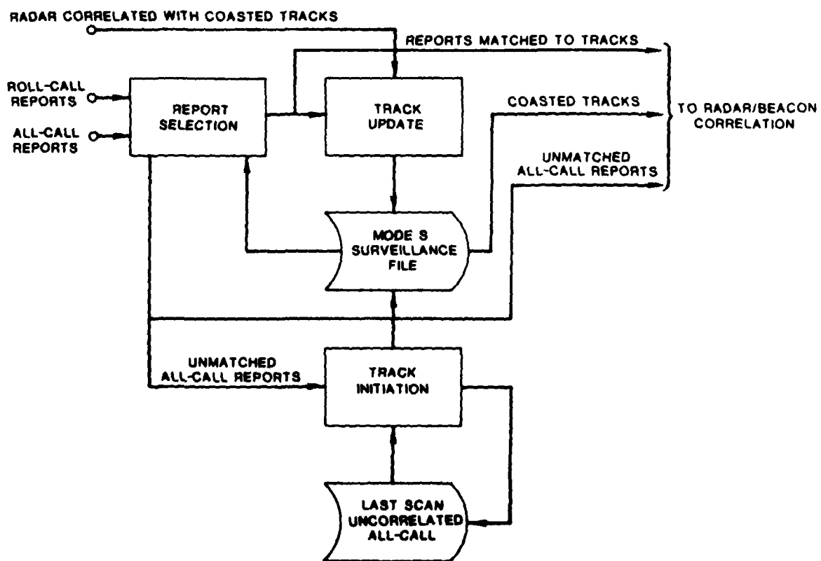
Fig. 3-15. Mode S Surveillance Processing
