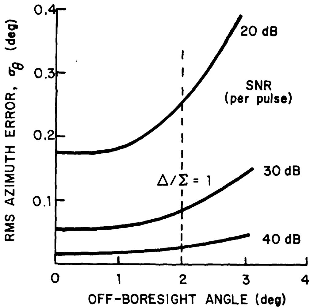
Fig. 5-5. Noise Induced Monopulse Error.
