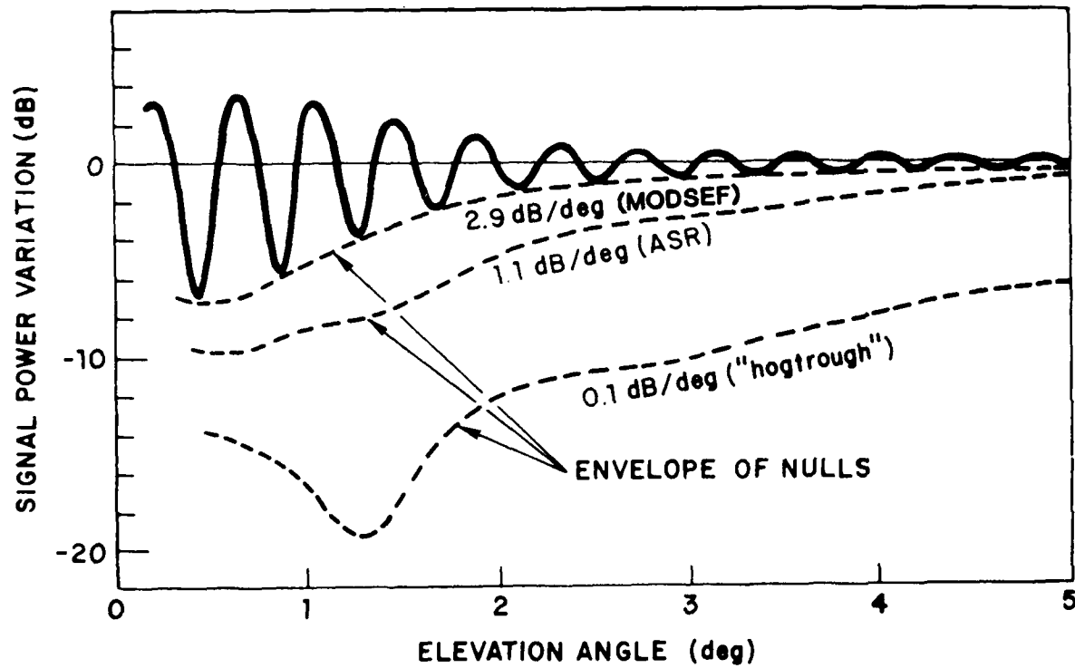
Fig. 5-1. Vertical Lobing.
