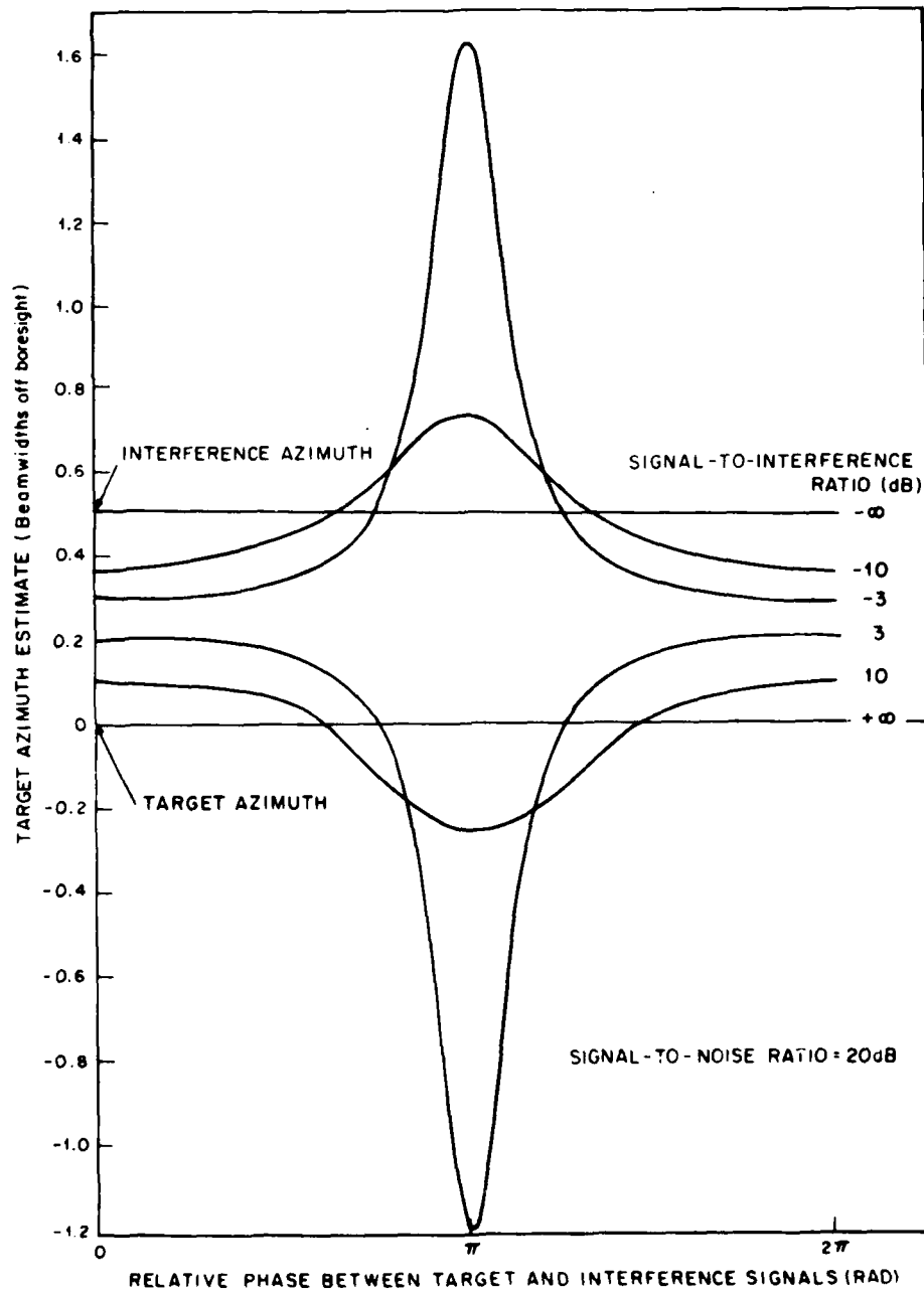
Fig. 5-6. Monopulse Estimate With Interference.
