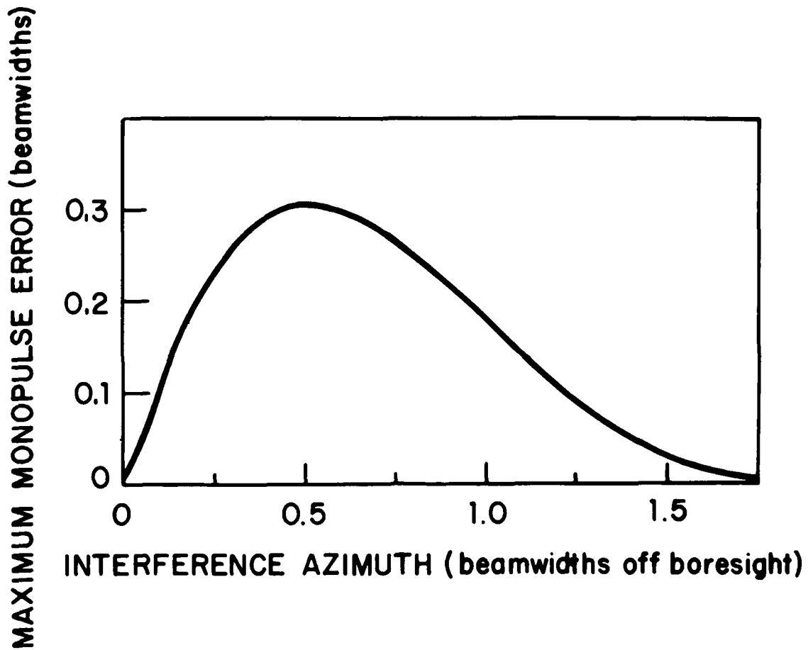
Fig. 5-7. Maximum Monopulse Error With Target On Boresight.
