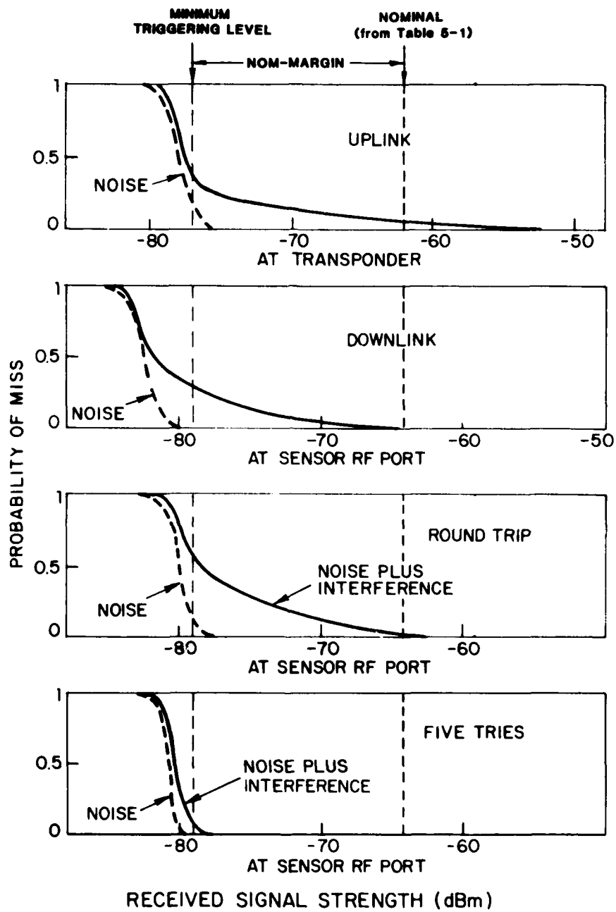
Fig. 5-3. Miss Probability.
