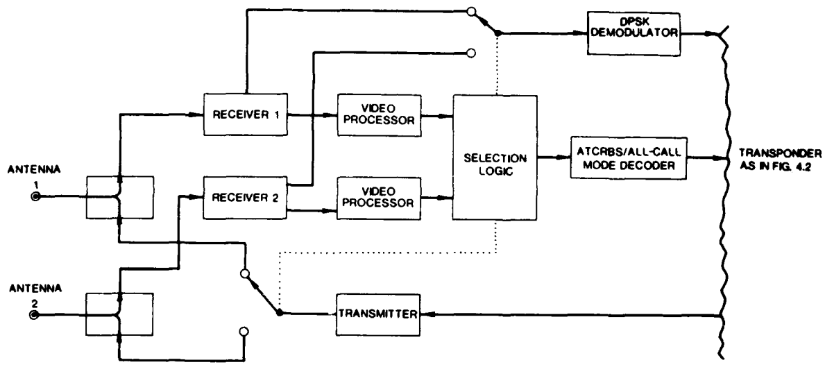
Fig. 4-3. Diversity Transponder.
