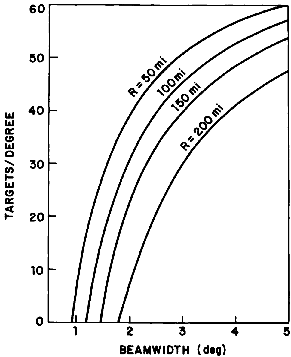
Fig. 5-8. Capacity Plots.
