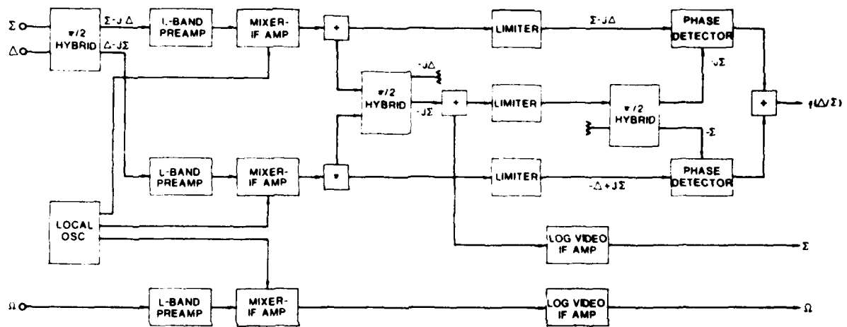
Fig. 3-10. Multi-channel Receiver.
