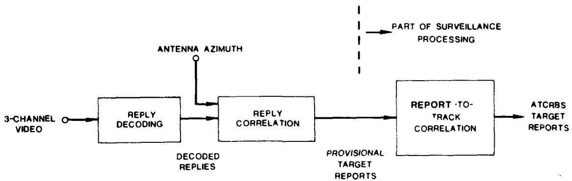
Fig. 3-12. ATRBS Reply Processing.
