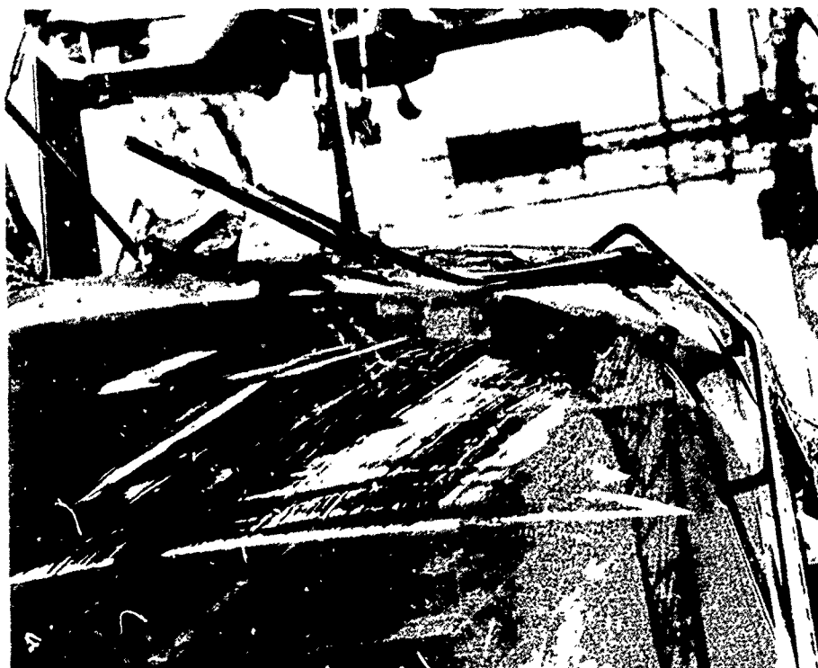
Figure 14. Aircraft condition after test 6.
