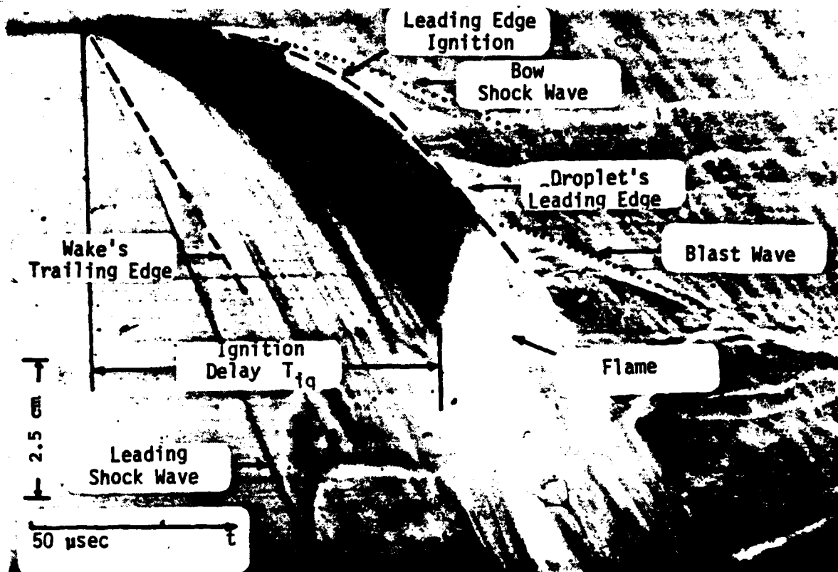
Figure 11(a). Run #501, Decane/Cabosil Droplet, 3000 μm, M = 3.5 .
