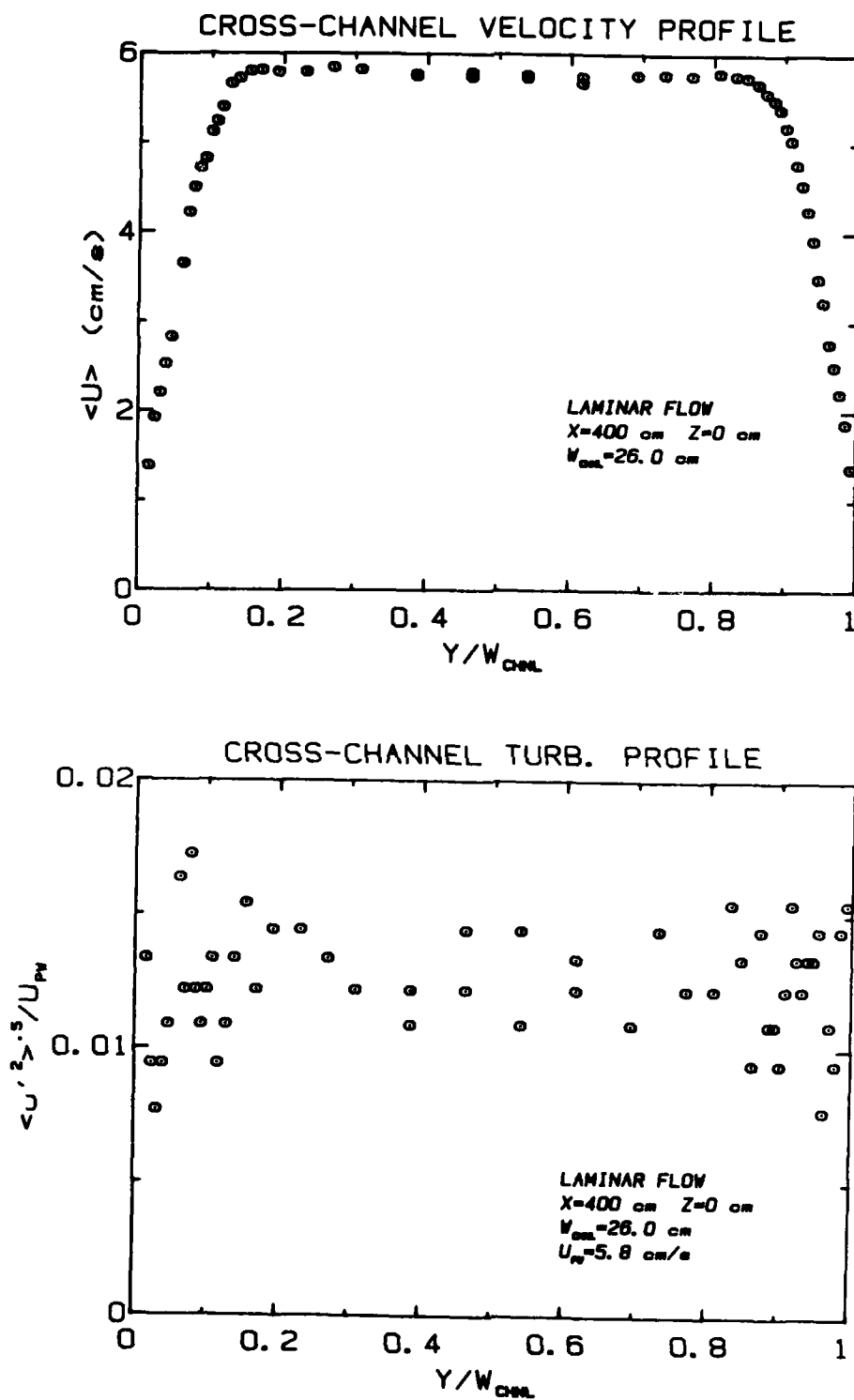
Figure 12: Laminar profiles.
