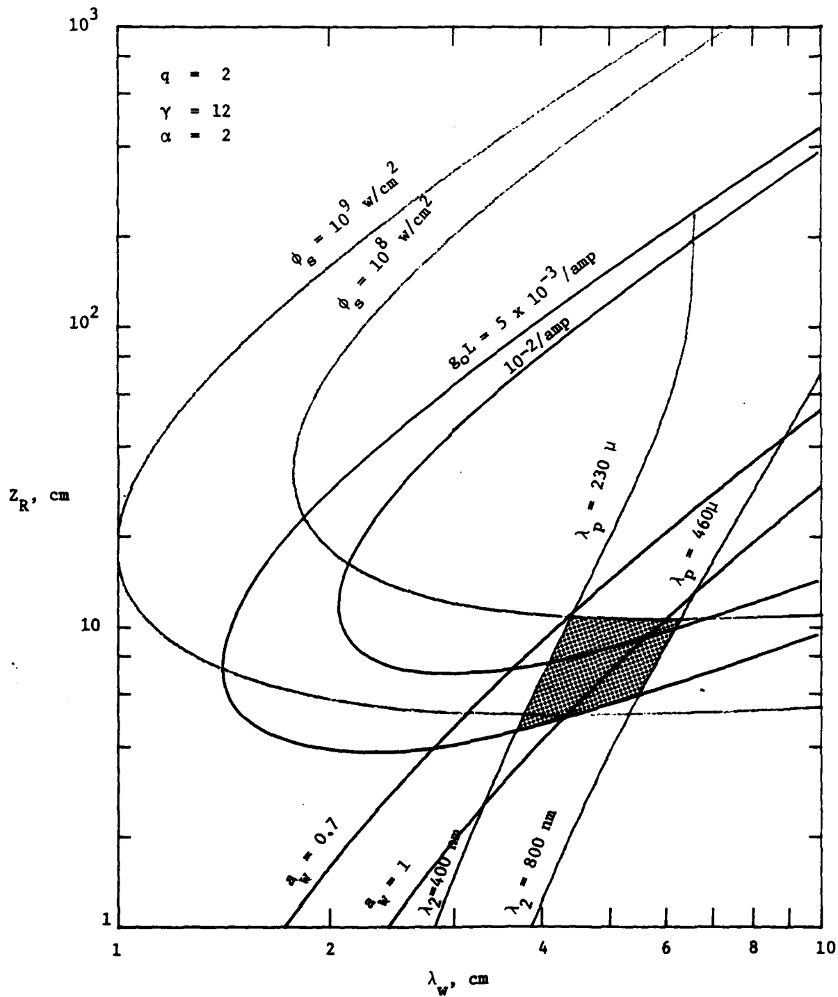
Figure 6. Two-Stage FEL Design Map for \gamma = 12 and L_w = 4Z_R
