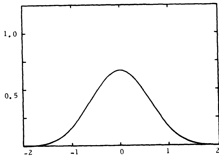
(b) B-spline of degree 3 (cubic B-spline)
