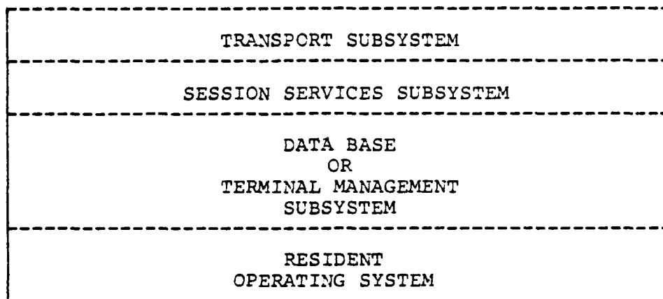
Figure 1.4 Functional LAN Resource Layered Architecture.
