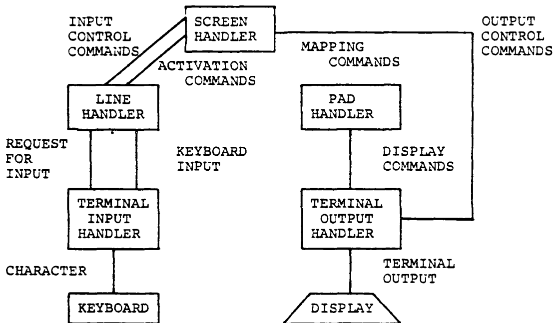
Figure 3.2 Virtual Terminal Controller.
