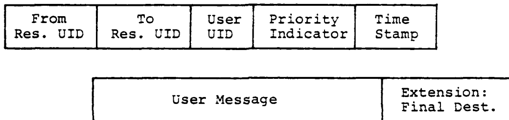
Figure 2.4 Decentralized Message Format.
