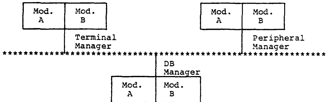
b. Tandem Parallel Processor Architecture.
