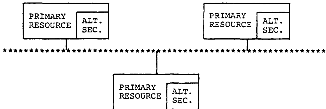
a. Primary and Alternate Secondary LAN Resource.
