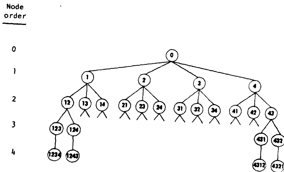
Fig. 5--Branch-and-bound tree for four damaged arcs
