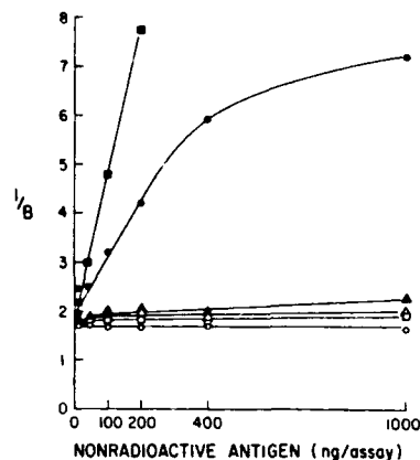
FIG. 5. Antitoxin binding by toxin treated with Formalin plus lysine. B represents the fraction of radiolabeled antigen immunoprecipitated. Toxin was treated with Formalin plus lysine for 24 h (○), 48 h (△), 72 h (□), 120 h (▲), or 240 h (●), or toxin was incubated alone for 240 h (■).
