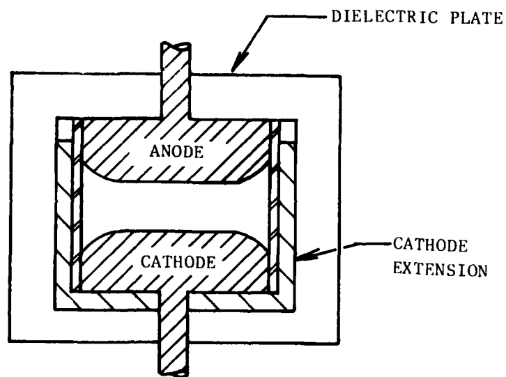
(a) HIGH VOLTAGE GRADIENT
