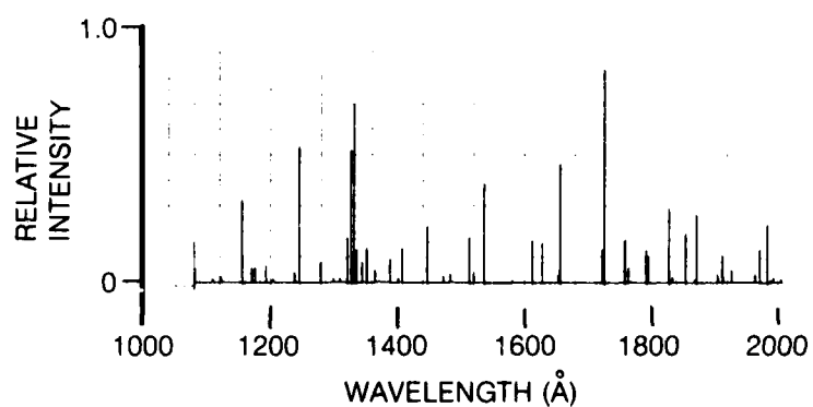
(b) 50% CO 2 , 50% He (TEST NO. 2.10)
