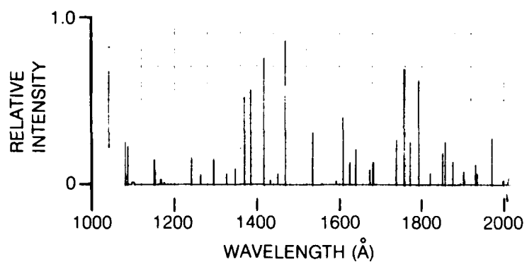
(a) CO 2 (TEST NO. 2.08)
