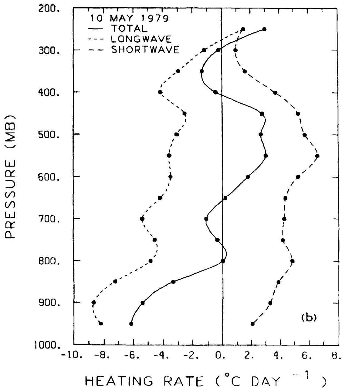
Figure 13 (b). Vertical distribution of the total heating (cooling) rates of the short and longwave radiations on 10 May 1979
