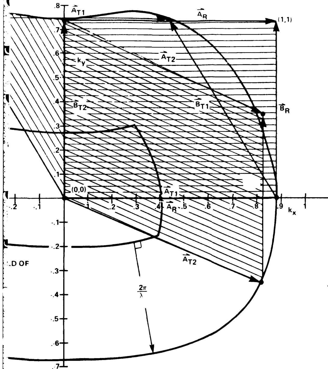
SPACE CONSTRUCTION FOR 10^\circ BORESIGHT ELEVATION
