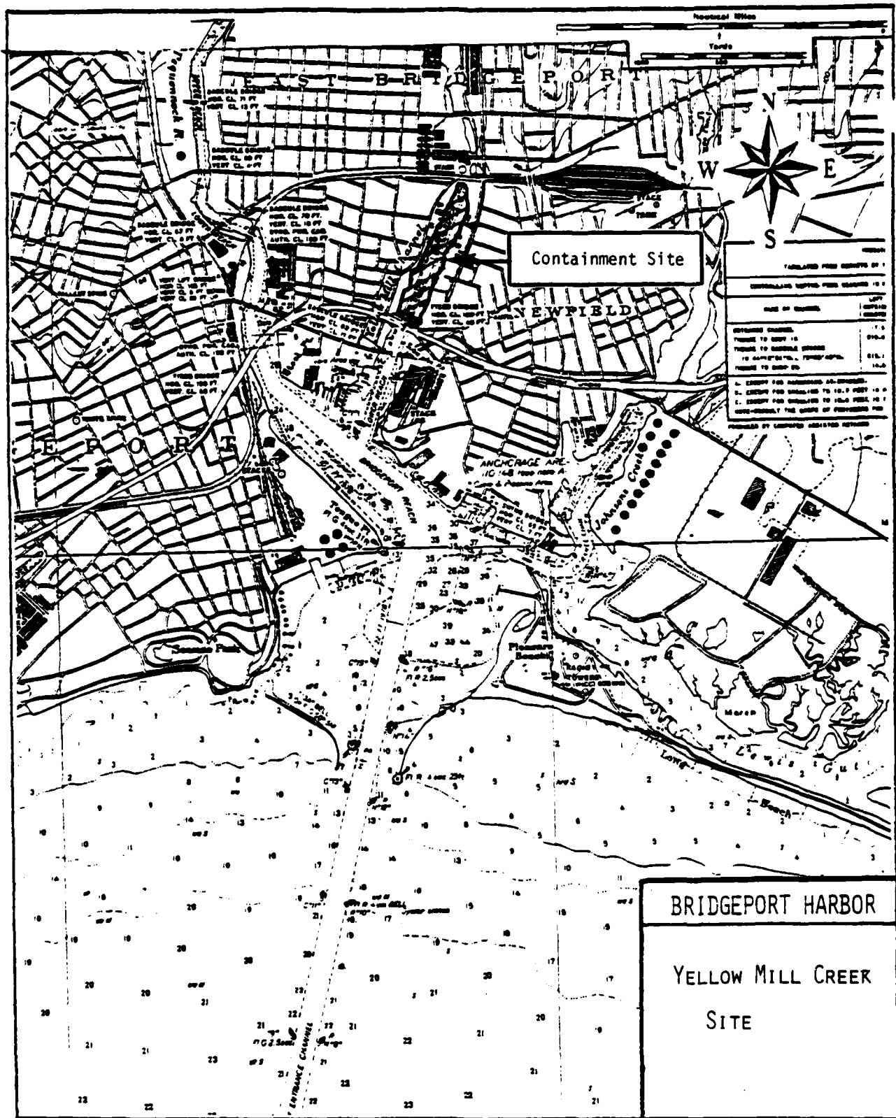
Figure 6-2. Proposed location of prototype dredged material containment facility.
