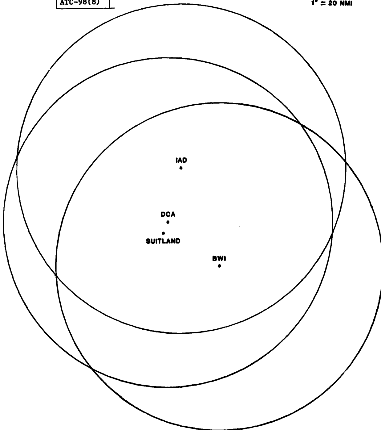
Fig. 8. Sensor locations and nominal coverage.
