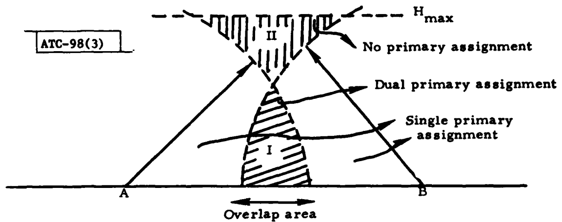
Fig. 3. Primary assignment in vertical plane.
