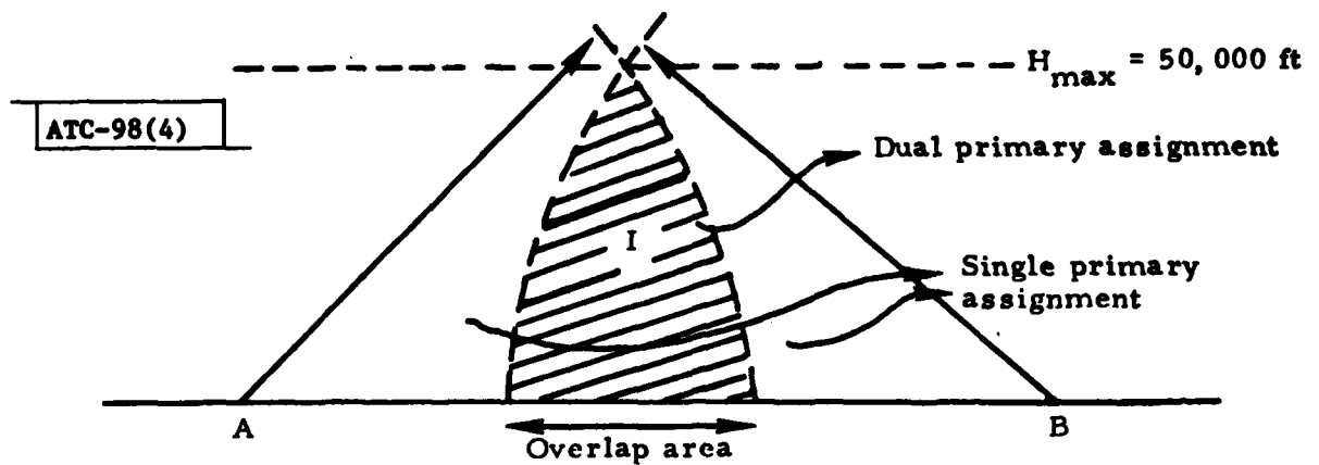
Fig. 4. Enlarged overlap area.
