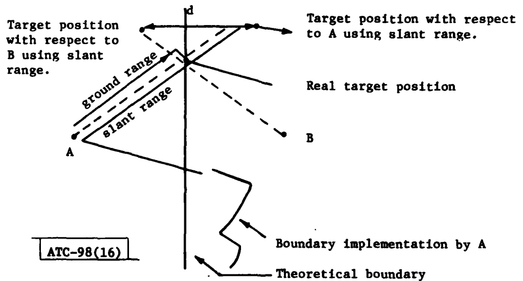
Fig. 16. Slant range overlap.
