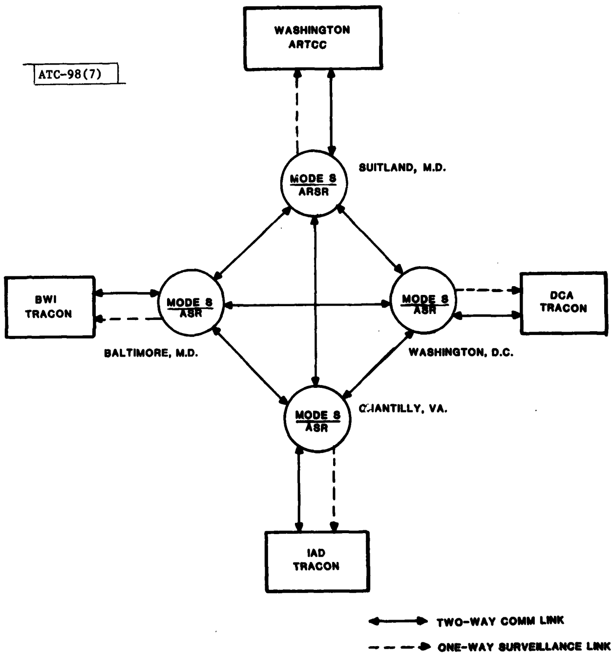
FIG. 7. MODE S SENSOR/ATC CONFIGURATION
