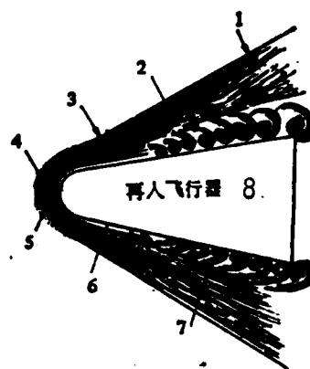
Figure 1. Schematic diagram of the structure of the reentry plasma sheath. 1--slanted shock wave; 2--non-viscous shock wave layer; 3--shock wave front; 4--ionization front zone; 5--stationary point zone with dense plasma; 6--cold inner boundary layer; 7--turbulent boundary layer; 8--reentry flight vehicle
