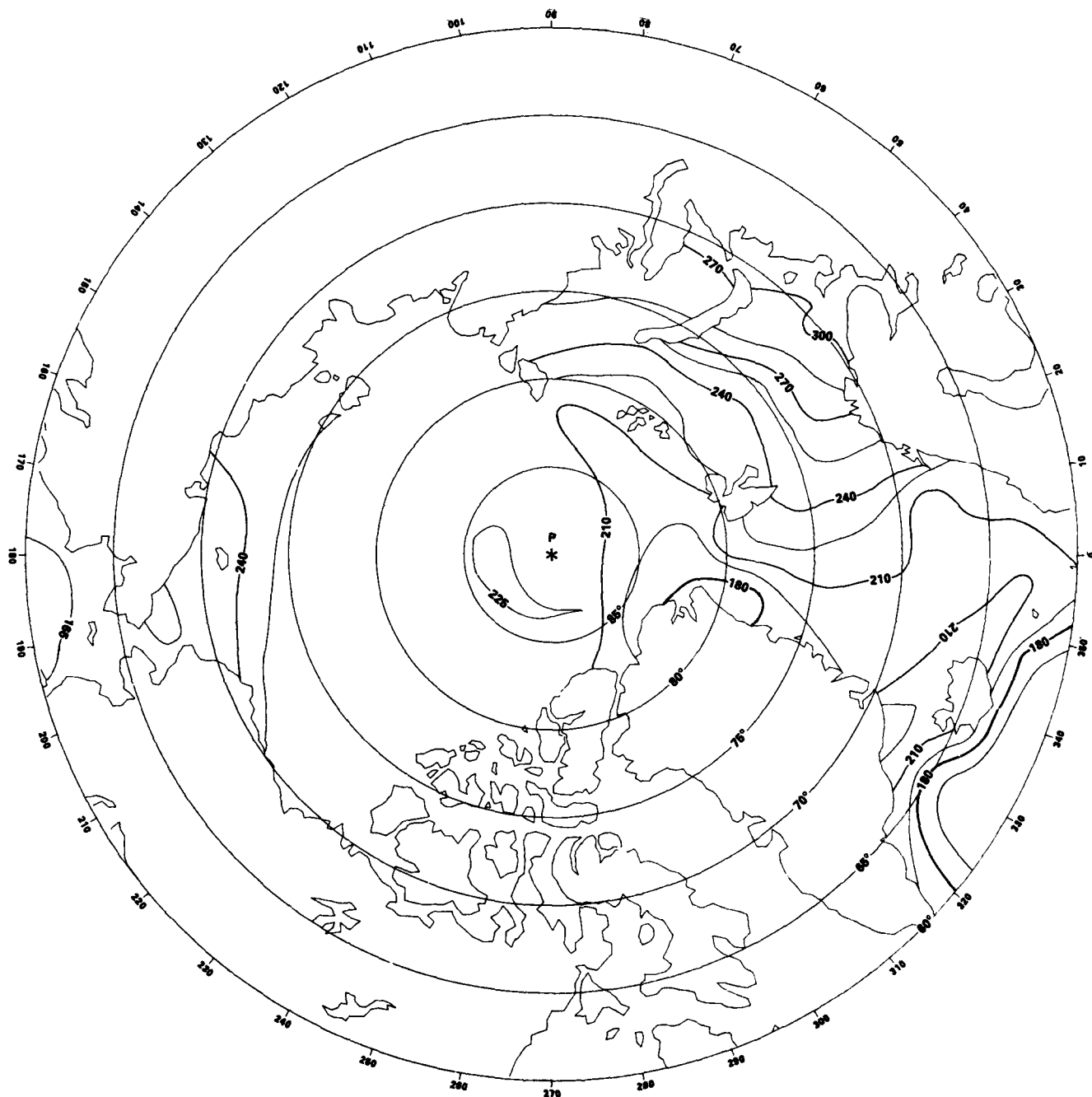
ARCTIC COTIDAL MAP OF M1 OCEAN TIDE GREENWICH PHASES \phi IN DEGREES 30° \approx 27.32 HOURS *P NORTH POLE
