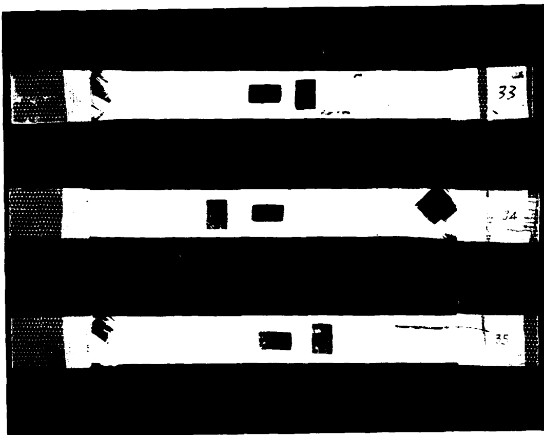
Figure 45. The [\pm 45]_s XP-250 Glass-Epoxy Tension Coupons After Failure
