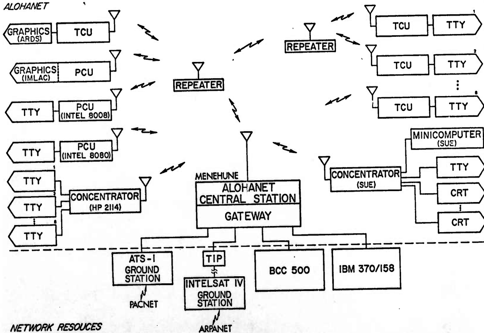
FIGURE 1 THE ALOHANET
