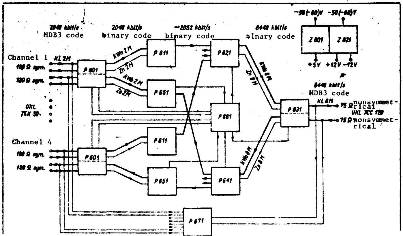
Fig. 4. Block diagram of the KWZ-TCC 120 multichannel terminal.
