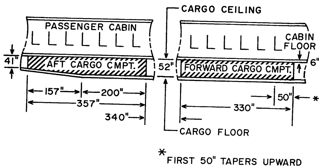
Figure 10. DC-8-43/55
