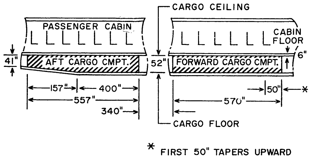
Figure 11. DC-8-61/63
