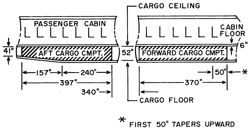
Figure 12. DC-8-62
