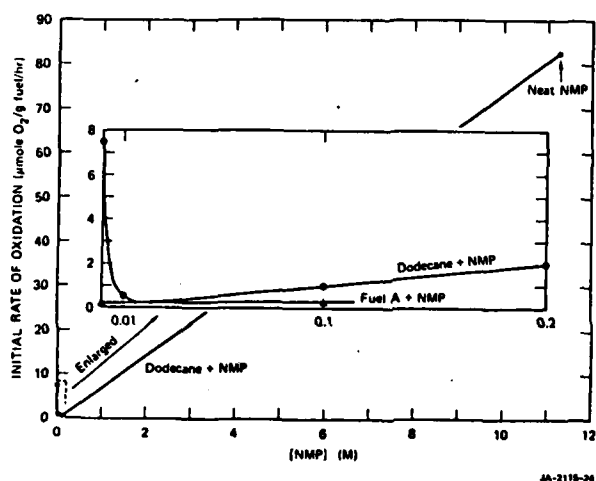
FIGURE 5. INITIAL RATES OF OXIDATION OF FUEL A AND n -DODECANE WITH NMP AT 130°C
