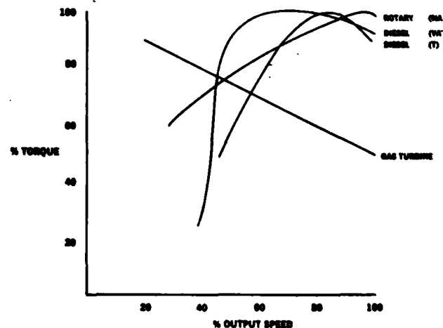
Fig. 15 - Engine Torque Characteristics
