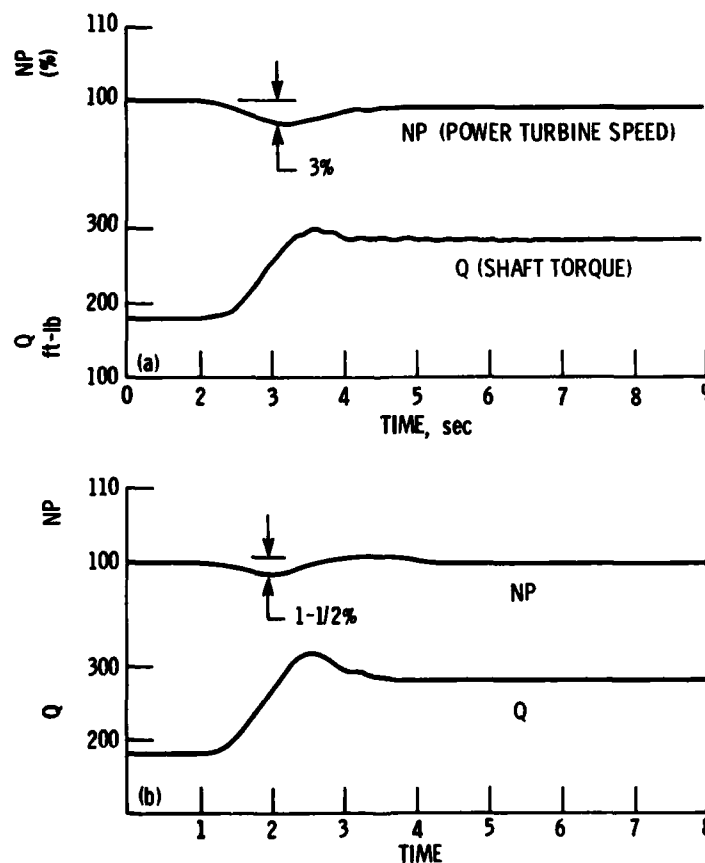
(a) Typical steep turn or approach transient for baseline system. (b) Typical steep turn or approach transient for multi-input system.
