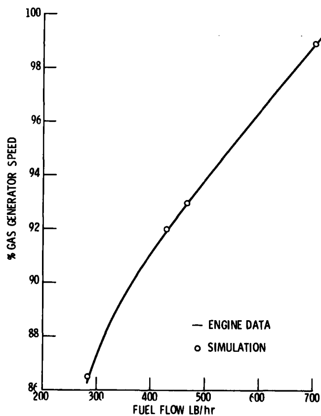
Figure 13. - Comparison of real-time hybrid simulation with engine data.
