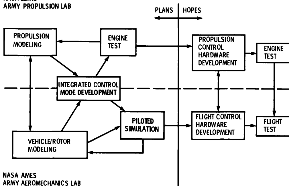
Figure 1. - Rotorcraft integrated flight/propulsion control.
