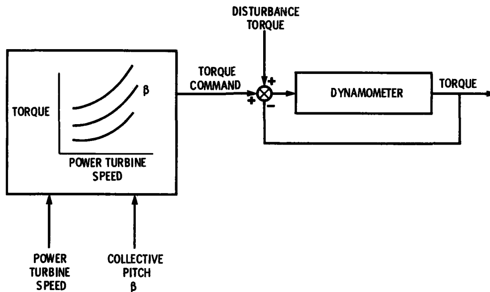
Figure 4. - Dynamometer control system.
