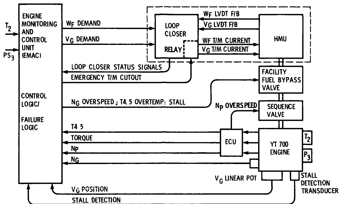
Figure 8 - YT700 research digital control system.
