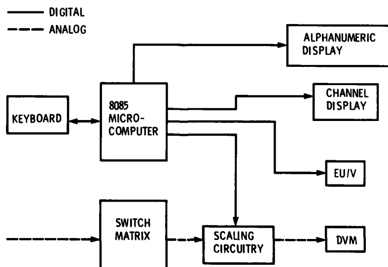
Figure 9 - EMAC monitoring unit.
