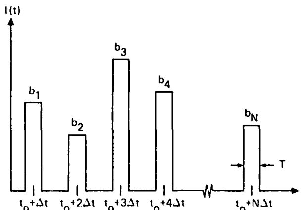
Fig. 2. Typical temporal light signal I(t) containing input column vector (B) information, used to illuminate the optical transparency.
