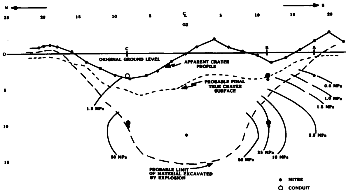
Figure 8. Crater Profile
