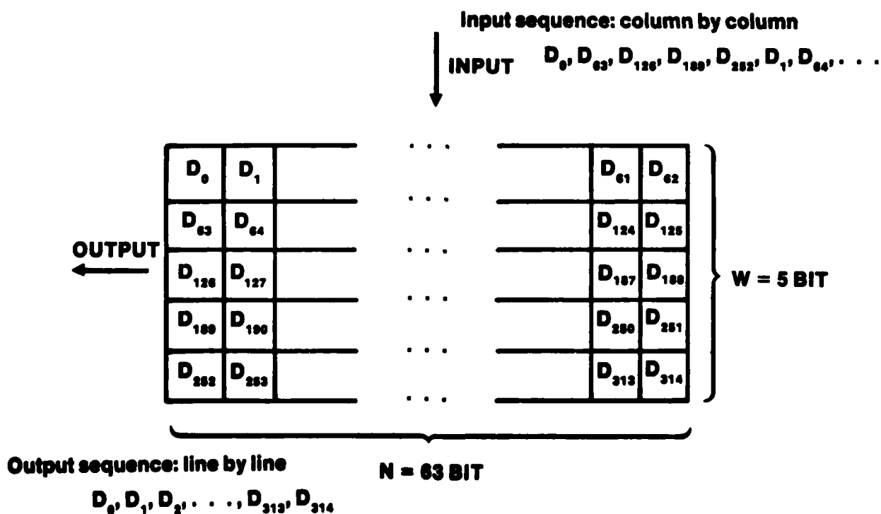
Figure A7b. Deinterleaving of data.
