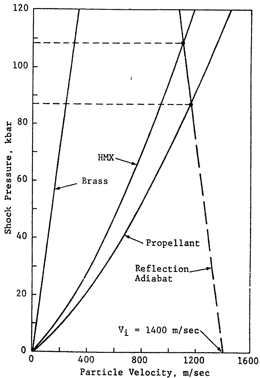
Figure 9. Shock Hugoniots and Impact Properties of HMX and Composite Propellant with a Brass Projectile.
