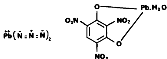
LEAD STYPHNATE
