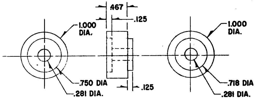
INTERMEDIATE SPACER
