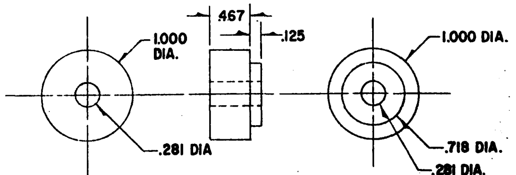
INTERMEDIATE SPACER
