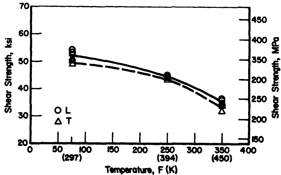
Figure 4. Effect of temperature on pin shear properties of CT 91-T7E69 aluminum.
