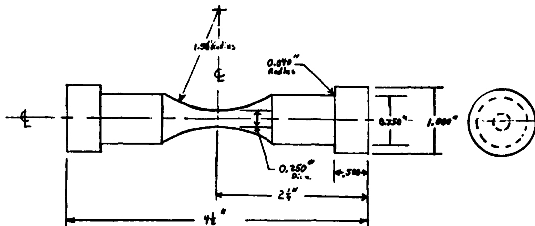
Unnotched fatigue
