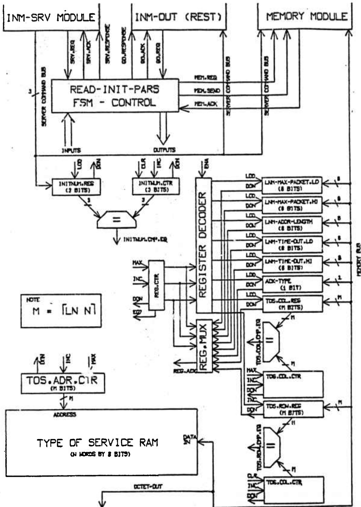
Figure 5-3: Block Diagram of Read_Init_Parameters
