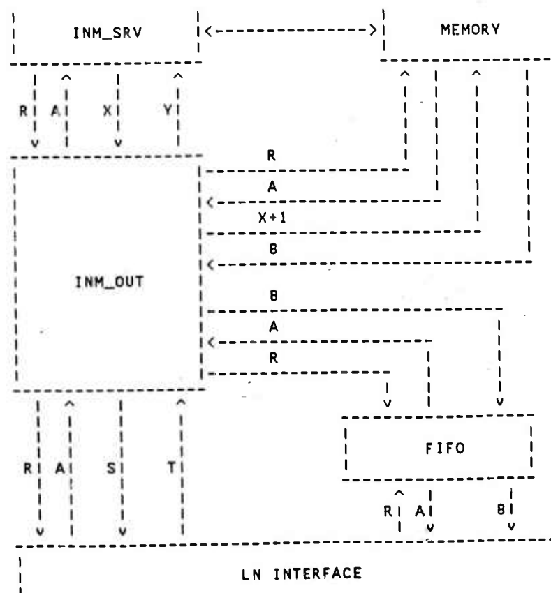
Block Diagram of Anticipated Hardware Realization
