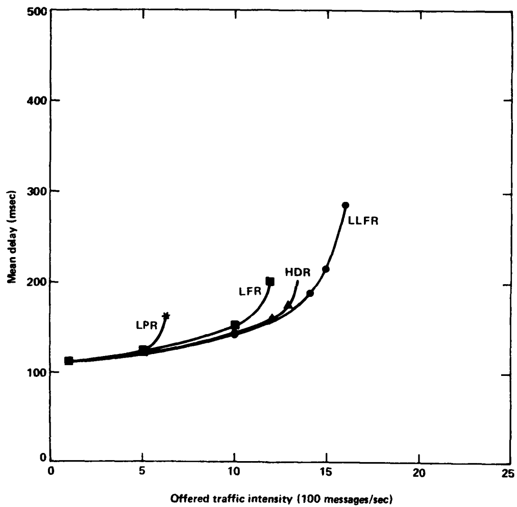
Figure 2.3. Comparative performance of adaptive routing procedures (simulation).
