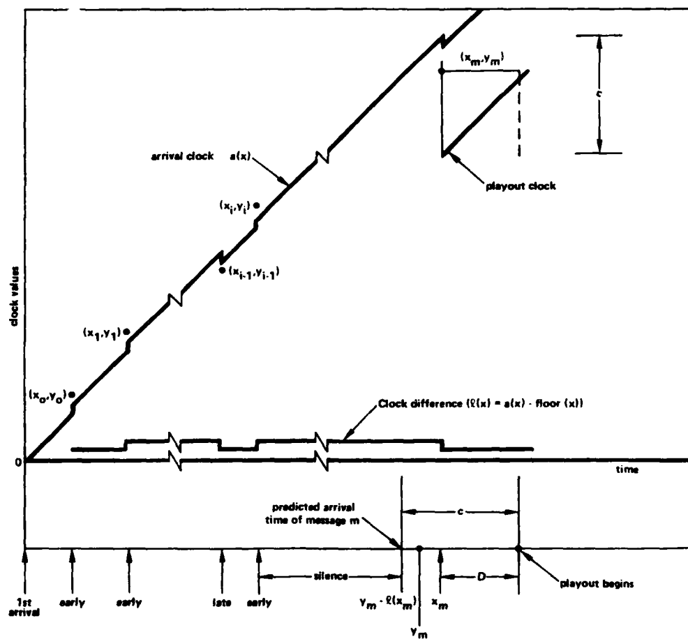
Figure 5.10. Delay tracker.
