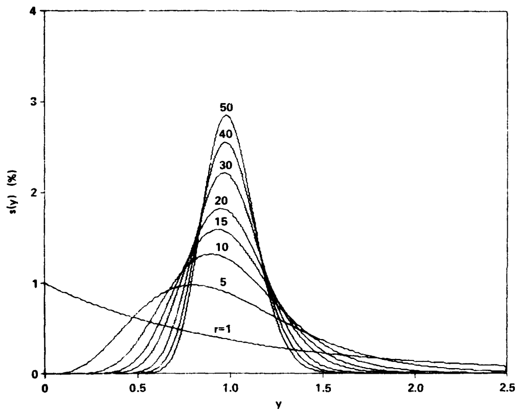
Figure 5.26. Erlang family of density functions.
