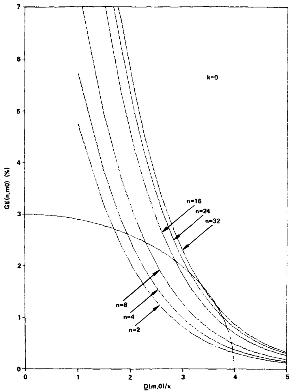
Figure 5.21. Gap probability (Method E) vs. mean range.
