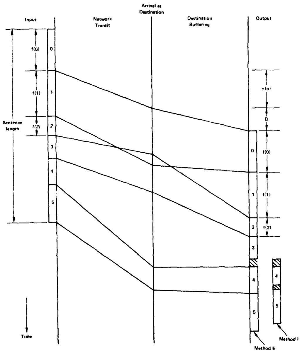
Figure 5.3. End-to-end communication.
