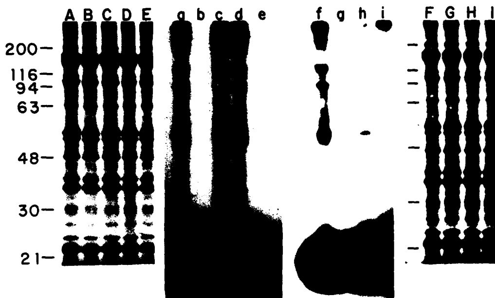
Figure 1: SDS-polyacrylamide gel (A-E) and corresponding autoradiograph (a-i) of coated vesicles exposed to azido- ^{125}\text{I} -CAM. Standard conditions are described in Methods; additions are indicated here. Samples A-E (a-e) contained 250 nM reagent; samples F-I (f-i) contained 125 nM reagent. A (a) 2 mM \text{CaCl}_2 ; B (b) 2 mM \text{MgCl}_2 ; C (c) 2 mM \text{MnCl}_2 ; D (d) same as A; E (e) same as A except that sample was not photolyzed; F (f) same as A except using the lower concentration of reagent; G (g) \text{CaCl}_2 omitted; H (h) 2 mM \text{CaCl}_2 and 25 \mu\text{M} native CAM; I (i) 2 mM \text{CaCl}_2 and 200 \mu\text{M} Stelazine. The overexposed area at the bottom of the autoradiographs corresponds to azido- ^{125}\text{I} -CAM.
