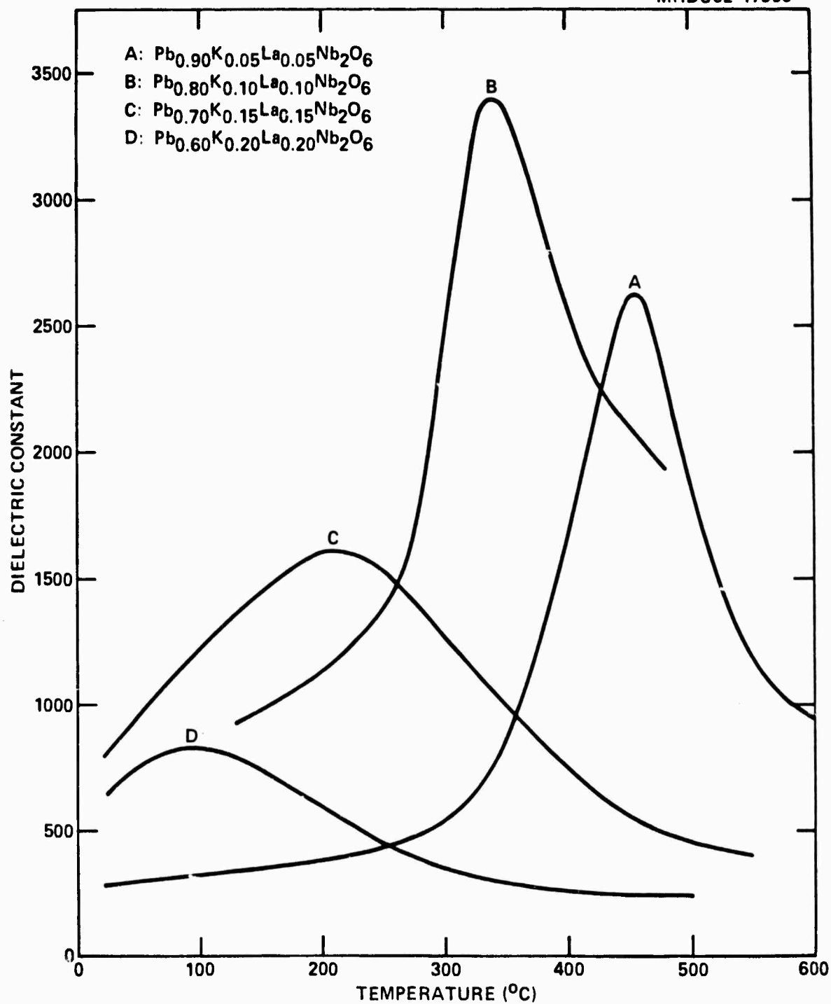
Fig. 30 Dielectric constant vs temperature of \text{Pb}_{1-2x}\text{K}_x\text{La}_x\text{Nb}_2\text{O}_6 .
